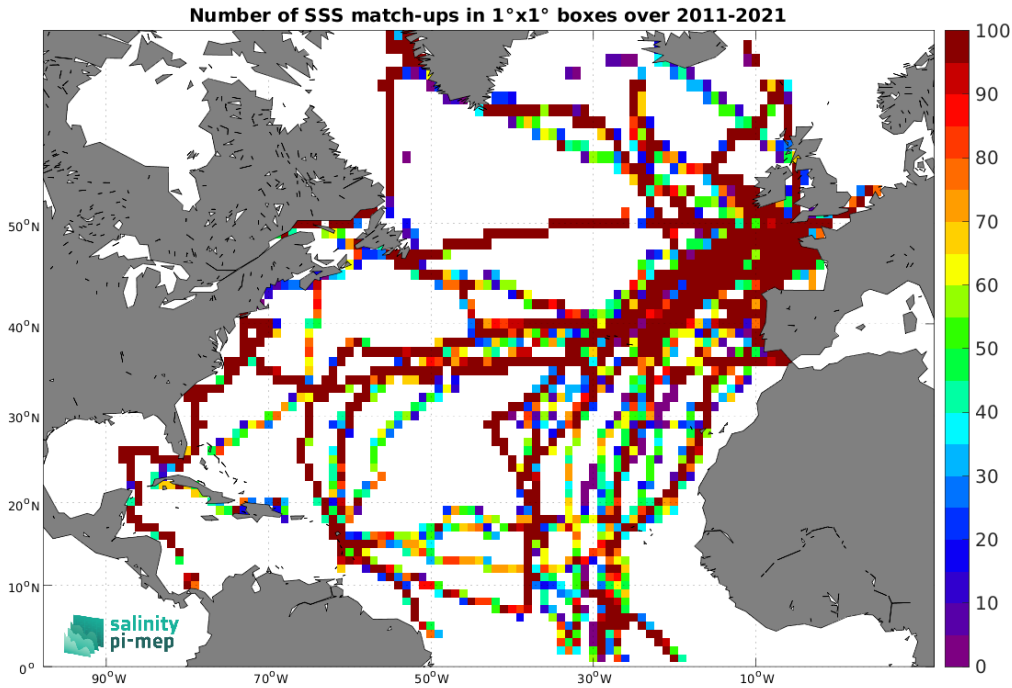
Figure 5: Number of SSS match-ups between TSG (GOSUD-Sailing-ship) SSS and the SMOS SSS L4 v1 - Daily (CMEMS-CNR) SSS product for the North Atlantic Ocean Pi-MEP region over 1^\circ \times 1^\circ boxes and for the full satellite product period.
