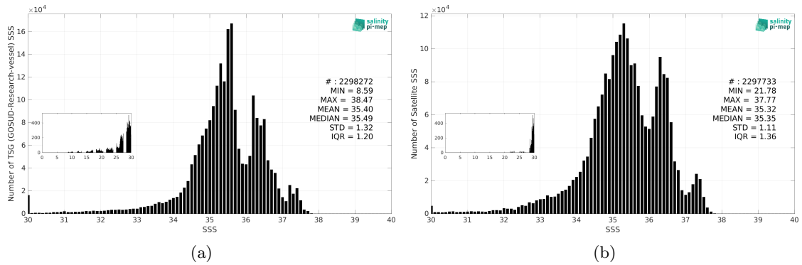
Figure 3: Histograms of SSS from TSG (GOSUD-Research-vessel) (a) and SMOS SSS L4 v1 - Daily (CMEMS-CNR) (b) considering all match-up pairs per bins of 0.1 over the North Atlantic Ocean Pi-MEP region and for the full satellite product period.
