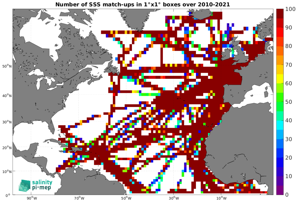
Figure 5: Number of SSS match-ups between TSG (GOSUD-Research-vessel) SSS and the SMOS SSS L4 v1 - Daily (CMEMS-CNR) SSS product for the North Atlantic Ocean Pi-MEP region over 1^\circ \times 1^\circ boxes and for the full satellite product period.
