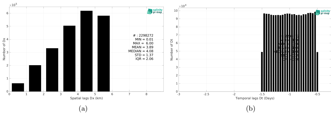
Figure 6: Histograms of the spatial (a) and temporal (b) lags between the location/time of the TSG (GOSUD-Research-vessel) measurement and the date of the corresponding SMOS SSS L4 v1 - Daily (CMEMS-CNR) SSS pixel.
