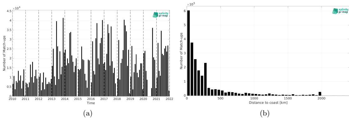
Figure 2: Number of match-ups between TSG (GOSUD-Research-vessel) and SMOS SSS L4 v1 - Daily (CMEMS-CNR) SSS as a function of time (a) and as function of the distance to coast (b) over the North Atlantic Ocean Pi-MEP region and for the full satellite product period.
