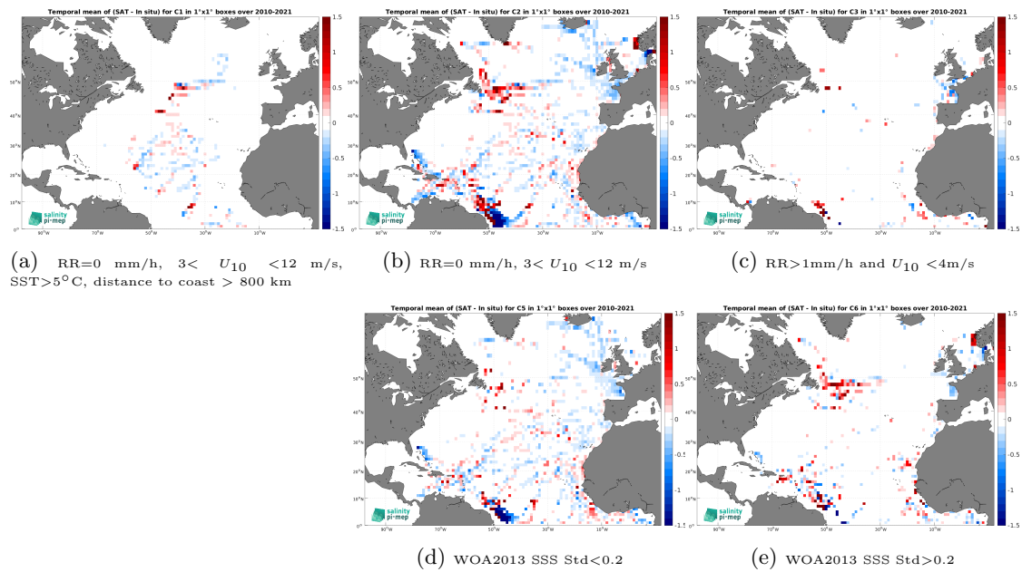
Figure 14: Temporal mean gridded over spatial boxes of size 1^\circ \times 1^\circ of \Delta\text{SSS} (SMOS SSS L4 v1 - Daily (CMEMS-CNR) - TSG (GOSUD-Research-vessel)) for 5 different subdatasets corresponding to:RR=0 mm/h, 3 < U_{10} < 12 m/s, SST>5°C, distance to coast > 800 km (a), RR=0 mm/h, 3 < U_{10} < 12 m/s (b), RR>1mm/h and U_{10} < 4 m/s (c), WOA2013 SSS Std<0.2 (d), WOA2013 SSS Std>0.2 (e).
