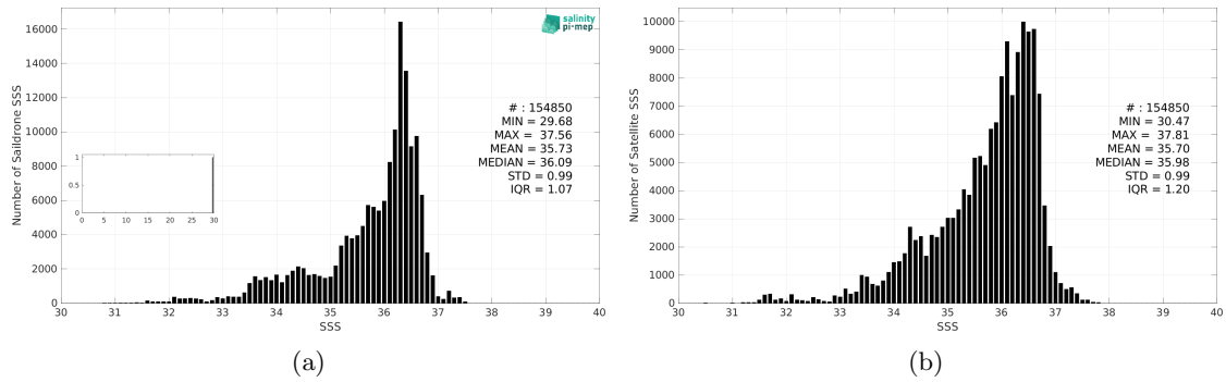
Figure 3: Histograms of SSS from Sailability (a) and SMOS SSS L4 v1 - Daily (CMEMS-CNR) (b) considering all match-up pairs per bins of 0.1 over the North Atlantic Ocean Pi-MEP region and for the full satellite product period.
