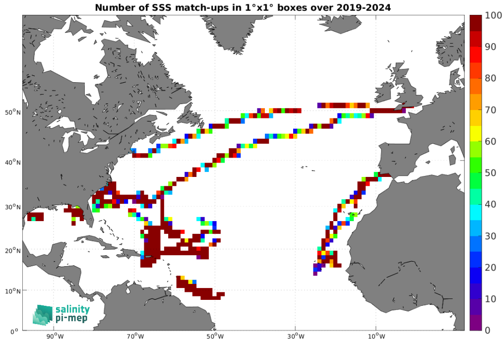
Figure 5: Number of SSS match-ups between Saildrone SSS and the SMOS SSS L4 v1 - Daily (CMEMS-CNR) SSS product for the North Atlantic Ocean Pi-MEP region over 1^\circ \times 1^\circ boxes and for the full satellite product period.
