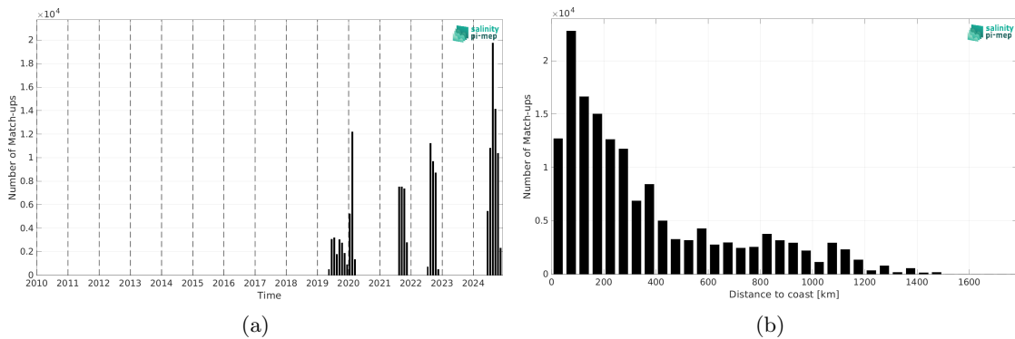
Figure 2: Number of match-ups between Saildrone and SMOS SSS L4 v1 - Daily (CMEMS-CNR) SSS as a function of time (a) and as function of the distance to coast (b) over the North Atlantic Ocean Pi-MEP region and for the full satellite product period.
