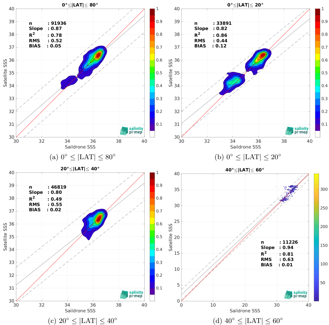
Figure 10: Contour maps of the concentration of SMOS SSS L4 v1 - Daily (CMEMS-CNR) SSS (y-axis) versus Saildrone SSS (x-axis) at match-up pairs for different latitude bands. For each plot, the red line shows x=y . The black thin and dashed lines indicate a linear fit through the data cloud and the \pm 95\% confidence levels, respectively. The number match-up pairs n , the slope and R^2 coefficient of the linear fit, the root mean square (RMS) and the mean bias between satellite and in situ data are indicated for each latitude band in each plots.
