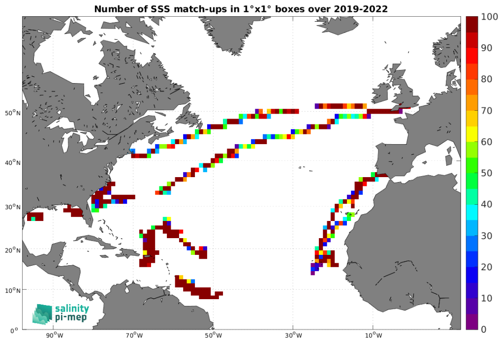
Figure 5: Number of SSS match-ups between Saildrone SSS and the SMOS SSS L4 v1 - Daily (CMEMS-CNR) SSS product for the North Atlantic Ocean Pi-MEP region over 1^{\circ} \times 1^{\circ} boxes and for the full satellite product period.
