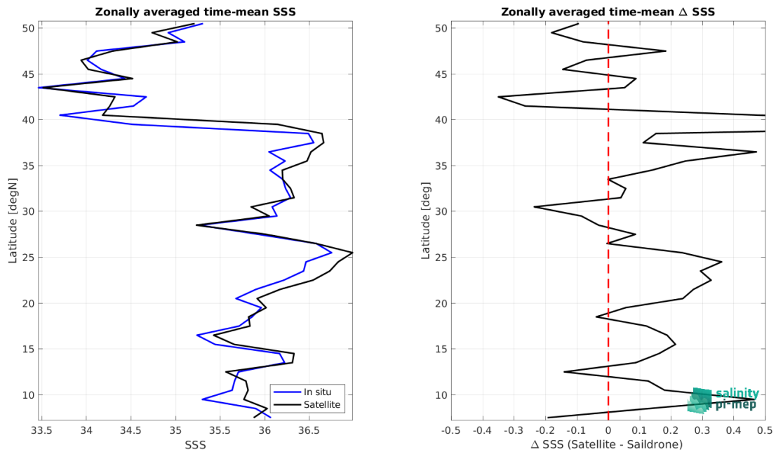
Figure 9: Left panel: Zonal mean SSS from SMOS SSS L4 v1 - Daily (CMEMS-CNR) satellite product (black) and from Saildrone (blue). Right panel: Zonal mean of \Delta SSS (Satellite - Saildrone) for all the collected Pi-MEP match-up pairs estimated over the full satellite product period.
