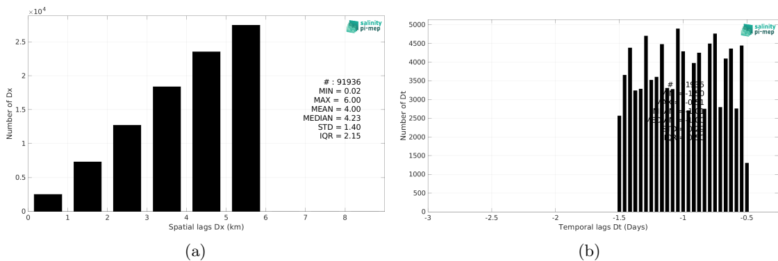
Figure 6: Histograms of the spatial (a) and temporal (b) lags between the location/time of the Saildrone measurement and the date of the corresponding SMOS SSS L4 v1 - Daily (CMEMS-CNR) SSS pixel.
