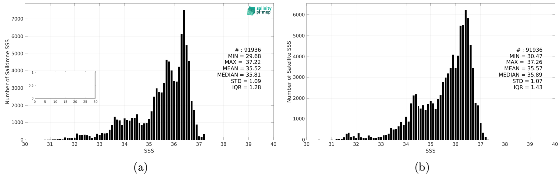
Figure 3: Histograms of SSS from Saildrone (a) and SMOS SSS L4 v1 - Daily (CMEMS-CNR) (b) considering all match-up pairs per bins of 0.1 over the North Atlantic Ocean Pi-MEP region and for the full satellite product period.
