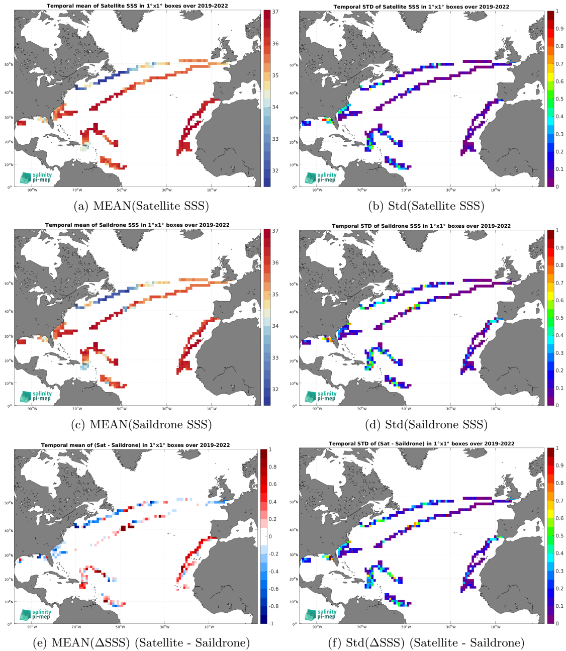
Figure 7: Temporal mean (left) and Std (right) of SSS from SMOS SSS L4 v1 - Daily (CMEMS-CNR) (top), Saildrone (middle), and of \Delta SSS (Satellite - Saildrone). Only match-up pairs are used to generate these maps.
