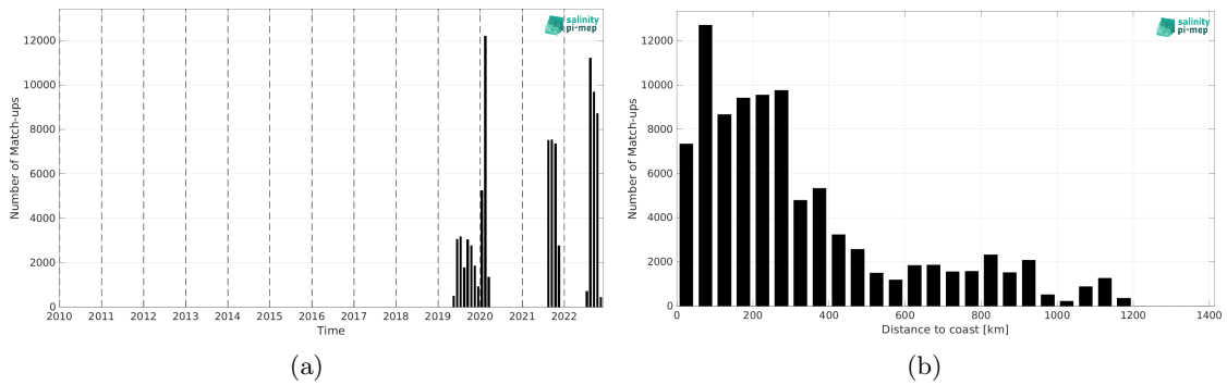
Figure 2: Number of match-ups between Saildrone and SMOS SSS L4 v1 - Daily (CMEMS-CNR) SSS as a function of time (a) and as function of the distance to coast (b) over the North Atlantic Ocean Pi-MEP region and for the full satellite product period.
