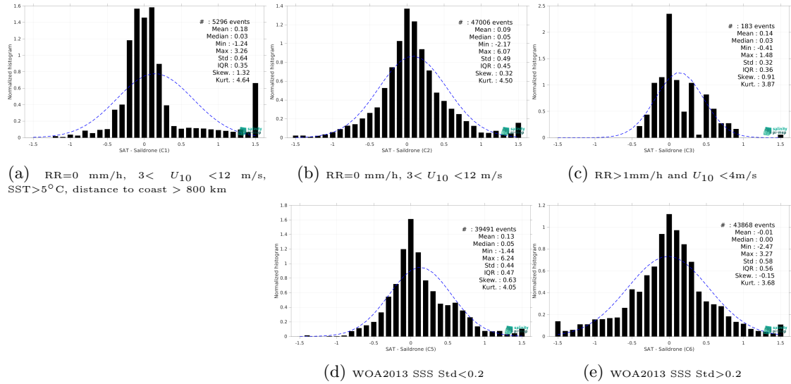
Figure 15: Normalized histogram of \Delta SSS (SMOS SSS L4 v1 - Daily (CMEMS-CNR) - Sairdrone) for 5 different subdatasets corresponding to: RR=0 mm/h, 3 < U_{10} < 12 m/s, SST > 5°C, distance to coast > 800 km (a), RR=0 mm/h, 3 < U_{10} < 12 m/s (b), RR > 1mm/h and U_{10} < 4 m/s (c), WOA2013 SSS Std < 0.2 (d), WOA2013 SSS Std > 0.2 (e).
