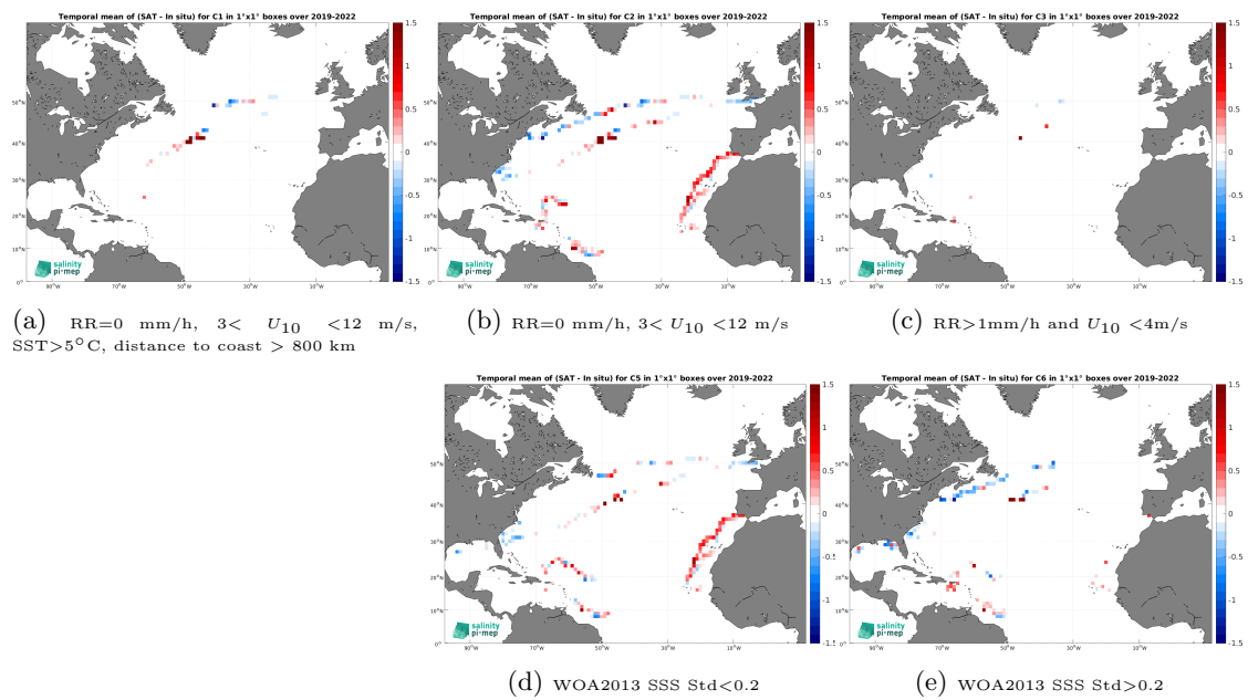
Figure 14: Temporal mean gridded over spatial boxes of size 1^\circ \times 1^\circ of \Delta\text{SSS} (SMOS SSS L4 v1 - Daily (CMEMS-CNR) - Saildrone) for 5 different subdatasets corresponding to:RR=0 mm/h, 3 < U_{10} < 12 m/s, SST>5°C, distance to coast > 800 km (a), RR=0 mm/h, 3 < U_{10} < 12 m/s (b), RR>1mm/h and U_{10} < 4 m/s (c), WOA2013 SSS Std<0.2 (d), WOA2013 SSS Std>0.2 (e).
