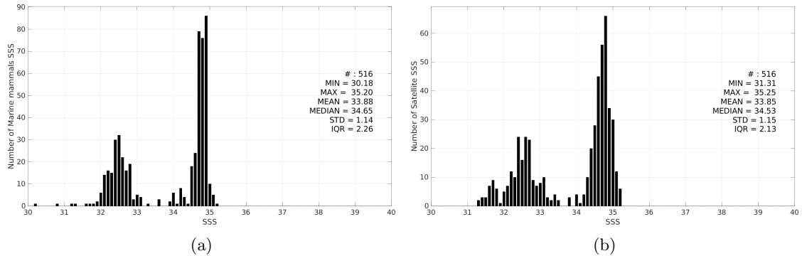
Figure 3: Histograms of SSS from Marine mammals (a) and SMOS SSS L4 v1 - Daily (CMEMS-CNR) (b) considering all match-up pairs per bins of 0.1 over the North Atlantic Ocean Pi-MEP region and for the full satellite product period.
