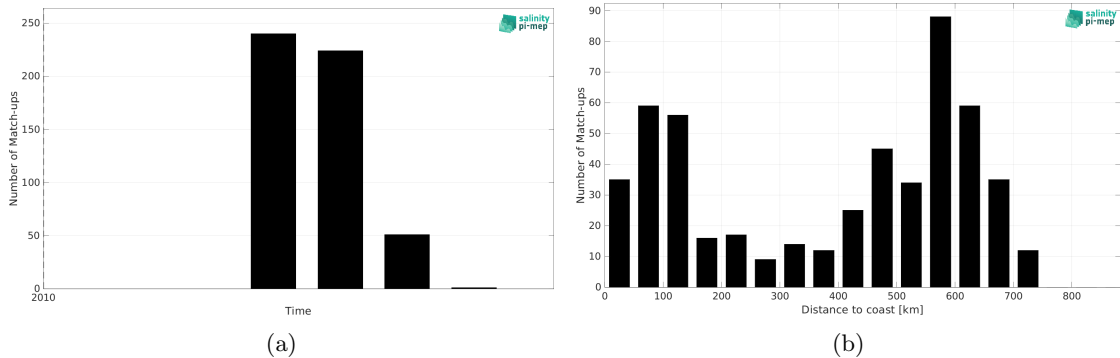
Figure 2: Number of match-ups between Marine mammals and SMOS SSS L4 v1 - Daily (CMEMS-CNR) SSS as a function of time (a) and as function of the distance to coast (b) over the North Atlantic Ocean Pi-MEP region and for the full satellite product period.
