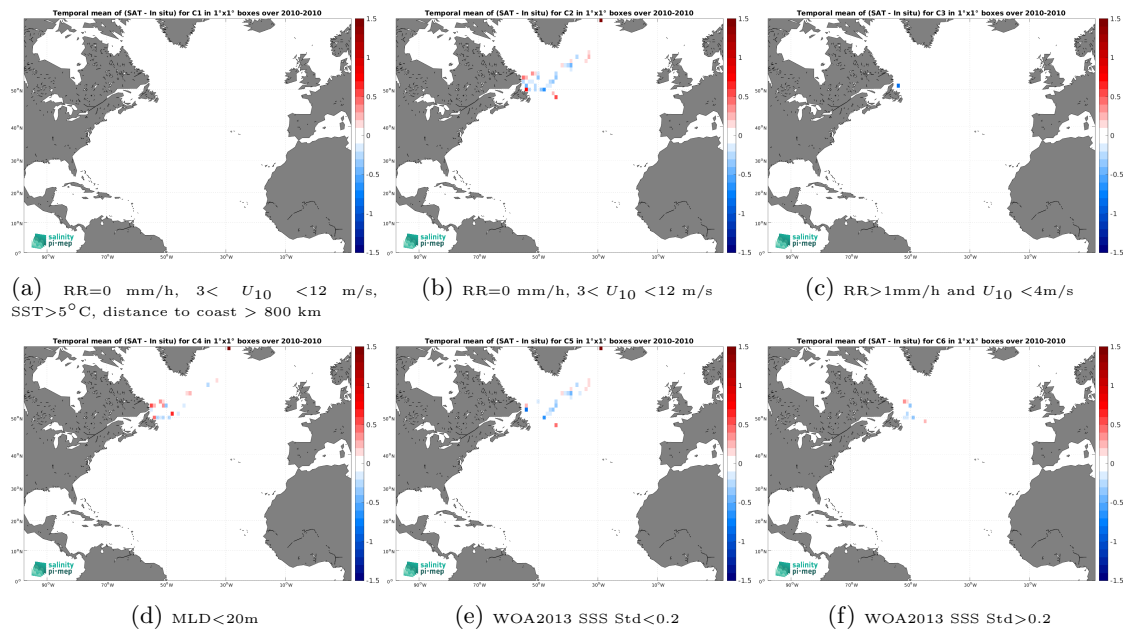
Figure 14: Temporal mean gridded over spatial boxes of size 1^\circ \times 1^\circ of \Delta\text{SSS} (SMOS SSS L4 v1 - Daily (CMEMS-CNR) - Marine mammals) for 6 different subdatasets corresponding to: RR=0 mm/h, 3 < U_{10} < 12 m/s, SST > 5°C, distance to coast > 800 km (a), RR=0 mm/h, 3 < U_{10} < 12 m/s (b), RR > 1mm/h and U_{10} < 4 m/s (c), MLD < 20m (d), WOA2013 SSS Std < 0.2 (e), WOA2013 SSS Std > 0.2 (f).
