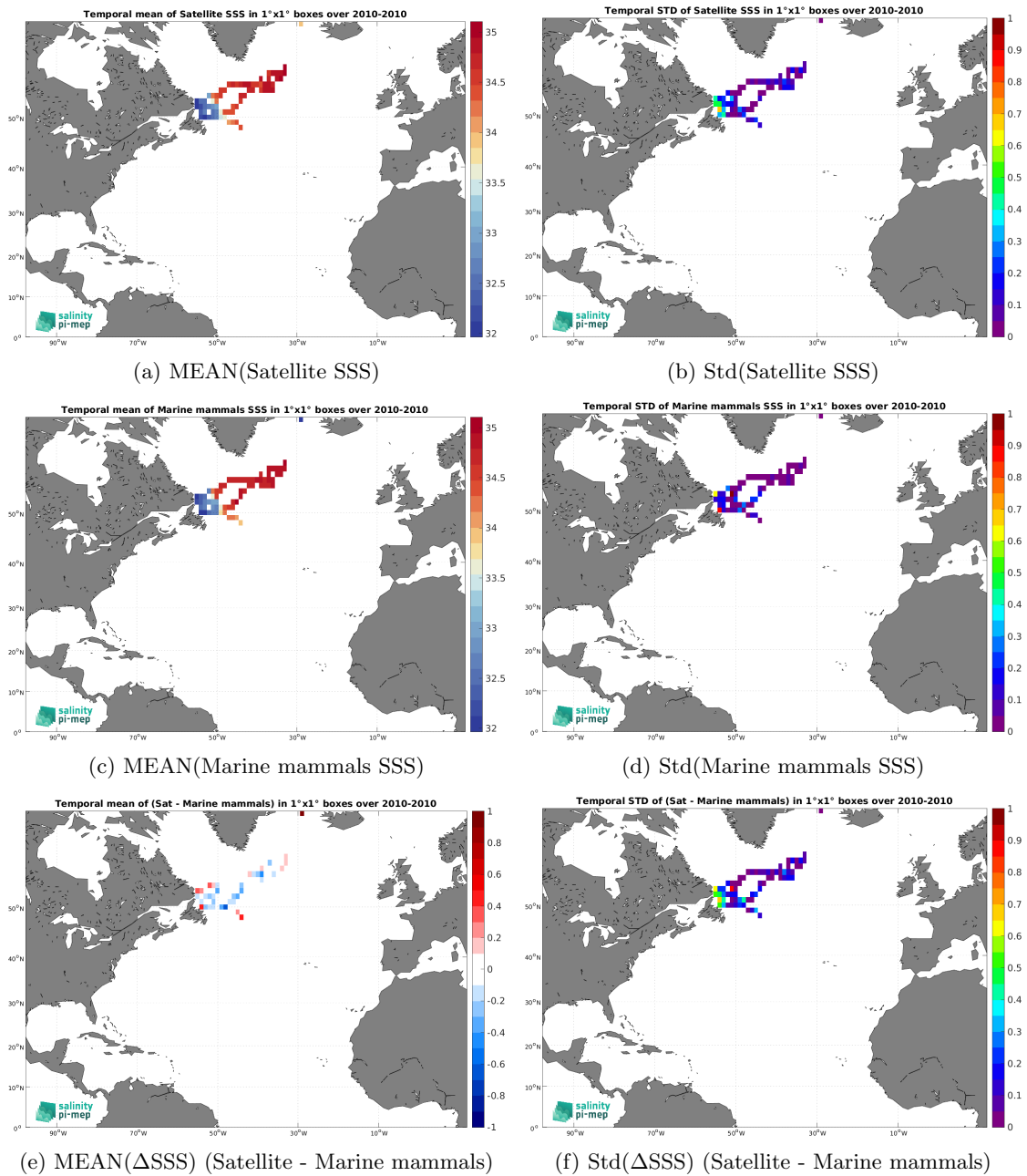
Figure 7: Temporal mean (left) and Std (right) of SSS from SMOS SSS L4 v1 - Daily (CMEMS-CNR) (top), Marine mammals (middle), and of \Delta SSS (Satellite - Marine mammals). Only match-up pairs are used to generate these maps.
