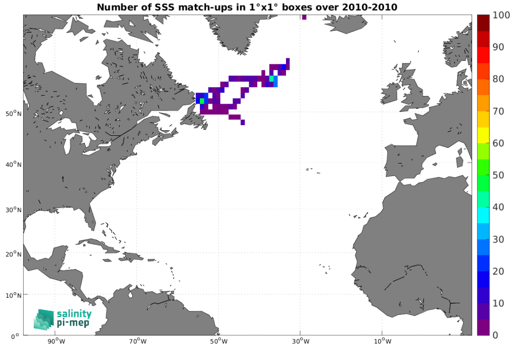
Figure 5: Number of SSS match-ups between Marine mammals SSS and the SMOS SSS L4 v1 - Daily (CMEMS-CNR) SSS product for the North Atlantic Ocean Pi-MEP region over 1^\circ \times 1^\circ boxes and for the full satellite product period.
