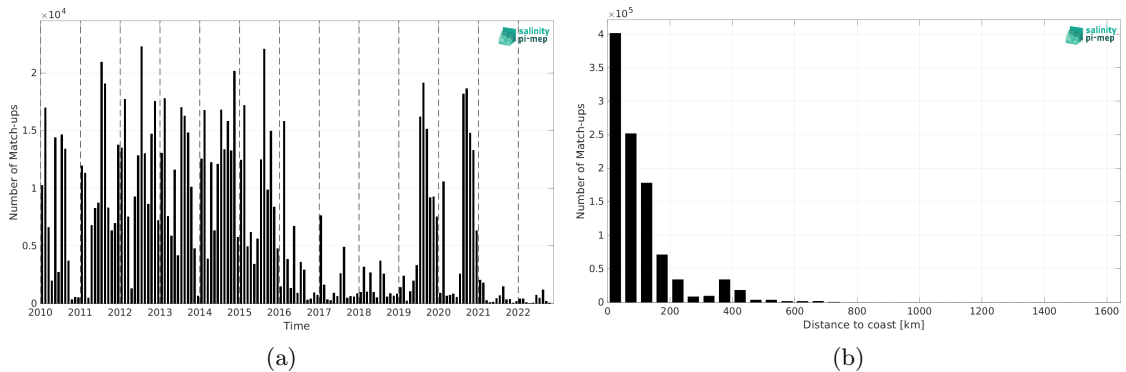
Figure 2: Number of match-ups between ICES and SMOS SSS L4 v1 - Daily (CMEMS-CNR) SSS as a function of time (a) and as function of the distance to coast (b) over the North Atlantic Ocean Pi-MEP region and for the full satellite product period.
