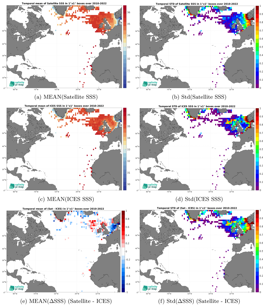
Figure 7: Temporal mean (left) and Std (right) of SSS from SMOS SSS L4 v1 - Daily (CMEMS-CNR) (top), ICES (middle), and of \Delta SSS (Satellite - ICES). Only match-up pairs are used to generate these maps.
