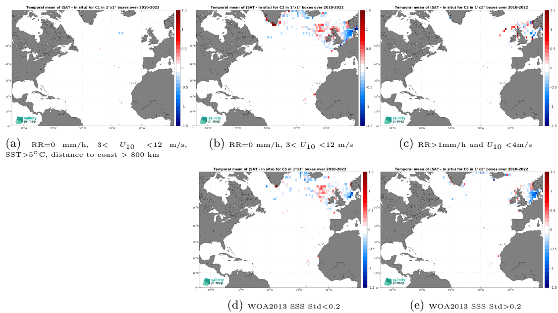
Figure 14: Temporal mean gridded over spatial boxes of size 1^\circ \times 1^\circ of \Delta SSS (SMOS SSS L4 v1 - Daily (CMEMS-CNR) - ICES) for 5 different subdatasets corresponding to:RR=0 mm/h, 3 < U_{10} < 12 m/s, SST >5^\circ\text{C} , distance to coast > 800 km (a), RR=0 mm/h, 3 < U_{10} < 12 m/s (b), RR >1 mm/h and U_{10} < 4 m/s (c), WOA2013 SSS Std <0.2 (d), WOA2013 SSS Std >0.2 (e).
