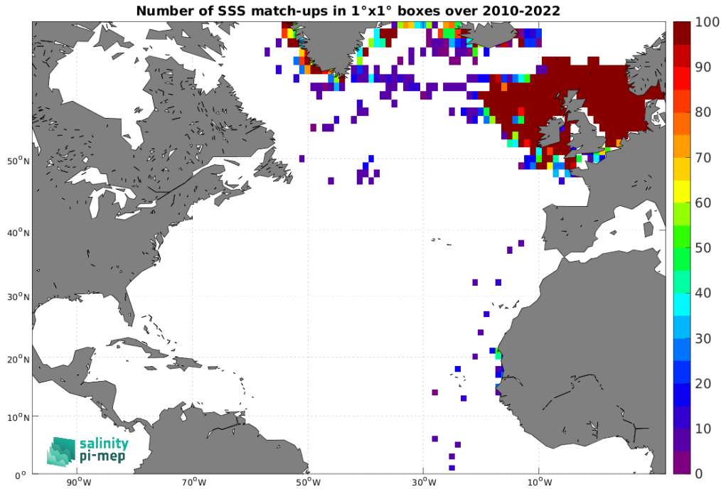
Figure 5: Number of SSS match-ups between ICES SSS and the SMOS SSS L4 v1 - Daily (CMEMS-CNR) SSS product for the North Atlantic Ocean Pi-MEP region over 1^\circ \times 1^\circ boxes and for the full satellite product period.
