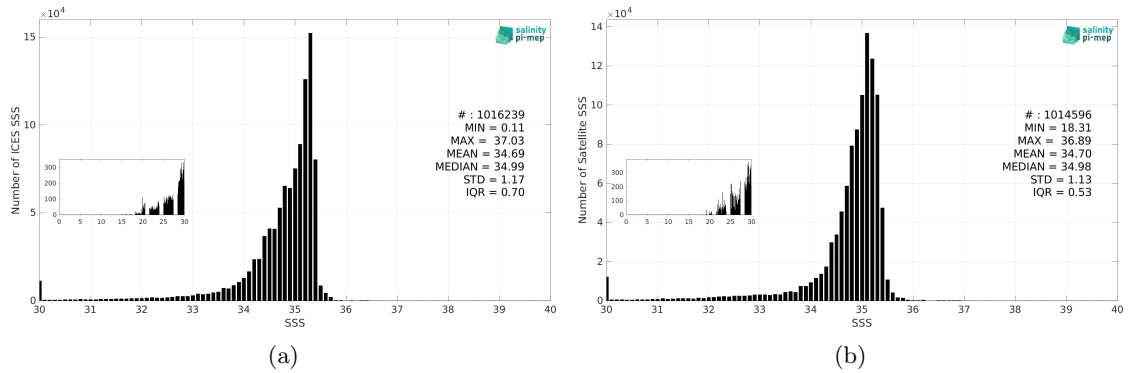
Figure 3: Histograms of SSS from ICES (a) and SMOS SSS L4 v1 - Daily (CMEMS-CNR) (b) considering all match-up pairs per bins of 0.1 over the North Atlantic Ocean Pi-MEP region and for the full satellite product period.
