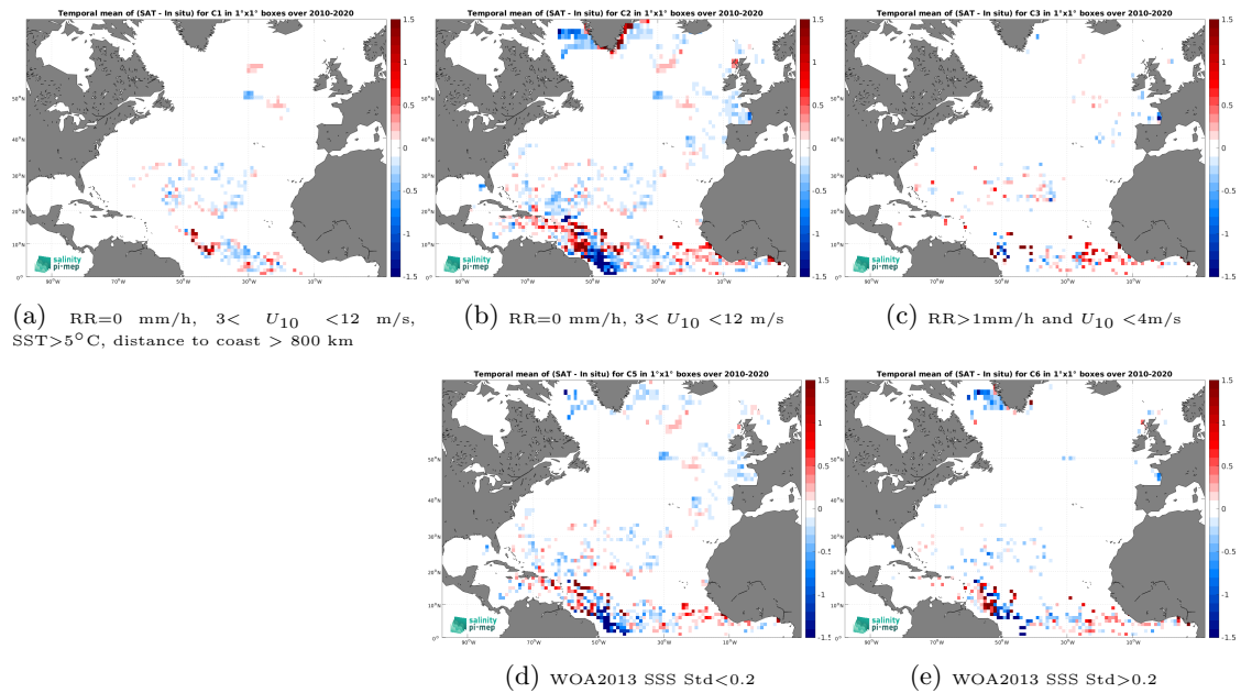
Figure 13: Temporal mean gridded over spatial boxes of size 1^\circ \times 1^\circ of \Delta SSS (SMOS SSS L4 v1 - Daily (CMEMS-CNR) - Surface drifters) for 5 different subdatasets corresponding to:RR=0 mm/h, 3 < U_{10} < 12 m/s, SST >5^\circ\text{C} , distance to coast > 800 km (a), RR=0 mm/h, 3 < U_{10} < 12 m/s (b), RR >1 mm/h and U_{10} < 4 m/s (c), WOA2013 SSS Std <0.2 (d), WOA2013 SSS Std >0.2 (e).
