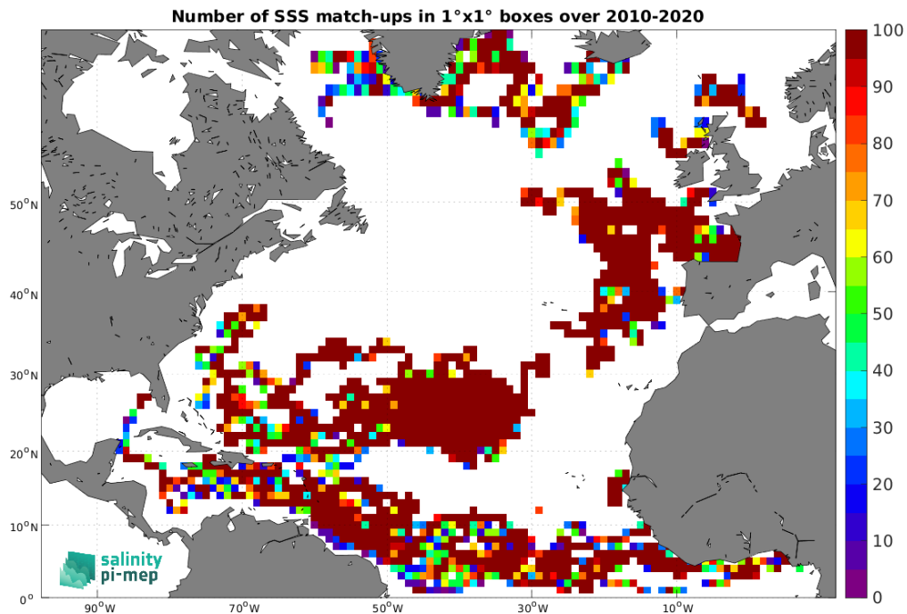
Figure 4: Number of SSS match-ups between Surface drifters SSS and the SMOS SSS L4 v1 - Daily (CMEMS-CNR) SSS product for the North Atlantic Ocean Pi-MEP region over 1^\circ \times 1^\circ boxes and for the full satellite product period.
