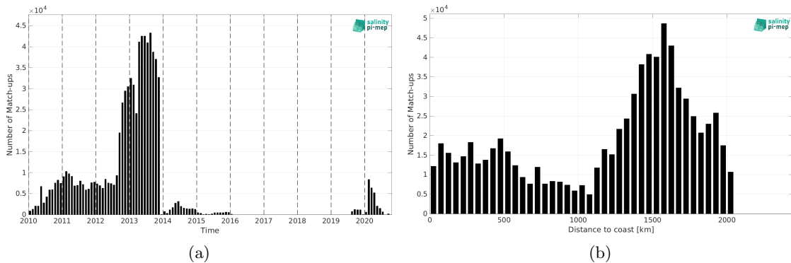
Figure 2: Number of match-ups between Surface drifters and SMOS SSS L4 v1 - Daily (CMEMS-CNR) SSS as a function of time (a) and as function of the distance to coast (b) over the North Atlantic Ocean Pi-MEP region and for the full satellite product period.
