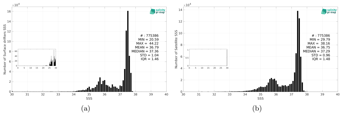
Figure 3: Histograms of SSS from Surface drifters (a) and SMOS SSS L4 v1 - Daily (CMEMS-CNR) (b) considering all match-up pairs per bins of 0.1 over the North Atlantic Ocean Pi-MEP region and for the full satellite product period.
