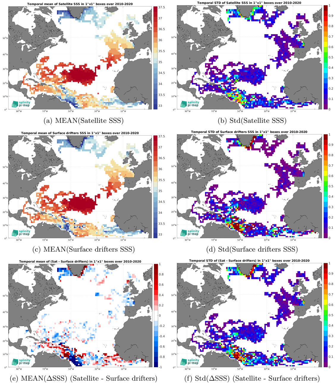
Figure 6: Temporal mean (left) and Std (right) of SSS from SMOS SSS L4 v1 - Daily (CMEMS-CNR) (top), Surface drifters (middle), and of \Delta SSS (Satellite - Surface drifters). Only match-up pairs are used to generate these maps.
