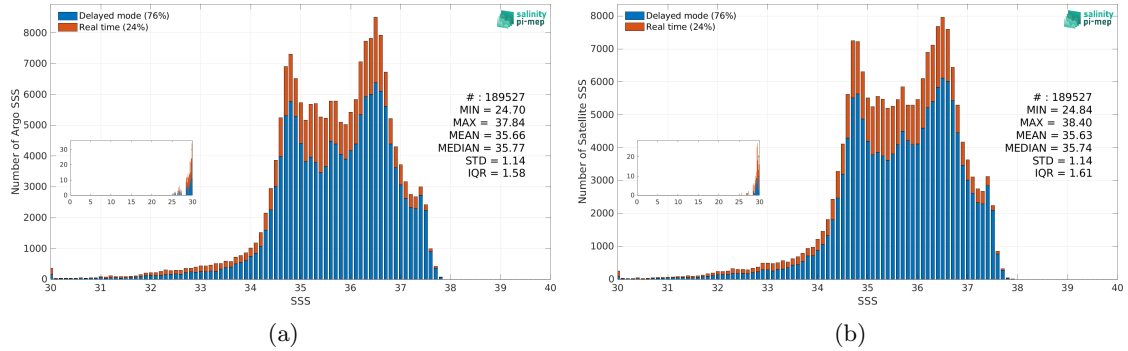
Figure 3: Histograms of SSS from Argo (a) and SMOS SSS L4 v1 - Daily (CMEMS-CNR) (b) considering all match-up pairs per bins of 0.1 over the North Atlantic Ocean Pi-MEP region and for the full satellite product period.
