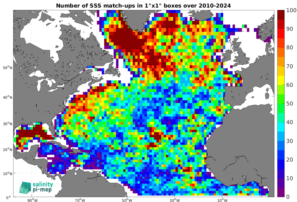
Figure 5: Number of SSS match-ups between Argo SSS and the SMOS SSS L4 v1 - Daily (CMEMS-CNR) SSS product for the North Atlantic Ocean Pi-MEP region over 1^\circ \times 1^\circ boxes and for the full satellite product period.
