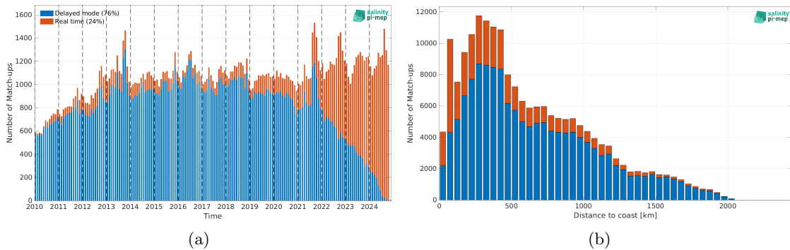
Figure 2: Number of match-ups between Argo and SMOS SSS L4 v1 - Daily (CMEMS-CNR) SSS as a function of time (a) and as function of the distance to coast (b) over the North Atlantic Ocean Pi-MEP region and for the full satellite product period.
