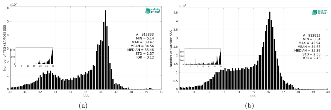
Figure 3: Histograms of SSS from TSG (SAMOS) (a) and SMOS SSS L4 OI v346 - Weekly (CMEMS-CATDS-LOPS) (b) considering all match-up pairs per bins of 0.1 over the North Atlantic Ocean Pi-MEP region and for the full satellite product period.
