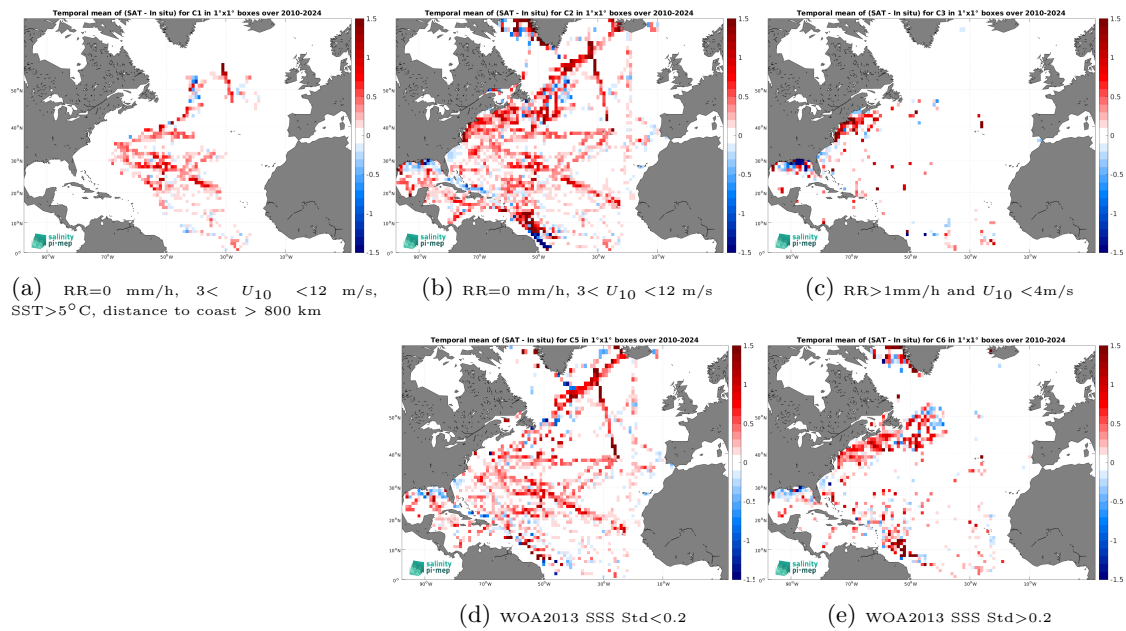
Figure 14: Temporal mean gridded over spatial boxes of size 1^\circ \times 1^\circ of \Delta\text{SSS} (SMOS SSS L4 OI v346 - Weekly (CMEMS-CATDS-LOPS) - TSG (SAMOS)) for 5 different subdatasets corresponding to:RR=0 mm/h, 3 < U_{10} < 12 m/s, SST>5°C, distance to coast > 800 km (a), RR=0 mm/h, 3 < U_{10} < 12 m/s (b), RR>1mm/h and U_{10} < 4 m/s (c), WOA2013 SSS Std<0.2 (d), WOA2013 SSS Std>0.2 (e).
