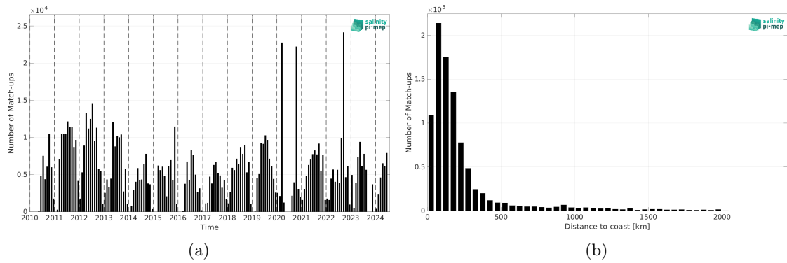
Figure 2: Number of match-ups between TSG (SAMOS) and SMOS SSS L4 OI v346 - Weekly (CMEMS-CATDS-LOPS) SSS as a function of time (a) and as function of the distance to coast (b) over the North Atlantic Ocean Pi-MEP region and for the full satellite product period.
