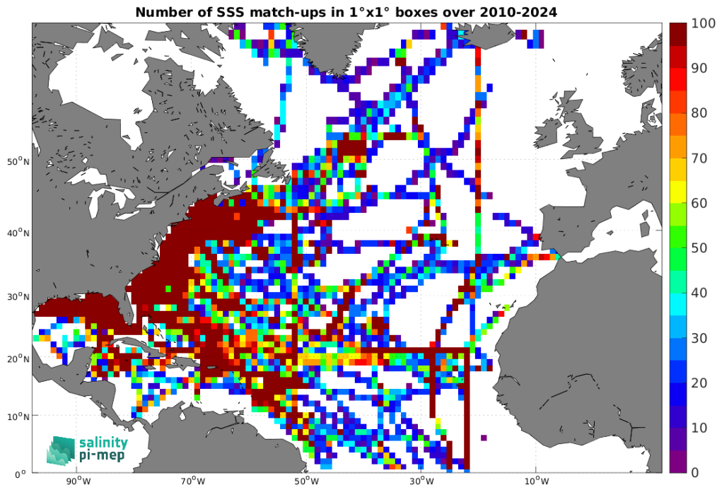
Figure 5: Number of SSS match-ups between TSG (SAMOS) SSS and the SMOS SSS L4 OI v346 - Weekly (CMEMS-CATDS-LOPS) SSS product for the North Atlantic Ocean Pi-MEP region over 1^\circ \times 1^\circ boxes and for the full satellite product period.
