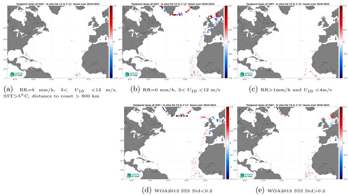
Figure 14: Temporal mean gridded over spatial boxes of size 1^\circ \times 1^\circ of \Delta\text{SSS} (SMOS SSS L4 OI v346 - Weekly (CMEMS-CATDS-LOPS) - TSG (Polarstern)) for 5 different subdatasets corresponding to:RR=0 mm/h, 3 < U_{10} < 12 m/s, SST >5^\circ\text{C} , distance to coast > 800 km (a), RR=0 mm/h, 3 < U_{10} < 12 m/s (b), RR >1 mm/h and U_{10} < 4 m/s (c), WOA2013 SSS Std <0.2 (d), WOA2013 SSS Std >0.2 (e).
