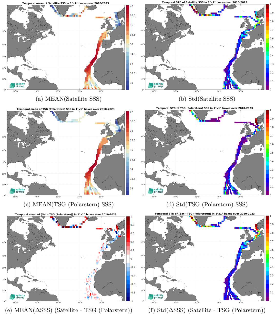
Figure 7: Temporal mean (left) and Std (right) of SSS from SMOS SSS L4 OI v346 - Weekly (CMEMS-CATDS-LOPS) (top), TSG (Polarstern) (middle), and of \Delta SSS (Satellite - TSG (Polarstern)). Only match-up pairs are used to generate these maps.
