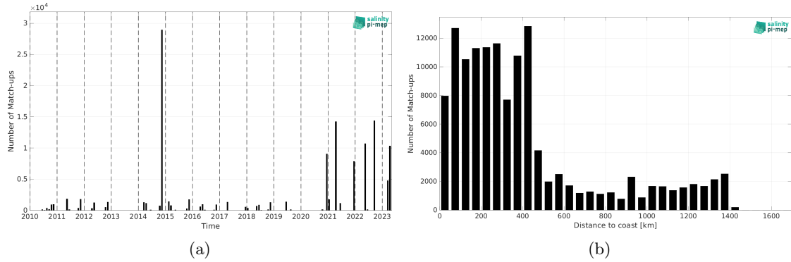
Figure 2: Number of match-ups between TSG (Polarstern) and SMOS SSS L4 OI v346 - Weekly (CMEMS-CATDS-LOPS) SSS as a function of time (a) and as function of the distance to coast (b) over the North Atlantic Ocean Pi-MEP region and for the full satellite product period.
