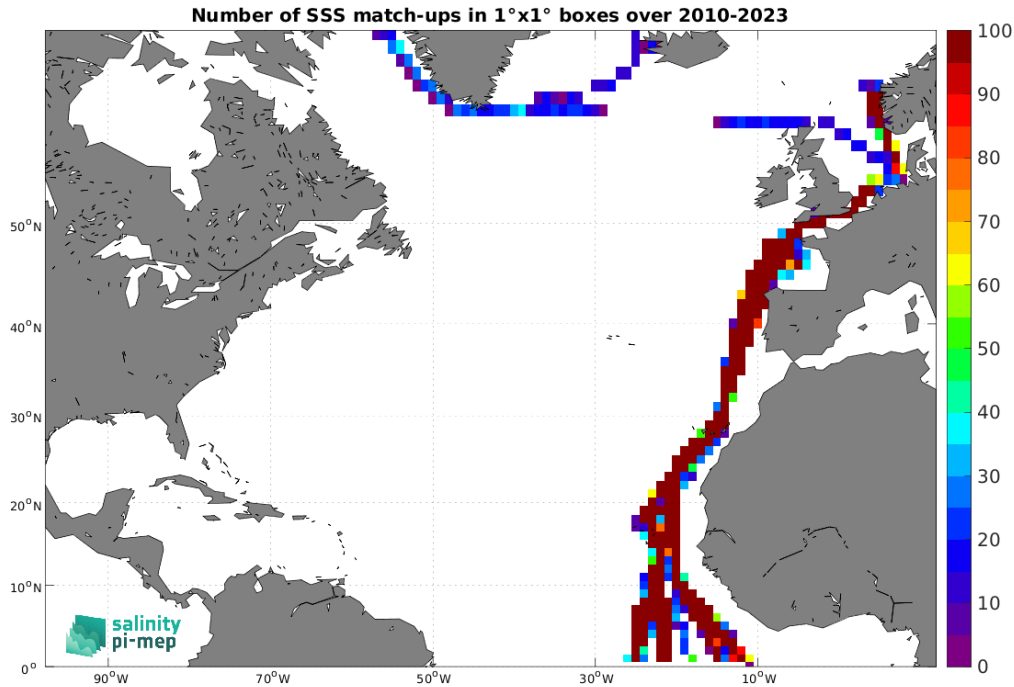
Figure 5: Number of SSS match-ups between TSG (Polarstern) SSS and the SMOS SSS L4 OI v346 - Weekly (CMEMS-CATDS-LOPS) SSS product for the North Atlantic Ocean Pi-MEP region over 1^\circ \times 1^\circ boxes and for the full satellite product period.
