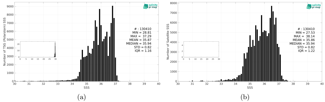
Figure 3: Histograms of SSS from TSG (Polarstern) (a) and SMOS SSS L4 OI v346 - Weekly (CMEMS-CATDS-LOPS) (b) considering all match-up pairs per bins of 0.1 over the North Atlantic Ocean Pi-MEP region and for the full satellite product period.
