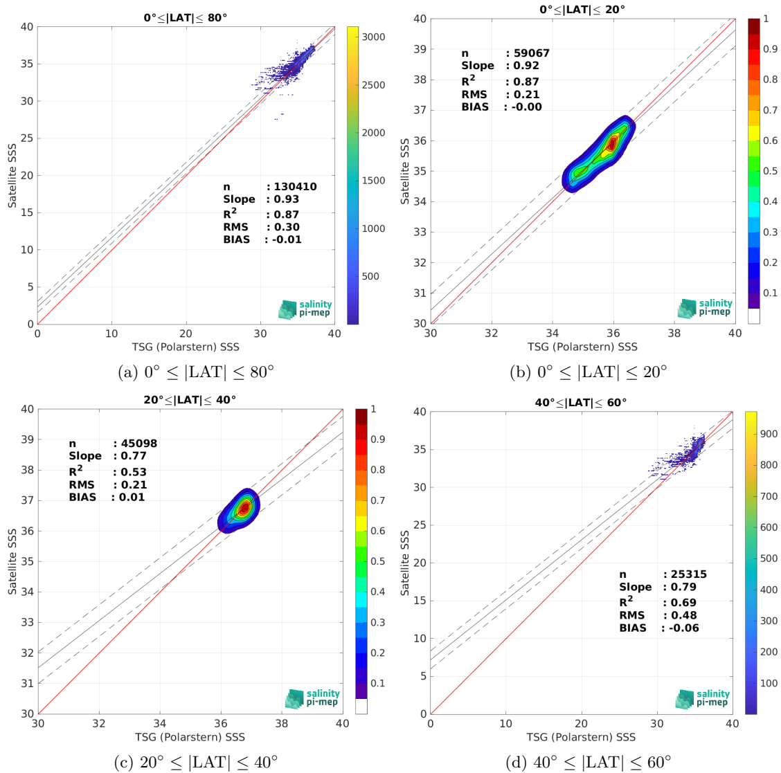
Figure 10: Contour maps of the concentration of SMOS SSS L4 OI v346 - Weekly (CMEMS-CATDS-LOPS) SSS ( y -axis) versus TSG (Polarstern) SSS ( x -axis) at match-up pairs for different latitude bands. For each plot, the red line shows x=y . The black thin and dashed lines indicate a linear fit through the data cloud and the \pm 95\% confidence levels, respectively. The number match-up pairs n , the slope and R^2 coefficient of the linear fit, the root mean square (RMS) and the mean bias between satellite and in situ data are indicated for each latitude band in each plots.
