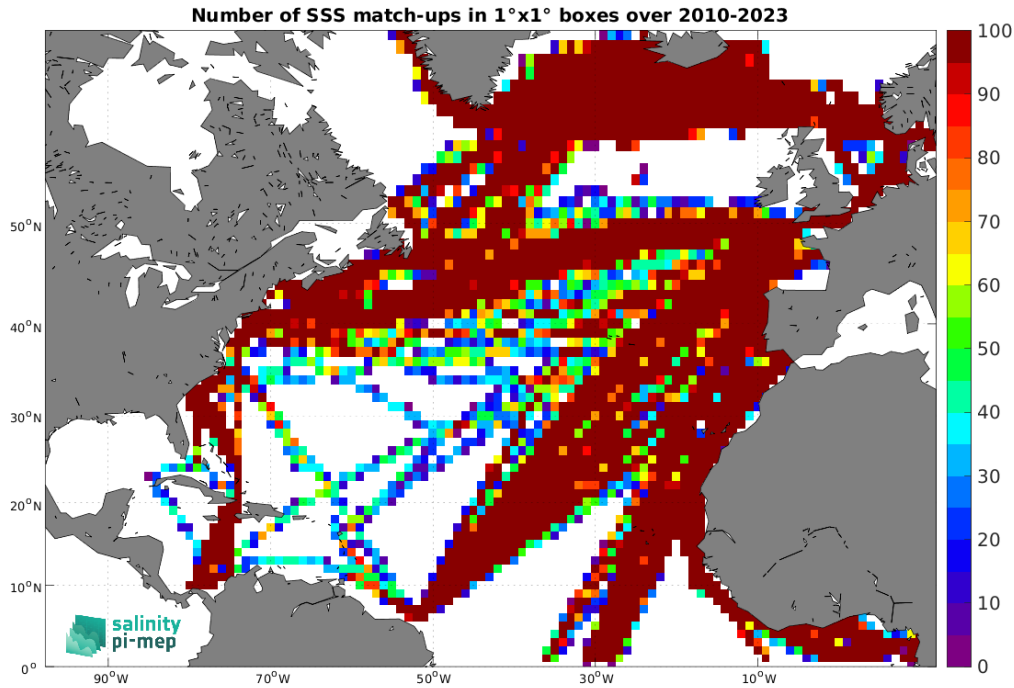
Figure 5: Number of SSS match-ups between TSG (LEGOS-DM) SSS and the SMOS SSS L4 OI v346 - Weekly (CMEMS-CATDS-LOPS) SSS product for the North Atlantic Ocean Pi-MEP region over 1^\circ \times 1^\circ boxes and for the full satellite product period.
