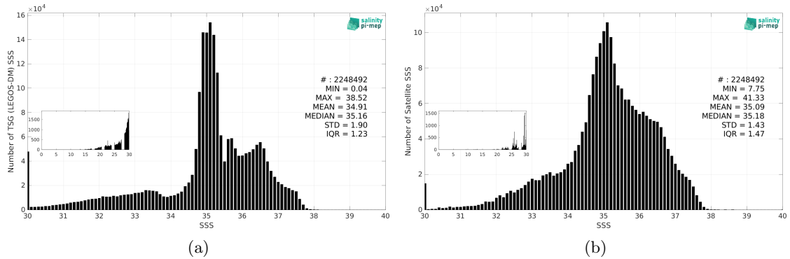
Figure 3: Histograms of SSS from TSG (LEGOS-DM) (a) and SMOS SSS L4 OI v346 - Weekly (CMEMS-CATDS-LOPS) (b) considering all match-up pairs per bins of 0.1 over the North Atlantic Ocean Pi-MEP region and for the full satellite product period.
