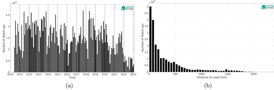
Figure 2: Number of match-ups between TSG (LEGOS-DM) and SMOS SSS L4 OI v346 - Weekly (CMEMS-CATDS-LOPS) SSS as a function of time (a) and as function of the distance to coast (b) over the North Atlantic Ocean Pi-MEP region and for the full satellite product period.
