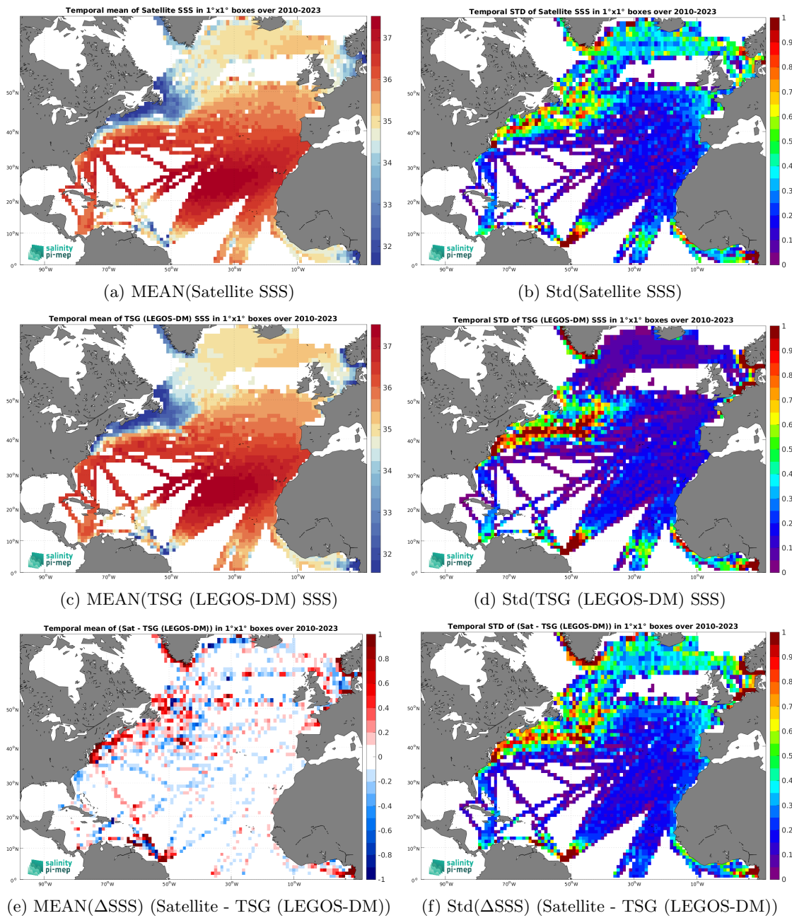
Figure 7: Temporal mean (left) and Std (right) of SSS from SMOS SSS L4 OI v346 - Weekly (CMEMS-CATDS-LOPS) (top), TSG (LEGOS-DM) (middle), and of \Delta SSS (Satellite - TSG (LEGOS-DM)). Only match-up pairs are used to generate these maps.
