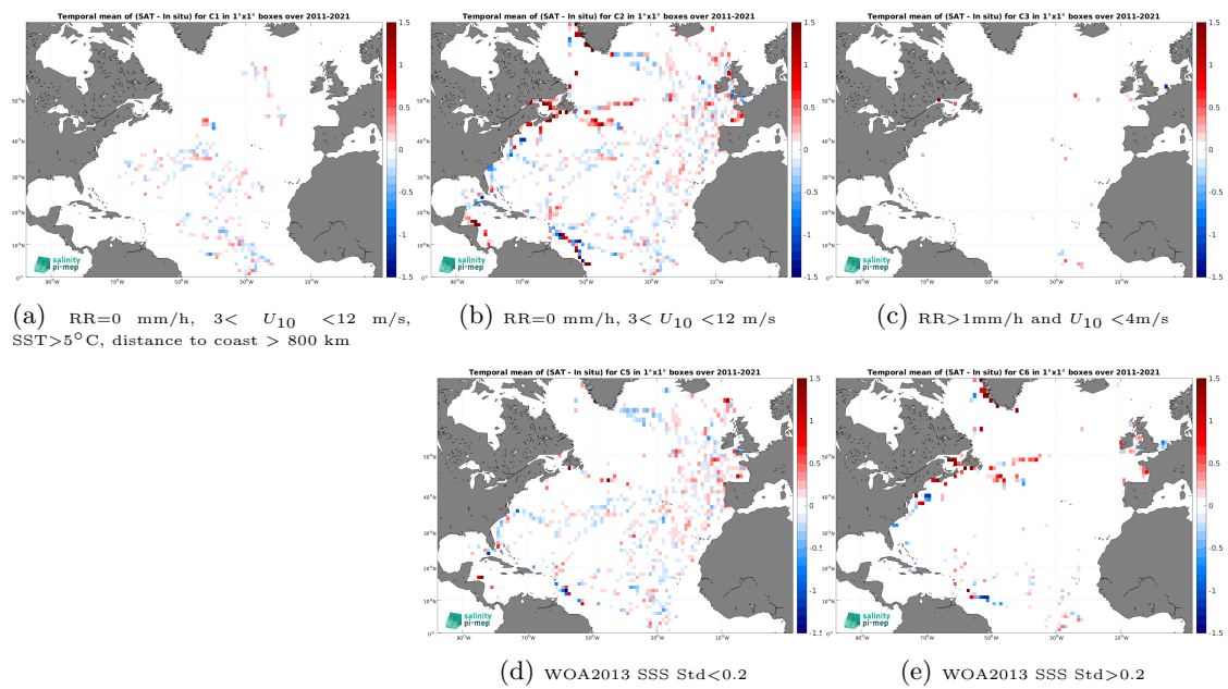
Figure 14: Temporal mean gridded over spatial boxes of size 1^\circ \times 1^\circ of \Delta\text{SSS} (SMOS SSS L4 OI v346 - Weekly (CMEMS-CATDS-LOPS) - TSG (GOSUD-Sailing-ship)) for 5 different sub-datasets corresponding to:RR=0 mm/h, 3 < U_{10} < 12 m/s, SST >5^\circ\text{C} , distance to coast > 800 km (a), RR=0 mm/h, 3 < U_{10} < 12 m/s (b), RR >1 mm/h and U_{10} < 4 m/s (c), WOA2013 SSS Std <0.2 (d), WOA2013 SSS Std >0.2 (e).
