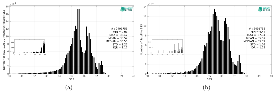
Figure 3: Histograms of SSS from TSG (GOSUD-Research-vessel) (a) and SMOS SSS L4 OI v346 - Weekly (CMEMS-CATDS-LOPS) (b) considering all match-up pairs per bins of 0.1 over the North Atlantic Ocean Pi-MEP region and for the full satellite product period.
