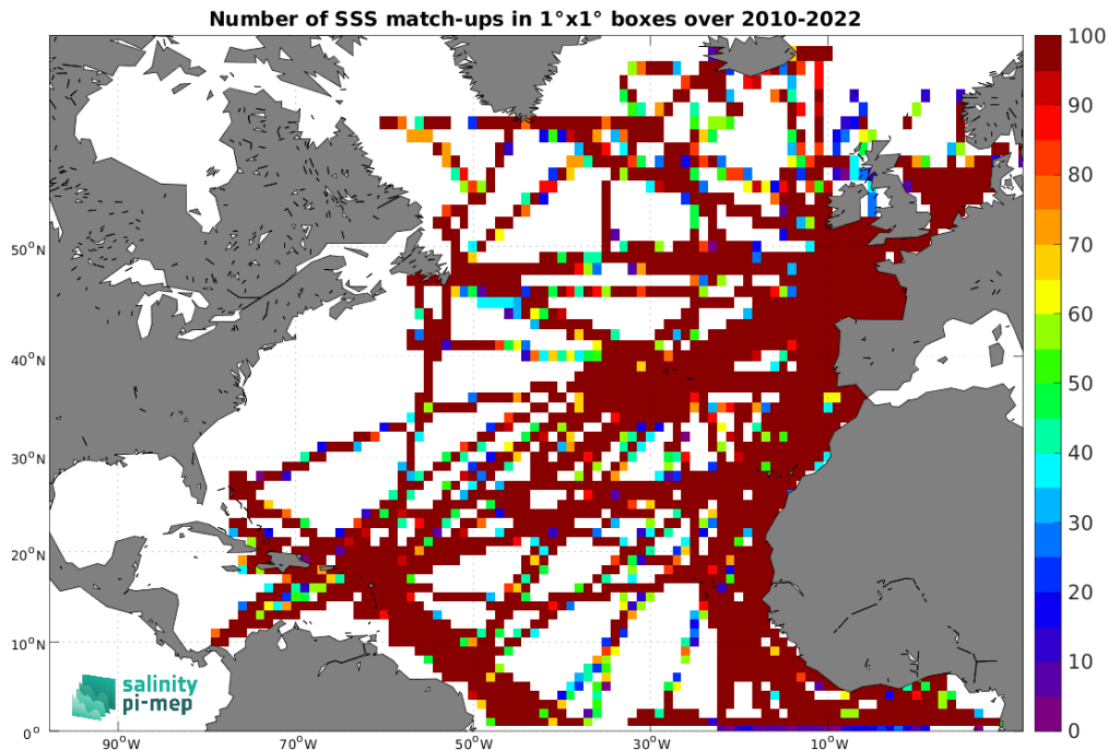
Figure 5: Number of SSS match-ups between TSG (GOSUD-Research-vessel) SSS and the SMOS SSS L4 OI v346 - Weekly (CMEMS-CATDS-LOPS) SSS product for the North Atlantic Ocean Pi-MEP region over 1^\circ \times 1^\circ boxes and for the full satellite product period.
