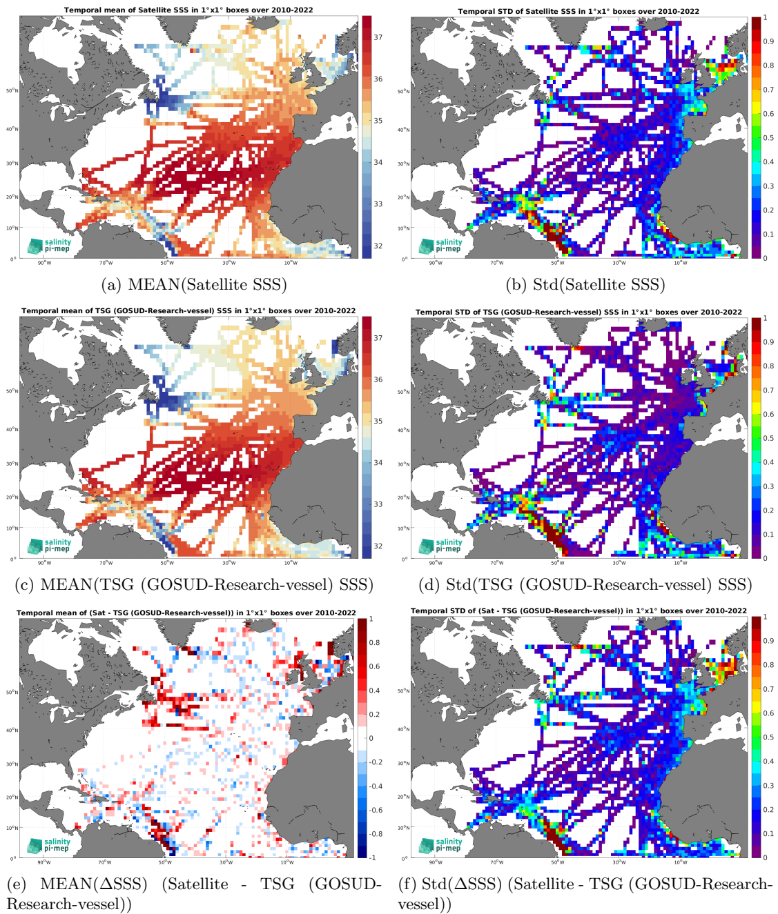
Figure 7: Temporal mean (left) and Std (right) of SSS from SMOS SSS L4 OI v346 - Weekly (CMEMS-CATDS-LOPS) (top), TSG (GOSUD-Research-vessel) (middle), and of \Delta SSS (Satellite - TSG (GOSUD-Research-vessel)). Only match-up pairs are used to generate these maps.
