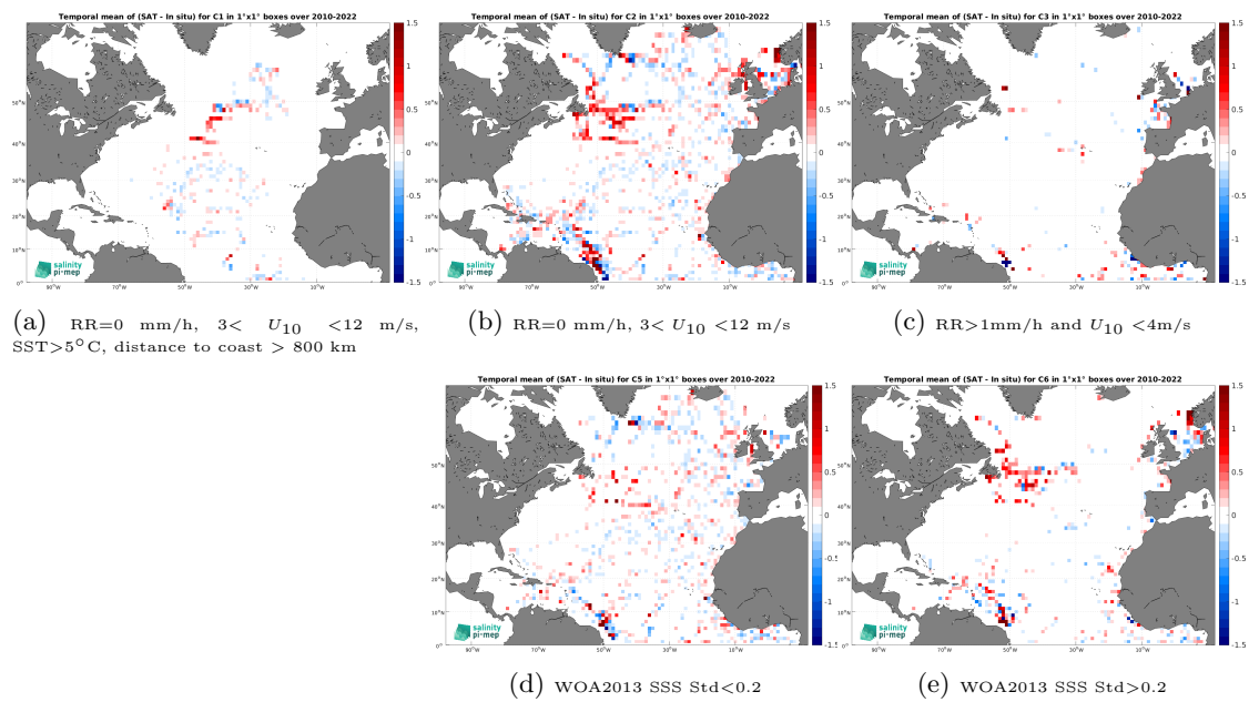
Figure 14: Temporal mean gridded over spatial boxes of size 1^\circ \times 1^\circ of \Delta SSS (SMOS SSS L4 OI v346 - Weekly (CMEMS-CATDS-LOPS) - TSG (GOSUD-Research-vessel)) for 5 different subdatasets corresponding to:RR=0 mm/h, 3 < U_{10} < 12 m/s, SST >5^\circ\text{C} , distance to coast > 800 km (a), RR=0 mm/h, 3 < U_{10} < 12 m/s (b), RR >1 mm/h and U_{10} < 4 m/s (c), WOA2013 SSS Std <0.2 (d), WOA2013 SSS Std >0.2 (e).
