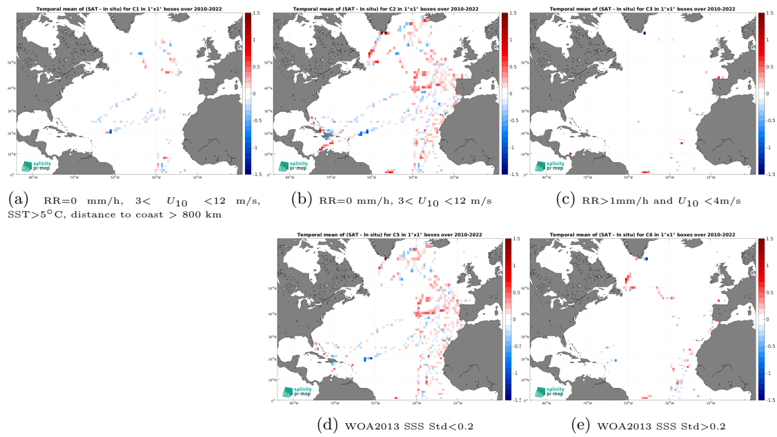
Figure 14: Temporal mean gridded over spatial boxes of size 1^\circ \times 1^\circ of \Delta\text{SSS} (SMOS SSS L4 OI v346 - Weekly (CMEMS-CATDS-LOPS) - TSG (CSIC-UTM)) for 5 different subdatasets corresponding to:RR=0 mm/h, 3 < U_{10} < 12 m/s, SST > 5°C, distance to coast > 800 km (a), RR=0 mm/h, 3 < U_{10} < 12 m/s (b), RR > 1mm/h and U_{10} < 4 m/s (c), WOA2013 SSS Std < 0.2 (d), WOA2013 SSS Std > 0.2 (e).
