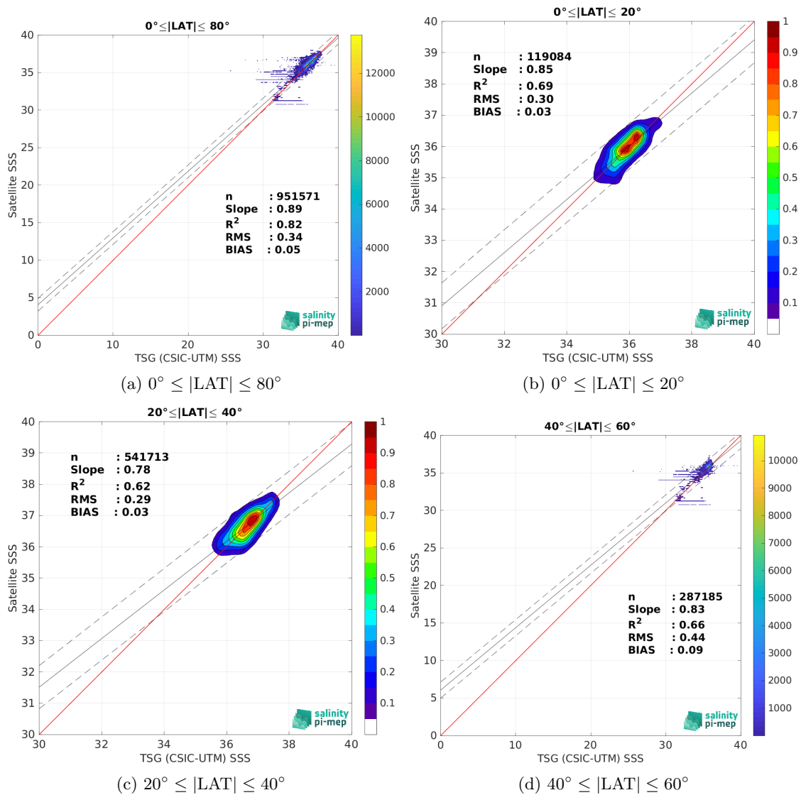
Figure 10: Contour maps of the concentration of SMOS SSS L4 OI v346 - Weekly (CMEMS-CATDS-LOPS) SSS (y-axis) versus TSG (CSIC-UTM) SSS (x-axis) at match-up pairs for different latitude bands. For each plot, the red line shows x=y . The black thin and dashed lines indicate a linear fit through the data cloud and the \pm 95\% confidence levels, respectively. The number match-up pairs n , the slope and R^2 coefficient of the linear fit, the root mean square (RMS) and the mean bias between satellite and in situ data are indicated for each latitude band in each plots.
