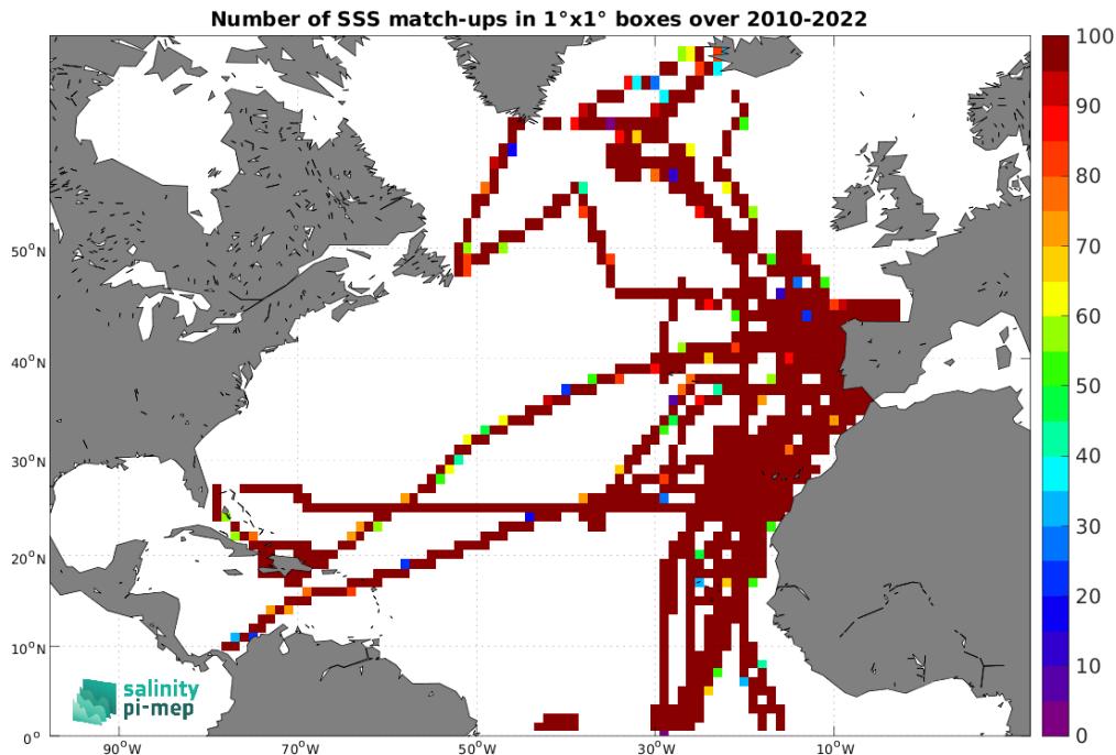
Figure 5: Number of SSS match-ups between TSG (CSIC-UTM) SSS and the SMOS SSS L4 OI v346 - Weekly (CMEMS-CATDS-LOPS) SSS product for the North Atlantic Ocean Pi-MEP region over 1^\circ \times 1^\circ boxes and for the full satellite product period.
