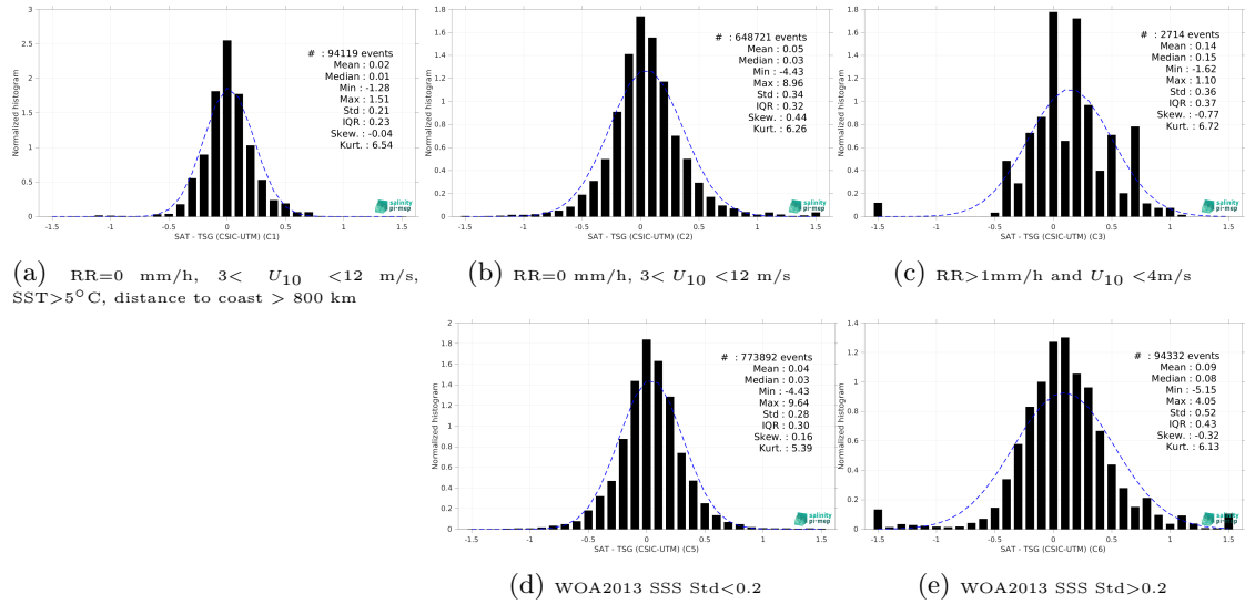
Figure 15: Normalized histogram of \Delta\text{SSS} (SMOS SSS L4 OI v346 - Weekly (CMEMS-CATDS-LOPS) - TSG (CSIC-UTM)) for 5 different subdatasets corresponding to: RR=0 mm/h, 3 < U_{10} < 12 m/s, SST > 5^\circ\text{C} , distance to coast > 800 km (a), RR=0 mm/h, 3 < U_{10} < 12 m/s (b), RR > 1 mm/h and U_{10} < 4 m/s (c), WOA2013 SSS Std < 0.2 (d), WOA2013 SSS Std > 0.2 (e).
