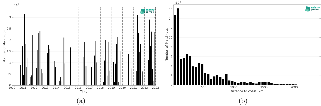
Figure 2: Number of match-ups between TSG (CSIC-UTM) and SMOS SSS L4 OI v346 - Weekly (CMEMS-CATDS-LOPS) SSS as a function of time (a) and as function of the distance to coast (b) over the North Atlantic Ocean Pi-MEP region and for the full satellite product period.
