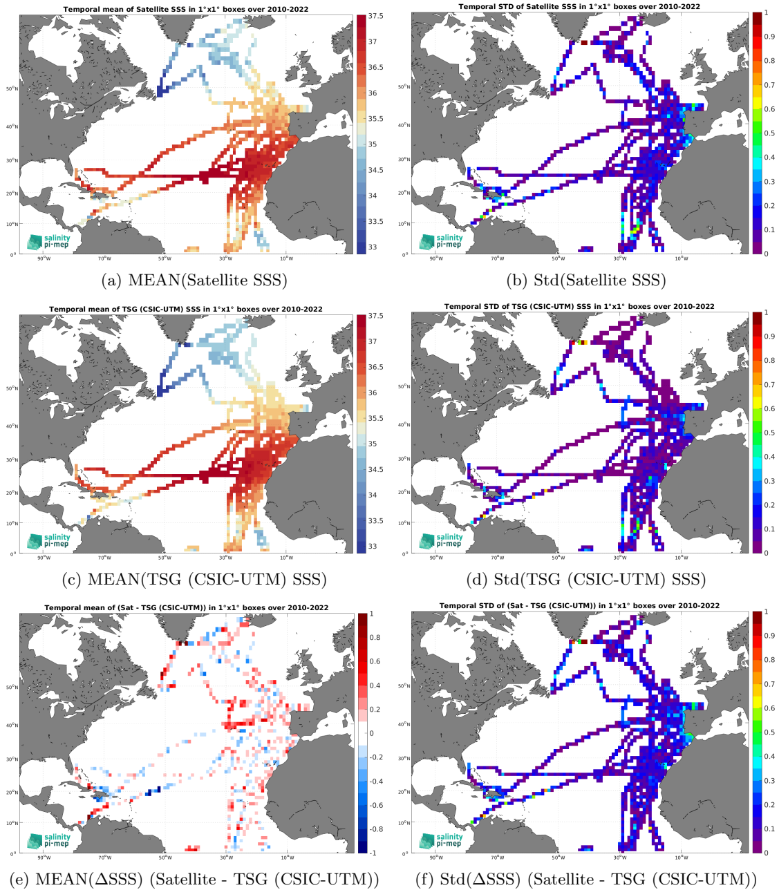
Figure 7: Temporal mean (left) and Std (right) of SSS from SMOS SSS L4 OI v346 - Weekly (CMEMS-CATDS-LOPS) (top), TSG (CSIC-UTM) (middle), and of \Delta SSS (Satellite - TSG (CSIC-UTM)). Only match-up pairs are used to generate these maps.
