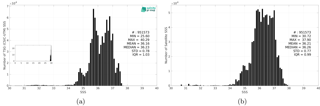
Figure 3: Histograms of SSS from TSG (CSIC-UTM) (a) and SMOS SSS L4 OI v346 - Weekly (CMEMS-CATDS-LOPS) (b) considering all match-up pairs per bins of 0.1 over the North Atlantic Ocean Pi-MEP region and for the full satellite product period.
