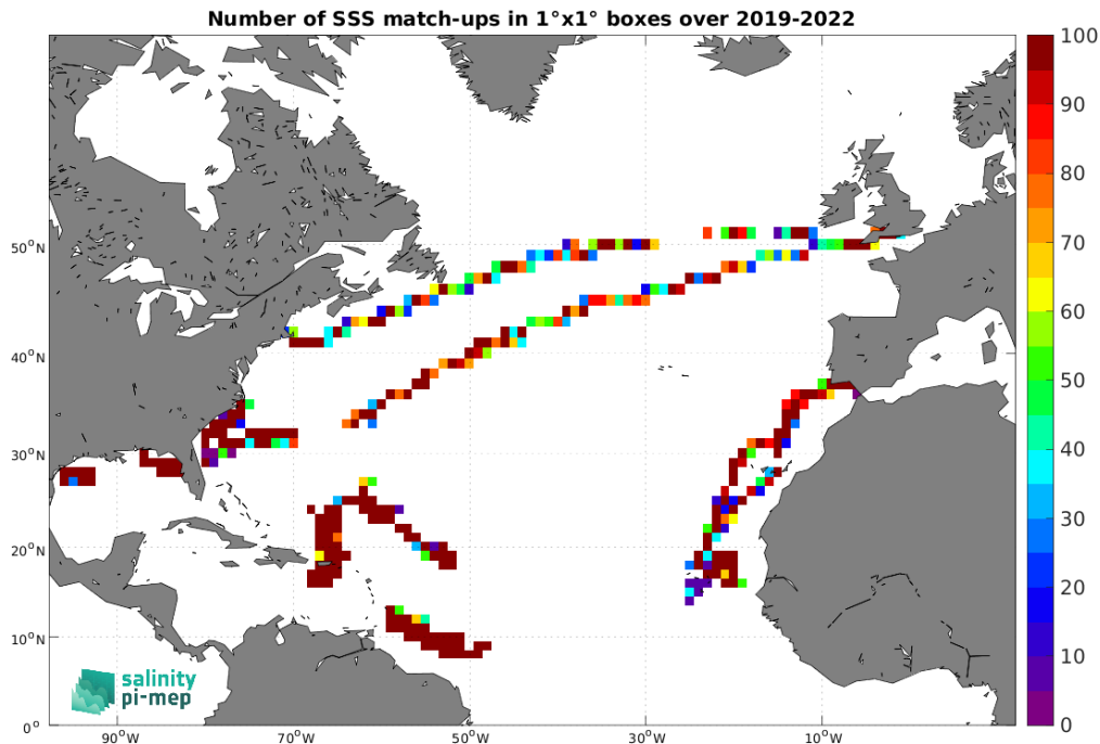
Figure 5: Number of SSS match-ups between Saildrone SSS and the SMOS SSS L4 OI v346 - Weekly (CMEMS-CATDS-LOPS) SSS product for the North Atlantic Ocean Pi-MEP region over 1^\circ \times 1^\circ boxes and for the full satellite product period.
