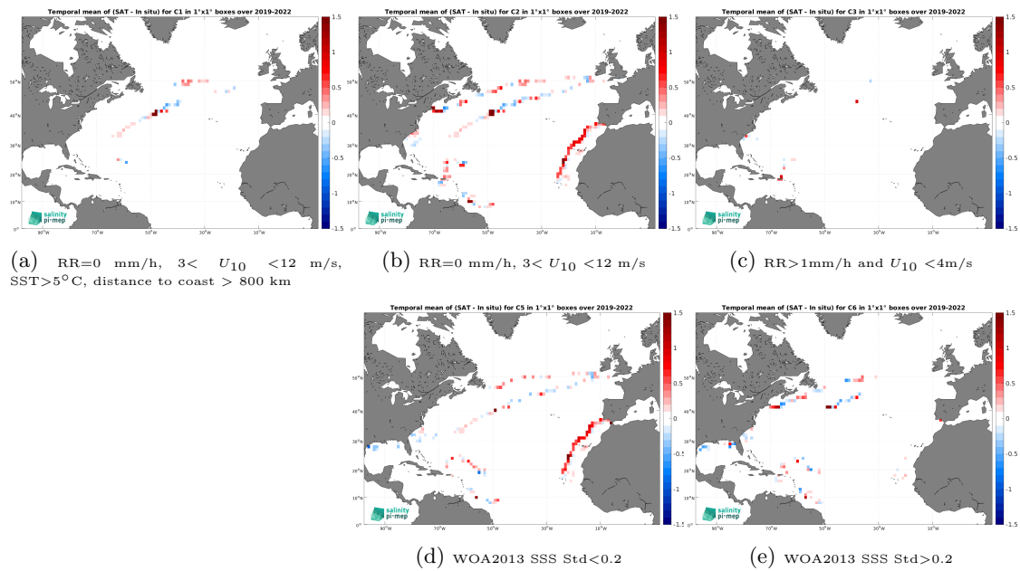
Figure 14: Temporal mean gridded over spatial boxes of size 1^\circ \times 1^\circ of \Delta\text{SSS} (SMOS SSS L4 OI v346 - Weekly (CMEMS-CATDS-LOPS) - Saildrone) for 5 different subdatasets corresponding to:RR=0 mm/h, 3 < U_{10} < 12 m/s, SST>5°C, distance to coast > 800 km (a), RR=0 mm/h, 3 < U_{10} < 12 m/s (b), RR>1mm/h and U_{10} < 4 m/s (c), WOA2013 SSS Std<0.2 (d), WOA2013 SSS Std>0.2 (e).
