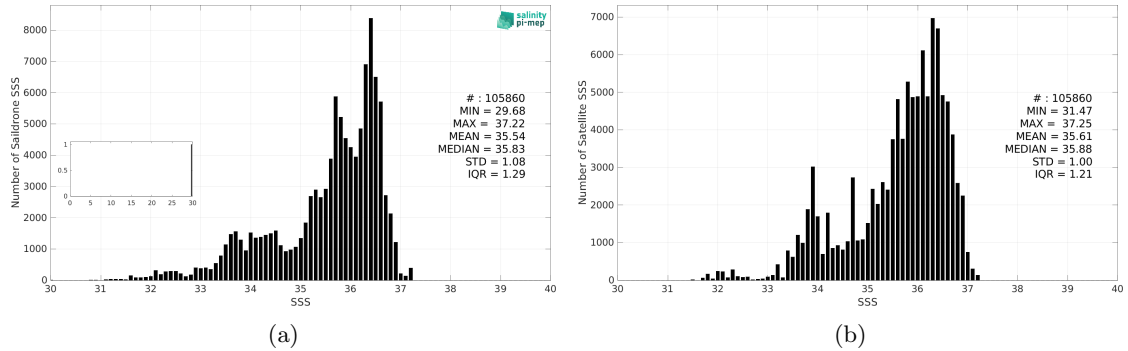
Figure 3: Histograms of SSS from Saildrone (a) and SMOS SSS L4 OI v346 - Weekly (CMEMS-CATDS-LOPS) (b) considering all match-up pairs per bins of 0.1 over the North Atlantic Ocean Pi-MEP region and for the full satellite product period.
