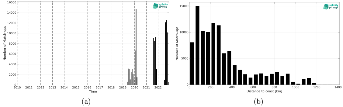
Figure 2: Number of match-ups between Saildrone and SMOS SSS L4 OI v346 - Weekly (CMEMS-CATDS-LOPS) SSS as a function of time (a) and as function of the distance to coast (b) over the North Atlantic Ocean Pi-MEP region and for the full satellite product period.
