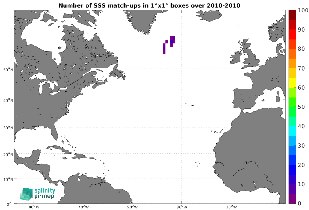
Figure 5: Number of SSS match-ups between Marine mammals SSS and the SMOS SSS L4 OI v346 - Weekly (CMEMS-CATDS-LOPS) SSS product for the North Atlantic Ocean Pi-MEP region over 1^\circ \times 1^\circ boxes and for the full satellite product period.
