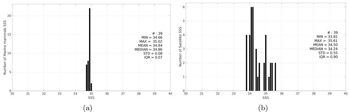
Figure 3: Histograms of SSS from Marine mammals (a) and SMOS SSS L4 OI v346 - Weekly (CMEMS-CATDS-LOPS) (b) considering all match-up pairs per bins of 0.1 over the North Atlantic Ocean Pi-MEP region and for the full satellite product period.
