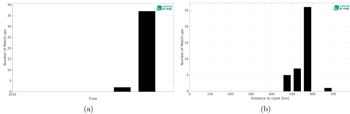
Figure 2: Number of match-ups between Marine mammals and SMOS SSS L4 OI v346 - Weekly (CMEMS-CATDS-LOPS) SSS as a function of time (a) and as function of the distance to coast (b) over the North Atlantic Ocean Pi-MEP region and for the full satellite product period.
