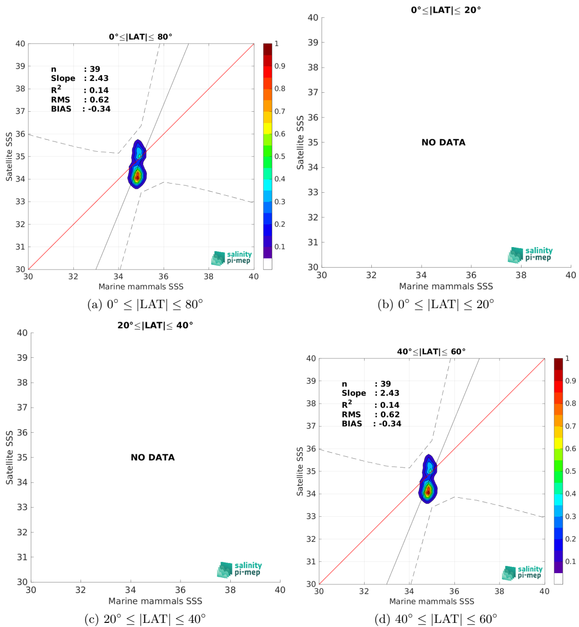
Figure 10: Contour maps of the concentration of SMOS SSS L4 OI v346 - Weekly (CMEMS-CATDS-LOPS) SSS (y-axis) versus Marine mammals SSS (x-axis) at match-up pairs for different latitude bands. For each plot, the red line shows x=y . The black thin and dashed lines indicate a linear fit through the data cloud and the \pm 95\% confidence levels, respectively. The number match-up pairs n , the slope and R^2 coefficient of the linear fit, the root mean square (RMS) and the mean bias between satellite and in situ data are indicated for each latitude band in each plots.
