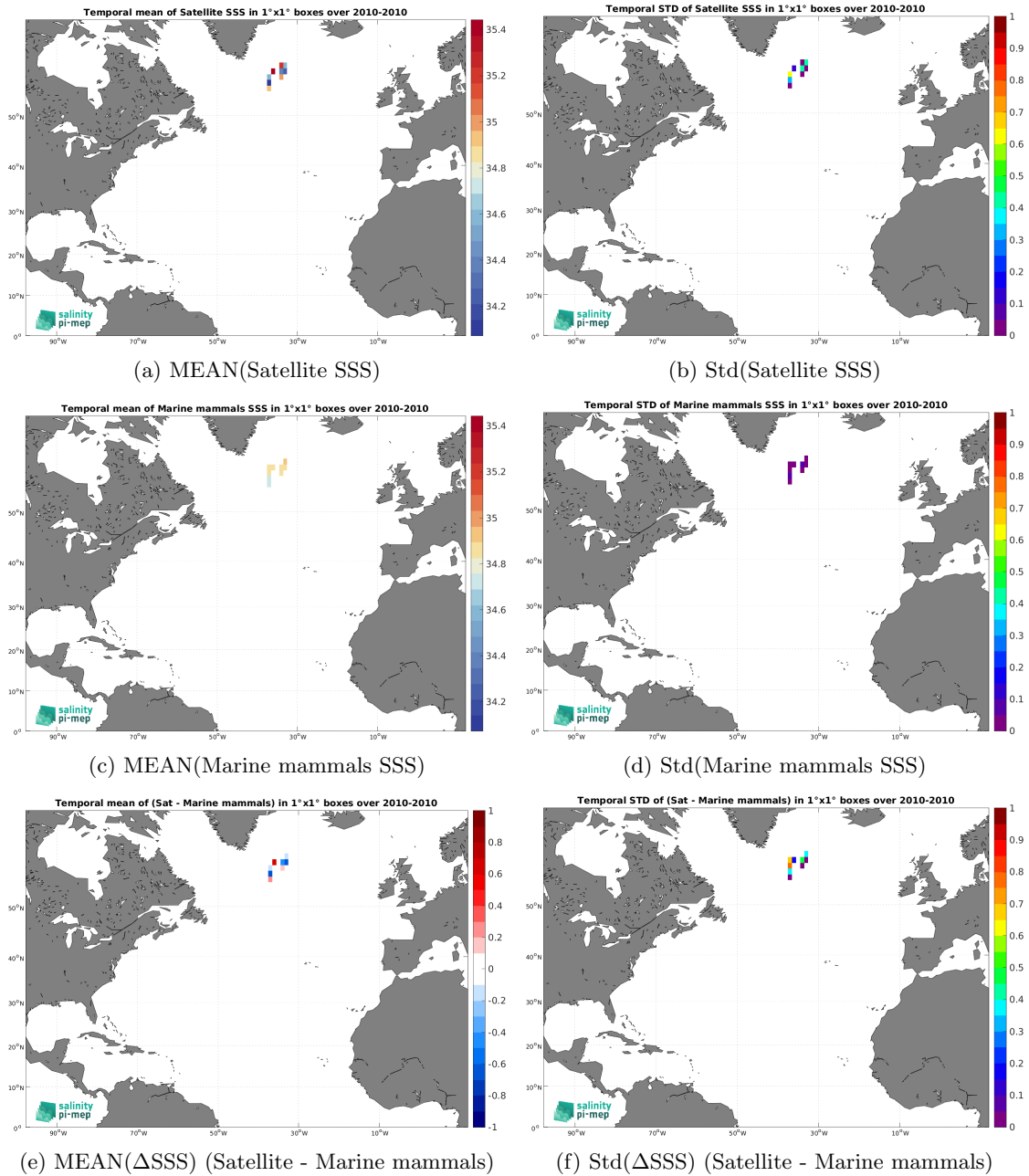
Figure 7: Temporal mean (left) and Std (right) of SSS from SMOS SSS L4 OI v346 - Weekly (CMEMS-CATDS-LOPS) (top), Marine mammals (middle), and of \Delta SSS (Satellite - Marine mammals). Only match-up pairs are used to generate these maps.
