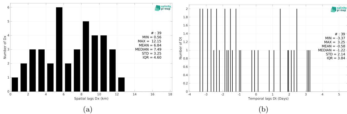
Figure 6: Histograms of the spatial (a) and temporal (b) lags between the location/time of the Marine mammals measurement and the date of the corresponding SMOS SSS L4 OI v346 - Weekly (CMEMS-CATDS-LOPS) SSS pixel.
