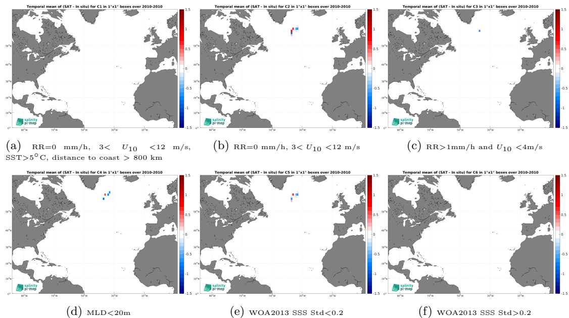
Figure 14: Temporal mean gridded over spatial boxes of size 1^\circ \times 1^\circ of \Delta SSS (SMOS SSS L4 OI v346 - Weekly (CMEMS-CATDS-LOPS) - Marine mammals) for 6 different subdatasets corresponding to:RR=0 mm/h, 3 < U_{10} < 12 m/s, SST > 5^\circ\text{C} , distance to coast > 800 km (a), RR=0 mm/h, 3 < U_{10} < 12 m/s (b), RR > 1 mm/h and U_{10} < 4 m/s (c),MLD < 20 m (d),WOA2013 SSS Std < 0.2 (e),WOA2013 SSS Std > 0.2 (f).
