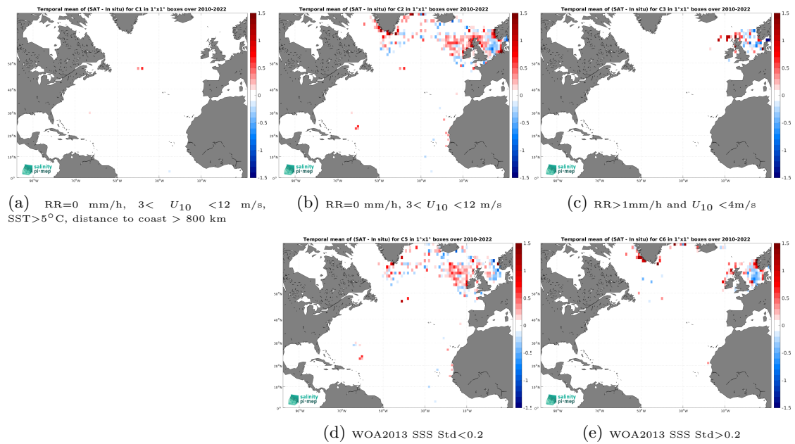
Figure 14: Temporal mean gridded over spatial boxes of size 1^\circ \times 1^\circ of \Delta\text{SSS} (SMOS SSS L4 OI v346 - Weekly (CMEMS-CATDS-LOPS) - ICES) for 5 different subdatasets corresponding to:RR=0 mm/h, 3 < U_{10} < 12 m/s, SST>5°C, distance to coast > 800 km (a), RR=0 mm/h, 3 < U_{10} < 12 m/s (b), RR>1mm/h and U_{10} < 4 m/s (c), WOA2013 SSS Std<0.2 (d), WOA2013 SSS Std>0.2 (e).
