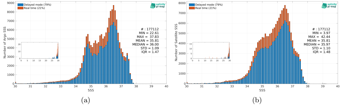
Figure 3: Histograms of SSS from Argo (a) and SMOS SSS L4 OI v346 - Weekly (CMEMS-CATDS-LOPS) (b) considering all match-up pairs per bins of 0.1 over the North Atlantic Ocean Pi-MEP region and for the full satellite product period.
