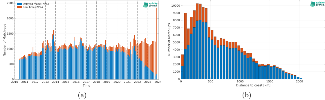
Figure 2: Number of match-ups between Argo and SMOS SSS L4 OI v346 - Weekly (CMEMS-CATDS-LOPS) SSS as a function of time (a) and as function of the distance to coast (b) over the North Atlantic Ocean Pi-MEP region and for the full satellite product period.
