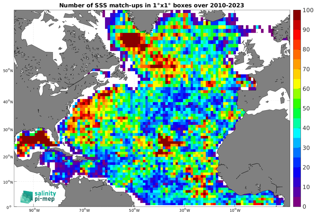
Figure 5: Number of SSS match-ups between Argo SSS and the SMOS SSS L4 OI v346 - Weekly (CMEMS-CATDS-LOPS) SSS product for the North Atlantic Ocean Pi-MEP region over 1^\circ \times 1^\circ boxes and for the full satellite product period.
