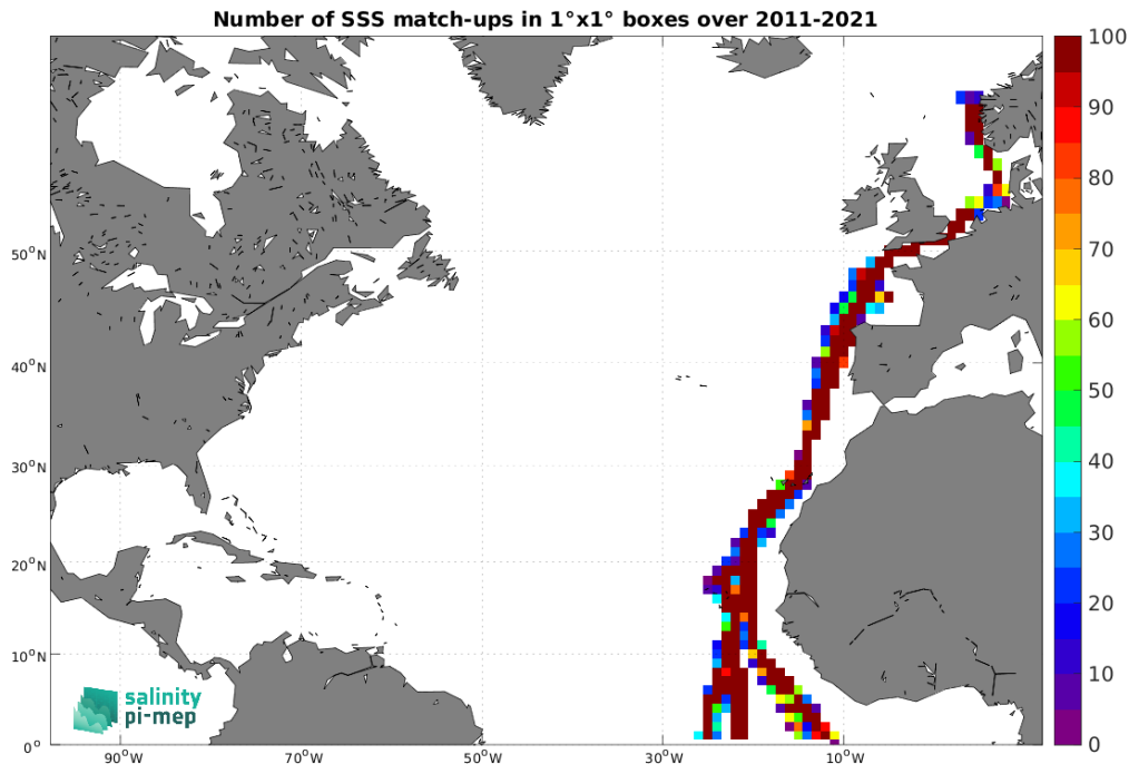
Figure 4: Number of SSS match-ups between TSG (Polarstern) SSS and the SMOS SSS L4 OI v342 - Weekly (CMEMS-CATDS-LOPS) SSS product for the North Atlantic Ocean Pi-MEP region over 1^\circ \times 1^\circ boxes and for the full satellite product period.
