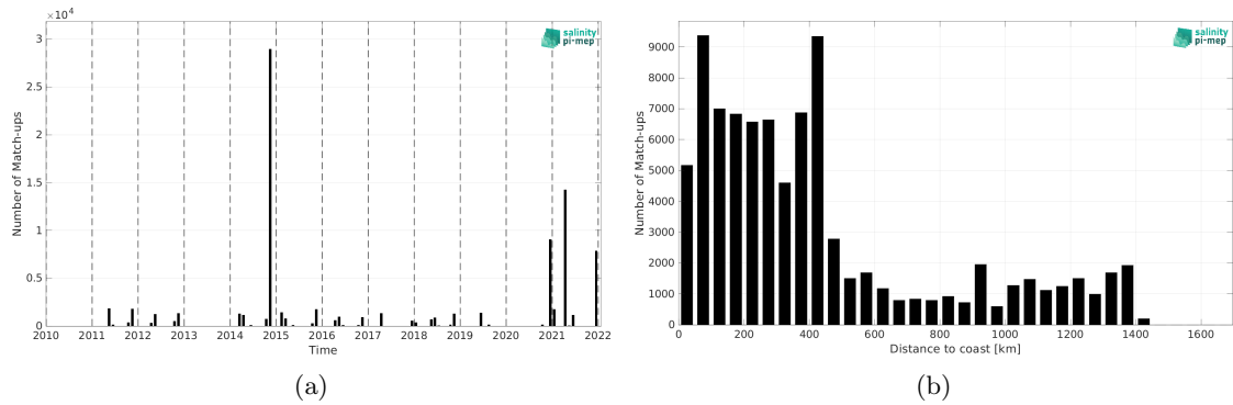
Figure 1: Number of match-ups between TSG (Polarstern) and SMOS SSS L4 OI v342 - Weekly (CMEMS-CATDS-LOPS) SSS as a function of time (a) and as function of the distance to coast (b) over the North Atlantic Ocean Pi-MEP region and for the full satellite product period.
