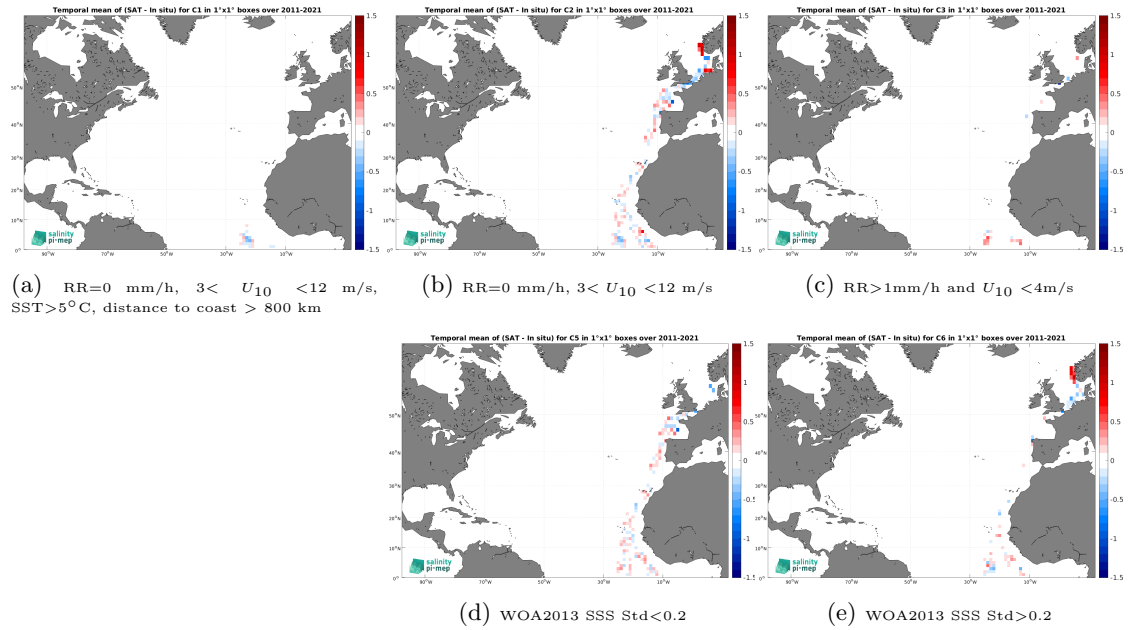
Figure 12: Temporal mean gridded over spatial boxes of size 1^\circ \times 1^\circ of \Delta\text{SSS} (SMOS SSS L4 OI v342 - Weekly (CMEMS-CATDS-LOPS) - TSG (Polarstern)) for 5 different subdatasets corresponding to:RR=0 mm/h, 3 < U_{10} < 12 m/s, SST >5^\circ\text{C} , distance to coast > 800 km (a), RR=0 mm/h, 3 < U_{10} < 12 m/s (b), RR >1 mm/h and U_{10} < 4 m/s (c), WOA2013 SSS Std <0.2 (d), WOA2013 SSS Std >0.2 (e).
