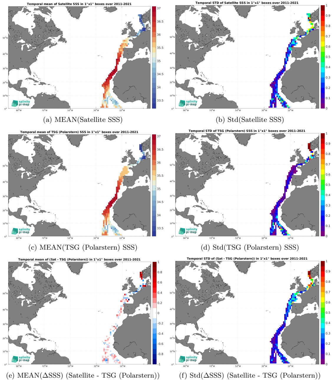
Figure 6: Temporal mean (left) and Std (right) of SSS from SMOS SSS L4 OI v342 - Weekly (CMEMS-CATDS-LOPS) (top), TSG (Polarstern) (middle), and of \Delta SSS (Satellite - TSG (Polarstern)). Only match-up pairs are used to generate these maps.
