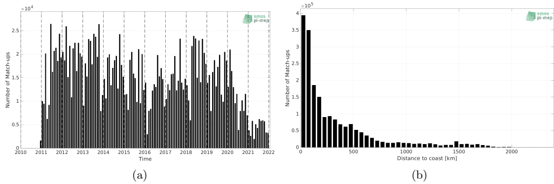
Figure 1: Number of match-ups between TSG (LEGOS-DM) and SMOS SSS L4 OI v342 - Weekly (CMEMS-CATDS-LOPS) SSS as a function of time (a) and as function of the distance to coast (b) over the North Atlantic Ocean Pi-MEP region and for the full satellite product period.
