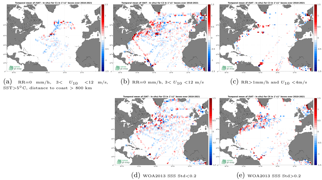
Figure 12: Temporal mean gridded over spatial boxes of size 1^\circ \times 1^\circ of \Delta\text{SSS} (SMOS SSS L4 OI v342 - Weekly (CMEMS-CATDS-LOPS) - TSG (LEGOS-DM)) for 5 different subdatasets corresponding to:RR=0 mm/h, 3 < U_{10} < 12 m/s, SST >5^\circ\text{C} , distance to coast > 800 km (a), RR=0 mm/h, 3 < U_{10} < 12 m/s (b), RR >1 mm/h and U_{10} < 4 m/s (c), WOA2013 SSS Std <0.2 (d), WOA2013 SSS Std >0.2 (e).
