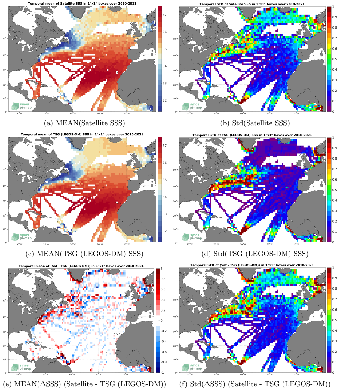
Figure 6: Temporal mean (left) and Std (right) of SSS from SMOS SSS L4 OI v342 - Weekly (CMEMS-CATDS-LOPS) (top), TSG (LEGOS-DM) (middle), and of \Delta SSS (Satellite - TSG (LEGOS-DM)). Only match-up pairs are used to generate these maps.
