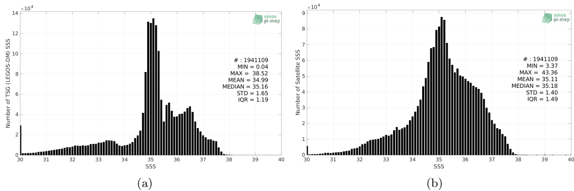
Figure 2: Histograms of SSS from TSG (LEGOS-DM) (a) and SMOS SSS L4 OI v342 - Weekly (CMEMS-CATDS-LOPS) (b) considering all match-up pairs per bins of 0.1 over the North Atlantic Ocean Pi-MEP region and for the full satellite product period.
