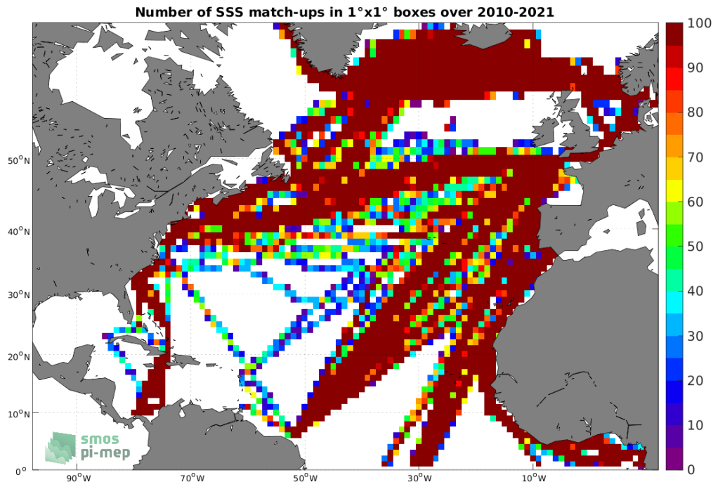
Figure 4: Number of SSS match-ups between TSG (LEGOS-DM) SSS and the SMOS SSS L4 OI v342 - Weekly (CMEMS-CATDS-LOPS) SSS product for the North Atlantic Ocean Pi-MEP region over 1^\circ \times 1^\circ boxes and for the full satellite product period.
