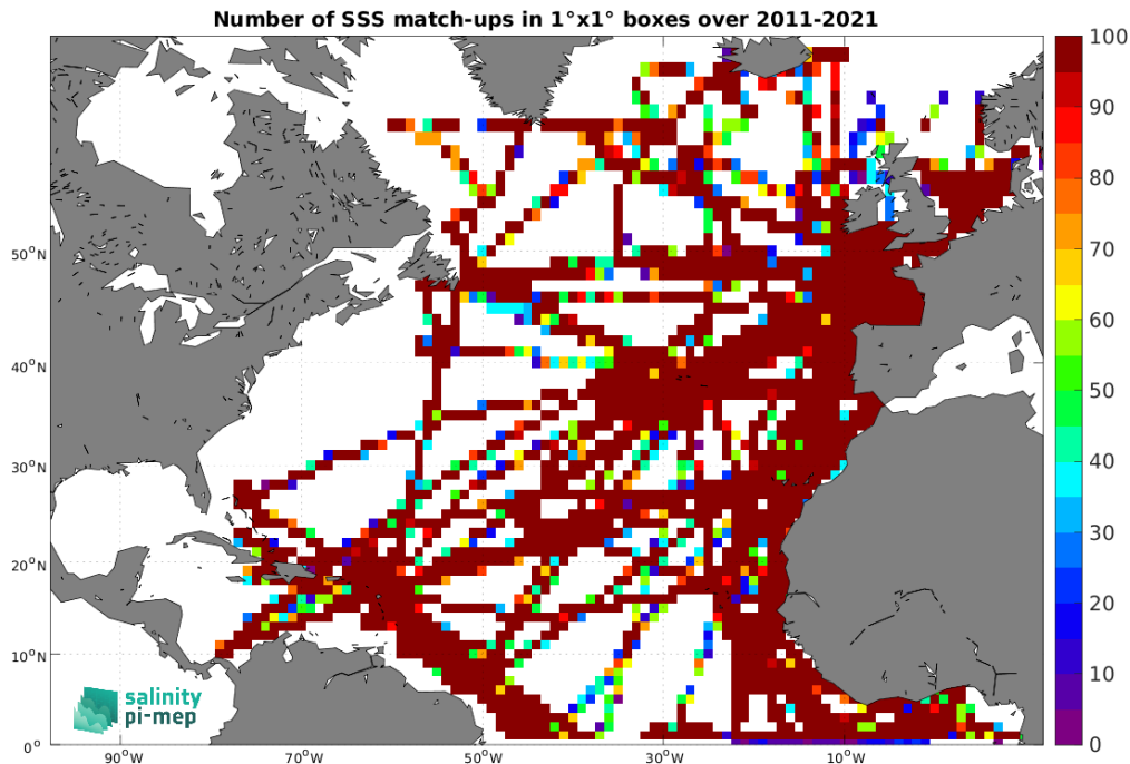
Figure 4: Number of SSS match-ups between TSG (GOSUD-Research-vessel) SSS and the SMOS SSS L4 OI v342 - Weekly (CMEMS-CATDS-LOPS) SSS product for the North Atlantic Ocean Pi-MEP region over 1°x1° boxes and for the full satellite product period.
