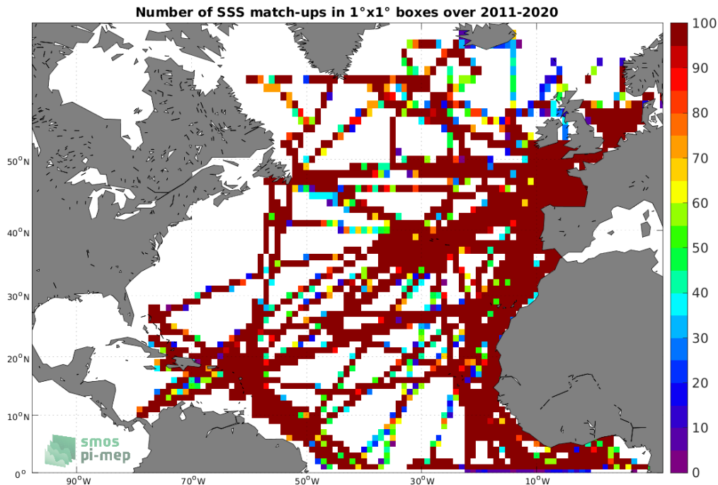
Figure 4: Number of SSS match-ups between TSG (GOSUD-Research-vessel) SSS and the SMOS SSS L4 OI v342 - Weekly (CMEMS-CATDS-LOPS) SSS product for the North Atlantic Ocean Pi-MEP region over 1^\circ \times 1^\circ boxes and for the full satellite product period.
