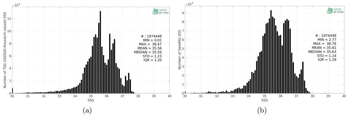
Figure 2: Histograms of SSS from TSG (GOSUD-Research-vessel) (a) and SMOS SSS L4 OI v342 - Weekly (CMEMS-CATDS-LOPS) (b) considering all match-up pairs per bins of 0.1 over the North Atlantic Ocean Pi-MEP region and for the full satellite product period.
