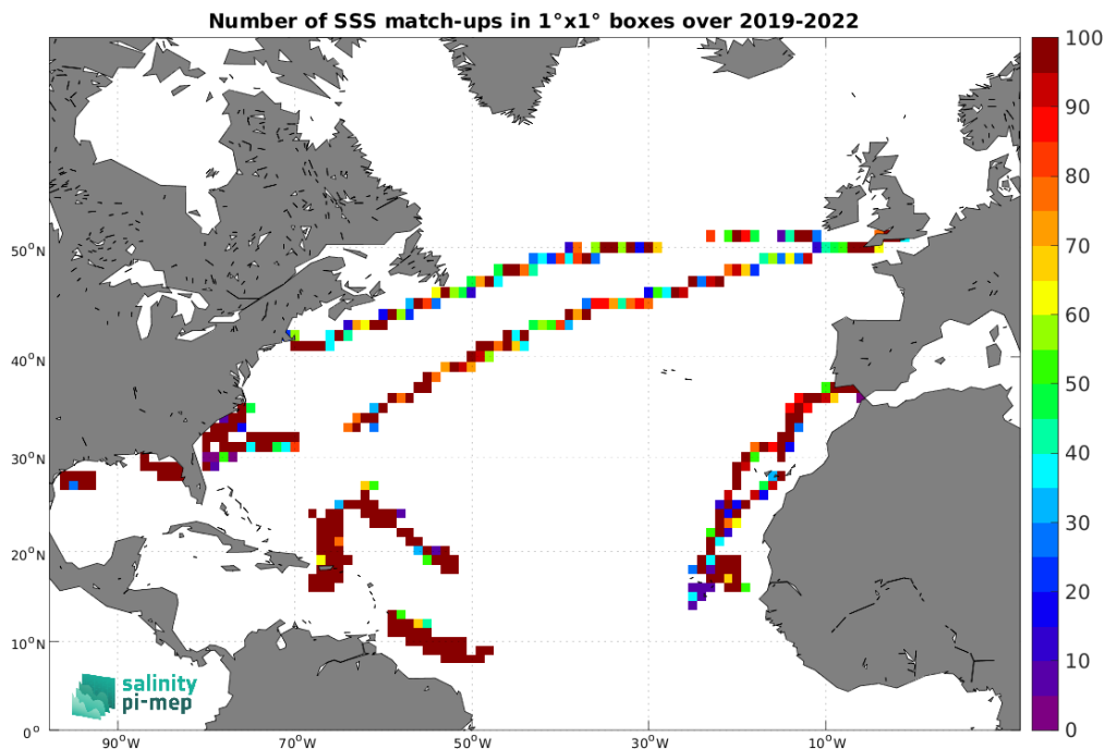
Figure 4: Number of SSS match-ups between Saildrone SSS and the SMOS SSS L4 OI v342 - Weekly (CMEMS-CATDS-LOPS) SSS product for the North Atlantic Ocean Pi-MEP region over 1°×1° boxes and for the full satellite product period.
