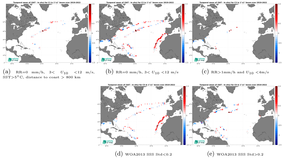
Figure 12: Temporal mean gridded over spatial boxes of size 1^\circ \times 1^\circ of \Delta\text{SSS} (SMOS SSS L4 OI v342 - Weekly (CMEMS-CATDS-LOPS) - Saildrone) for 5 different subdatasets corresponding to:RR=0 mm/h, 3 < U_{10} < 12 m/s, SST >5^\circ\text{C} , distance to coast > 800 km (a), RR=0 mm/h, 3 < U_{10} < 12 m/s (b), RR >1 mm/h and U_{10} < 4 m/s (c), WOA2013 SSS Std <0.2 (d), WOA2013 SSS Std >0.2 (e).
