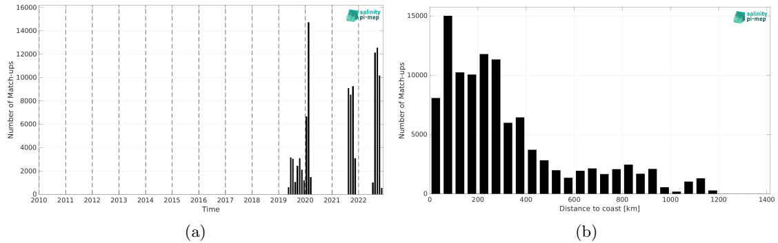
Figure 1: Number of match-ups between Sairdrone and SMOS SSS L4 OI v342 - Weekly (CMEMS-CATDS-LOPS) SSS as a function of time (a) and as function of the distance to coast (b) over the North Atlantic Ocean Pi-MEP region and for the full satellite product period.
