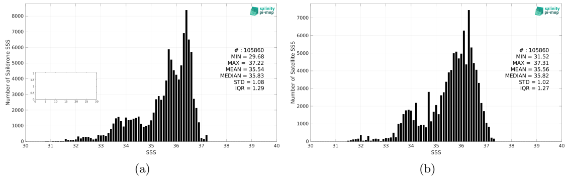
Figure 2: Histograms of SSS from Sairdrone (a) and SMOS SSS L4 OI v342 - Weekly (CMEMS-CATDS-LOPS) (b) considering all match-up pairs per bins of 0.1 over the North Atlantic Ocean Pi-MEP region and for the full satellite product period.
