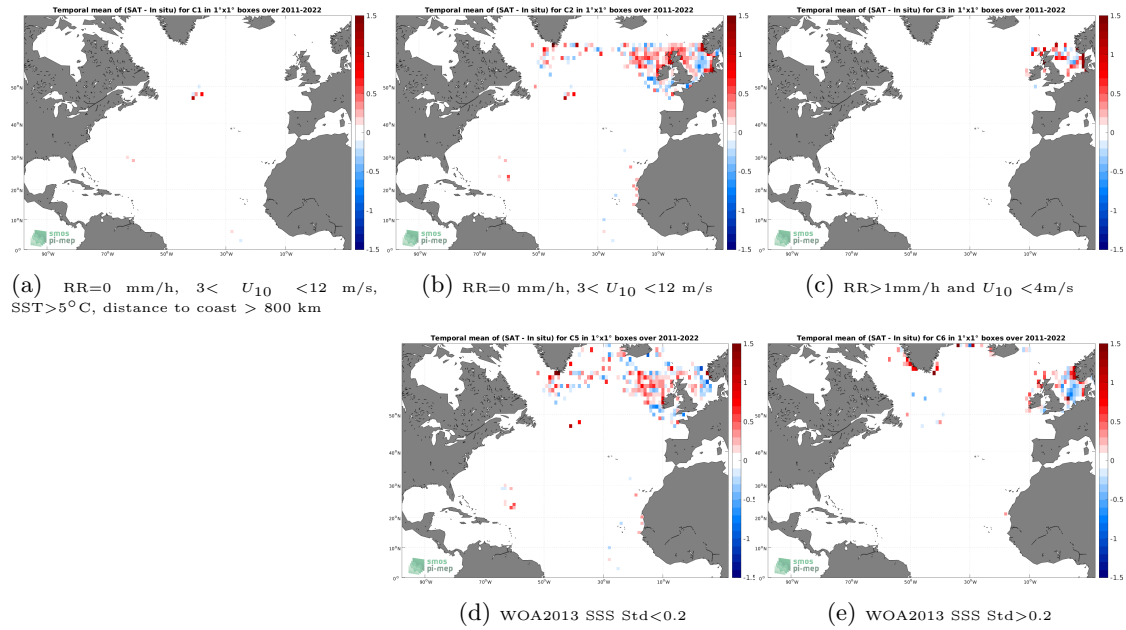
Figure 12: Temporal mean gridded over spatial boxes of size 1^\circ \times 1^\circ of \Delta SSS (SMOS SSS L4 OI v342 - Weekly (CMEMS-CATDS-LOPS) - ICES) for 5 different subdatasets corresponding to:RR=0 mm/h, 3 < U_{10} < 12 m/s, SST >5^\circ\text{C} , distance to coast > 800 km (a), RR=0 mm/h, 3 < U_{10} < 12 m/s (b), RR >1 mm/h and U_{10} < 4 m/s (c), WOA2013 SSS Std <0.2 (d), WOA2013 SSS Std >0.2 (e).
