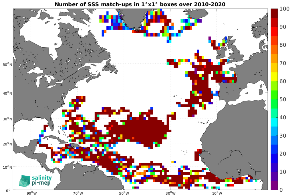
Figure 3: Number of SSS match-ups between Surface drifters SSS and the SMOS SSS L4 OI v342 - Weekly (CMEMS-CATDS-LOPS) SSS product for the North Atlantic Ocean Pi-MEP region over 1^\circ \times 1^\circ boxes and for the full satellite product period.
