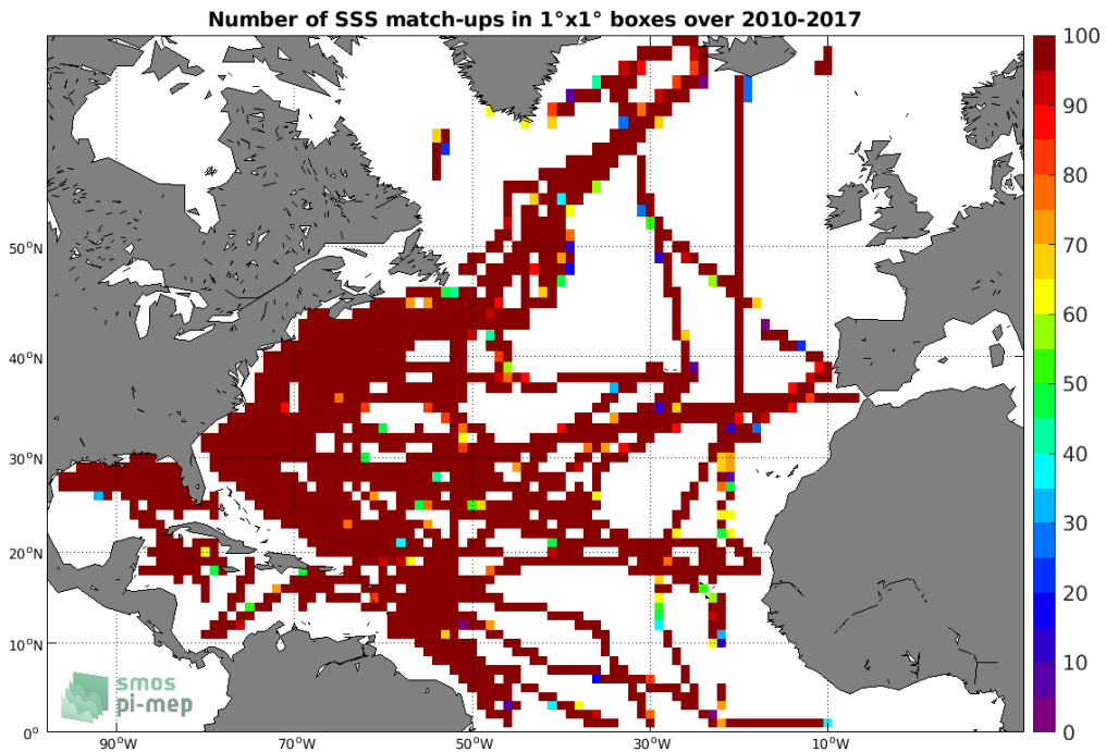
Figure 4: Number of SSS match-ups between TSG (SAMOS) SSS and the SMOS L4 v2 Weekly (CATDS-CECOS-IFREMER) SSS product for the North Atlantic Ocean Pi-MEP region over 1^{\circ} \times 1^{\circ} boxes and for the full satellite product period.
