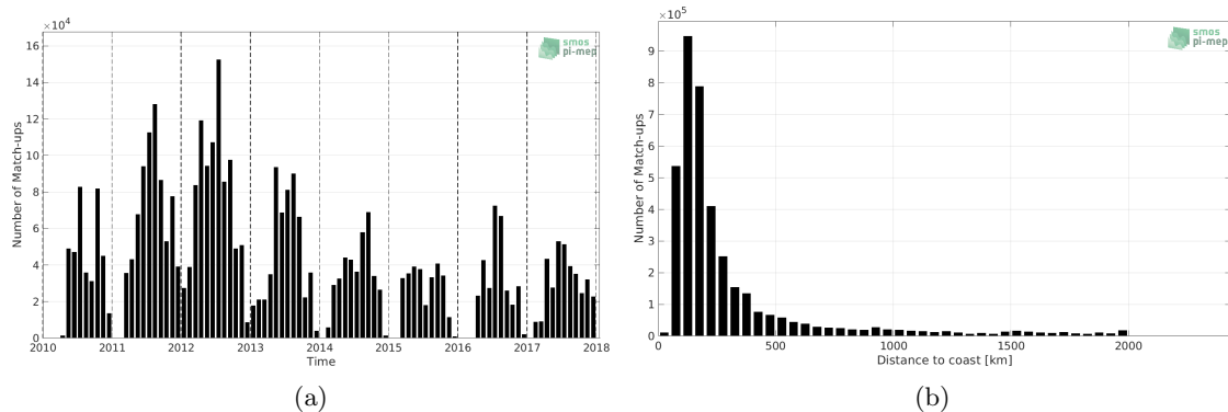
Figure 1: Number of match-ups between TSG (SAMOS) and SMOS L4 v2 Weekly (CATDS-CECOS-IFREMER) SSS as a function of time (a) and as function of the distance to coast (b) over the North Atlantic Ocean Pi-MEP region and for the full satellite product period.
