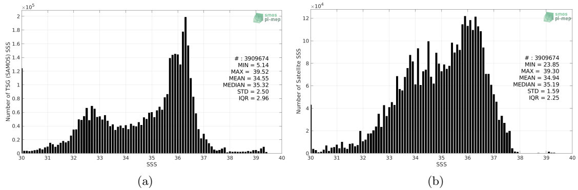
Figure 2: Histograms of SSS from TSG (SAMOS) (a) and SMOS L4 v2 Weekly (CATDS-CECOS-IFREMER) (b) considering all match-up pairs per bins of 0.1 over the North Atlantic Ocean Pi-MEP region and for the full satellite product period.
