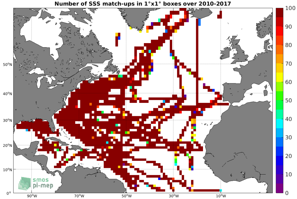
Figure 4: Number of SSS match-ups between TSG (SAMOS) SSS and the SMOS L4 v2 Weekly (CATDS-CECOS-IFREMER) SSS product for the North Atlantic Ocean Pi-MEP region over 1°x1° boxes and for the full satellite product period.
