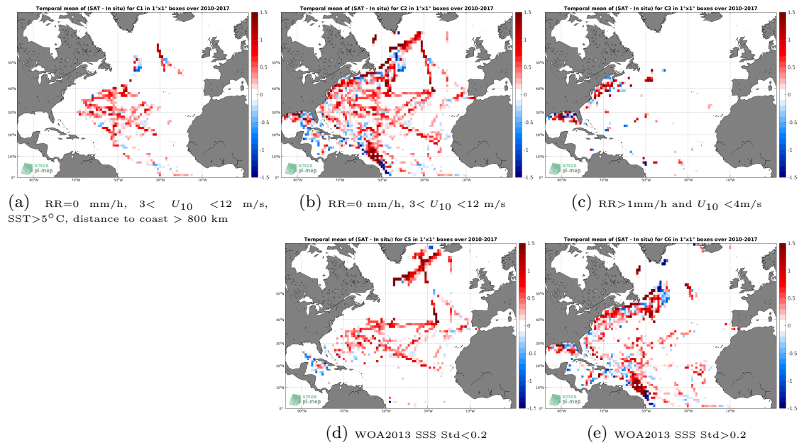
Figure 12: Temporal mean gridded over spatial boxes of size 1^\circ \times 1^\circ of \Delta SSS (SMOS L4 v2 Weekly (CATDS-CECOS-IFREMER) - TSG (SAMOS)) for 5 different subdatasets corresponding to: RR=0 mm/h, 3 < U_{10} < 12 m/s, SST > 5^\circ\text{C} , distance to coast > 800 km (a), RR=0 mm/h, 3 < U_{10} < 12 m/s (b), RR > 1 mm/h and U_{10} < 4 m/s (c), WOA2013 SSS Std < 0.2 (d), WOA2013 SSS Std > 0.2 (e).
