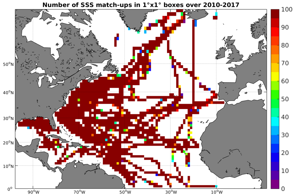
Figure 4: Number of SSS match-ups between TSG-SAMOS SSS and the SMOS-L4-CATDS-CECOS-IFREMER-V2-WEEKLY-0.5DEG SSS product for the North Atlantic Ocean Pi-MEP region over 1^\circ \times 1^\circ boxes and for the full satellite product period.
