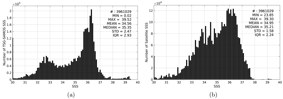
Figure 2: Histograms of SSS from TSG-SAMOS (a) and SMOS-L4-CATDS-CECOS-IFREMER-V2-WEEKLY-0.5DEG (b) considering all match-up pairs per bins of 0.1 over the North Atlantic Ocean Pi-MEP region and for the full satellite product period.
