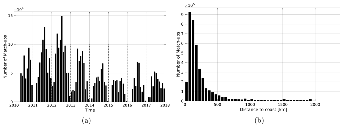
Figure 1: Number of match-ups between TSG-SAMOS and SMOS-L4-CATDS-CECOS-IFREMER-V2-WEEKLY-0.5DEG SSS as a function of time (a) and as function of the distance to coast (b) over the North Atlantic Ocean Pi-MEP region and for the full satellite product period.
