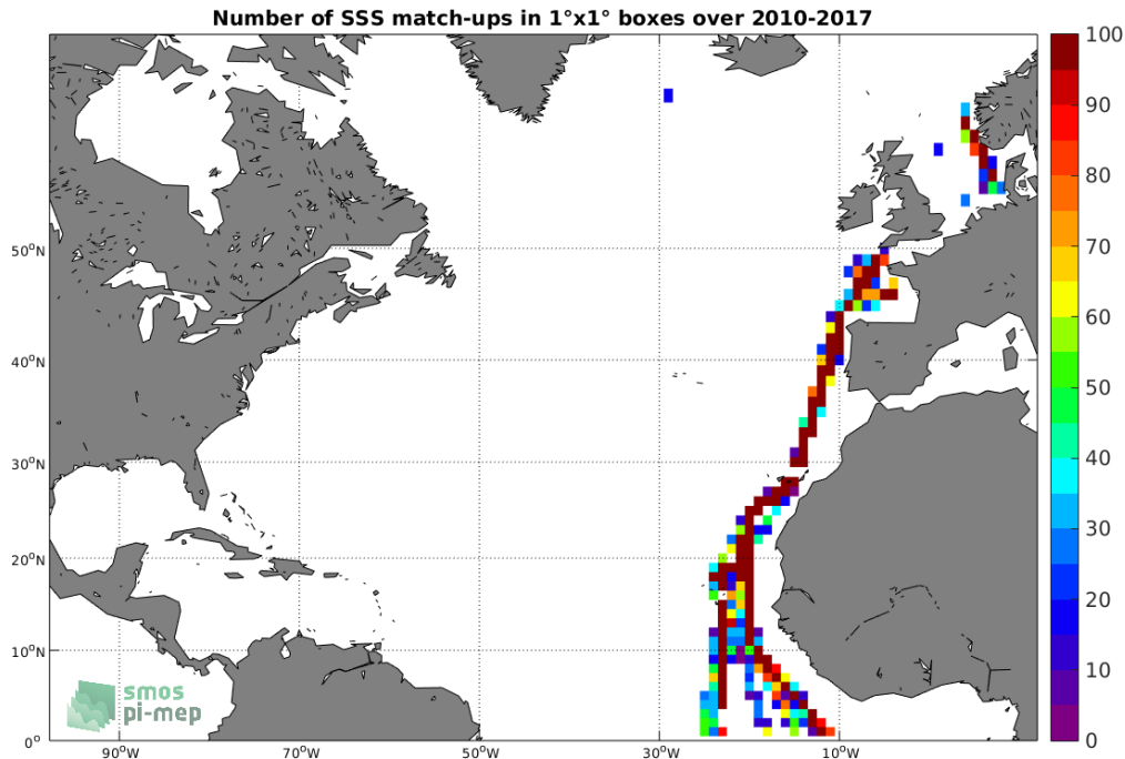
Figure 4: Number of SSS match-ups between TSG-POLARSTERN SSS and the SMOS-L4-CATDS-CECOS-IFREMER-V2-WEEKLY-0.5DEG SSS product for the North Atlantic Ocean Pi-MEP region over 1^{\circ} \times 1^{\circ} boxes and for the full satellite product period.
