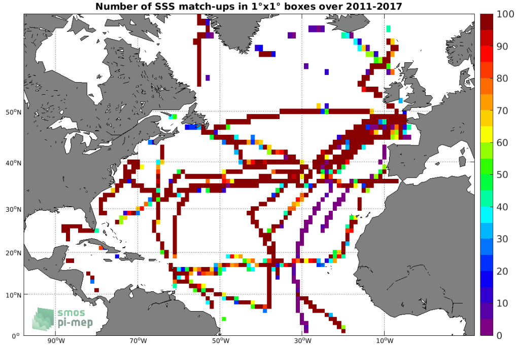
Figure 4: Number of SSS match-ups between TSG (GOSUD-Sailing-ship) SSS and the SMOS L4 v2 Weekly (CATDS-CECOS-IFREMER) SSS product for the North Atlantic Ocean Pi-MEP region over 1°x1° boxes and for the full satellite product period.
