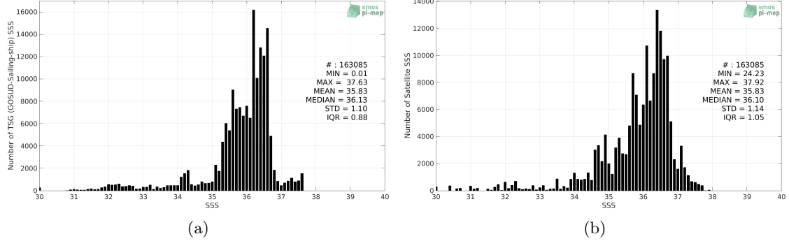
Figure 2: Histograms of SSS from TSG (GOSUD-Sailing-ship) (a) and SMOS L4 v2 Weekly (CATDS-CECOS-IFREMER) (b) considering all match-up pairs per bins of 0.1 over the North Atlantic Ocean Pi-MEP region and for the full satellite product period.
