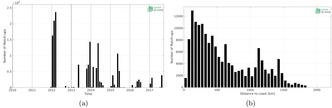
Figure 1: Number of match-ups between TSG (GOSUD-Sailing-ship) and SMOS L4 v2 Weekly (CATDS-CECOS-IFREMER) SSS as a function of time (a) and as function of the distance to coast (b) over the North Atlantic Ocean Pi-MEP region and for the full satellite product period.
