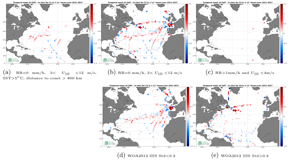
Figure 12: Temporal mean gridded over spatial boxes of size 1^\circ \times 1^\circ of \Delta SSS (SMOS L4 v2 Weekly (CATDS-CECOS-IFREMER) - TSG (GOSUD-Sailing-ship)) for 5 different subdatasets corresponding to: RR=0 mm/h, 3 < U_{10} < 12 m/s, SST > 5^\circ C , distance to coast > 800 km (a), RR=0 mm/h, 3 < U_{10} < 12 m/s (b), RR > 1 mm/h and U_{10} < 4 m/s (c), WOA2013 SSS Std < 0.2 (d), WOA2013 SSS Std > 0.2 (e).
