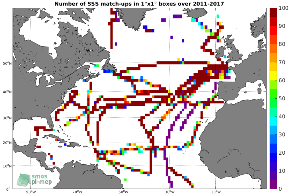
Figure 4: Number of SSS match-ups between TSG-GOSUD-Sailing-ship SSS and the SMOS-L4-CATDS-CECOS-IFREMER-V2-WEEKLY-0.5DEG SSS product for the North Atlantic Ocean Pi-MEP region over 1^\circ \times 1^\circ boxes and for the full satellite product period.
