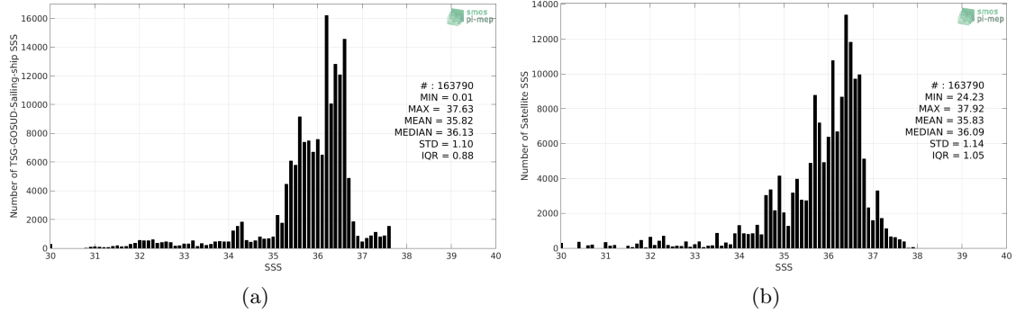
Figure 2: Histograms of SSS from TSG-GOSUD-Sailing-ship (a) and SMOS-L4-CATDS-CECOS-IFREMER-V2-WEEKLY-0.5DEG (b) considering all match-up pairs per bins of 0.1 over the North Atlantic Ocean Pi-MEP region and for the full satellite product period.
