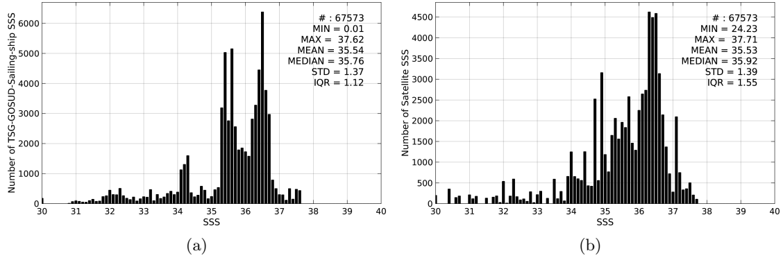
Figure 2: Histograms of SSS from TSG-GOSUD-Sailing-ship (a) and SMOS-L4-CATDS-CECOS-IFREMER-V2-WEEKLY-0.5DEG (b) considering all match-up pairs per bins of 0.1 over the North Atlantic Ocean Pi-MEP region and for the full satellite product period.
