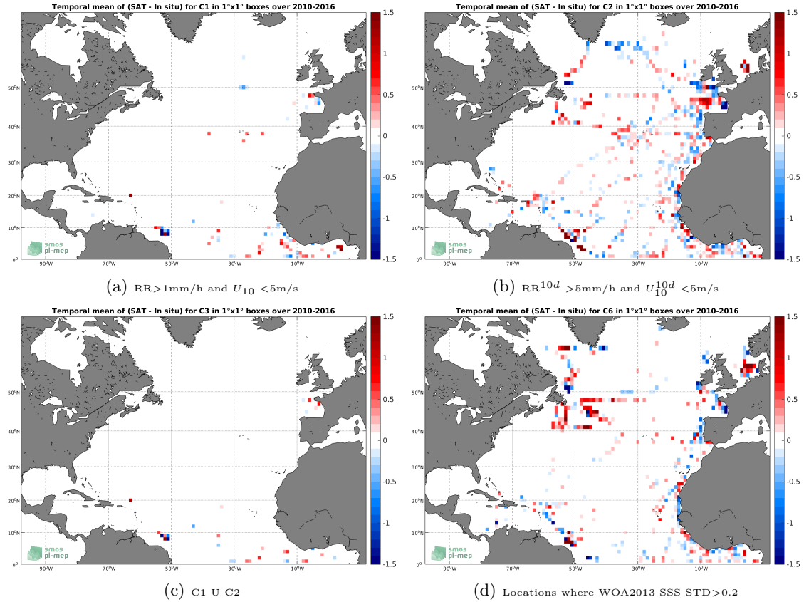
Figure 12: Temporal mean gridded over spatial boxes of size 1^\circ \times 1^\circ of \Delta SSS (SMOS-L4-CATDS-CECOS-IFREMER-V2-WEEKLY-0.5DEG - TSG-GOSUD-Research-vessel) for 4 different sub-datasets corresponding to: RR > 1mm/h and U_{10} < 5\text{m/s} (a), RR^{10d} > 5\text{mm/h} and U_{10}^{10d} < 5\text{m/s} (b), C1 U C2 (c), Locations where WOA2013 SSS STD > 0.2 (d).
