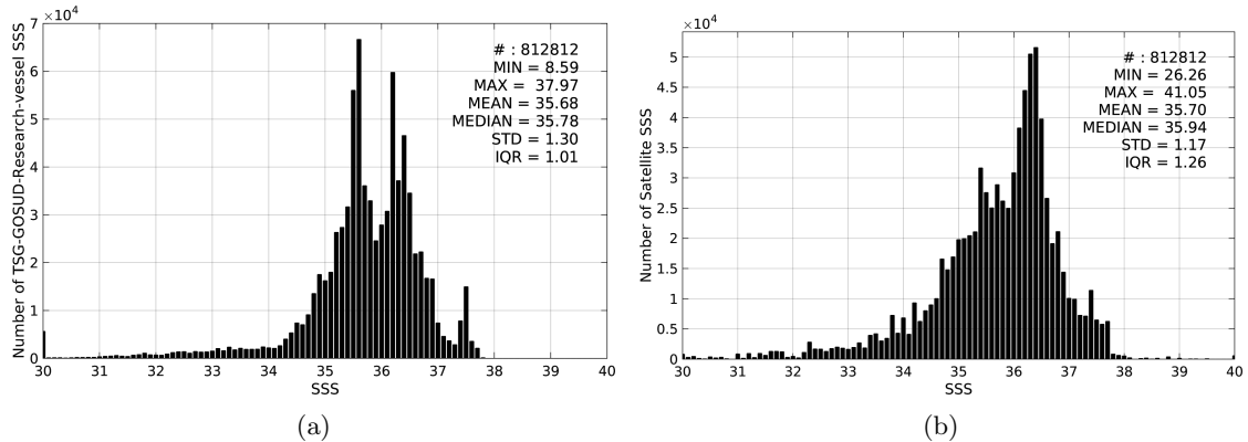
Figure 2: Histograms of SSS from TSG-GOSUD-Research-vessel (a) and SMOS-L4-CATDS-CECOS-IFREMER-V2-WEEKLY-0.5DEG (b) considering all match-up pairs per bins of 0.1 over the North Atlantic Ocean Pi-MEP region and for the full satellite product period.
