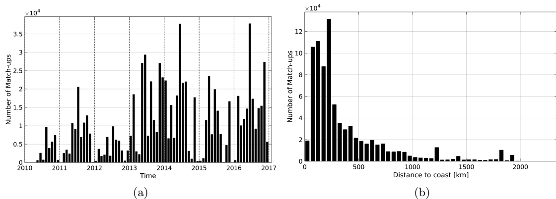
Figure 1: Number of match-ups between TSG-GOSUD-Research-vessel and SMOS-L4-CATDS-CECOS-IFREMER-V2-WEEKLY-0.5DEG SSS as a function of time (a) and as function of the distance to coast (b) over the North Atlantic Ocean Pi-MEP region and for the full satellite product period.
