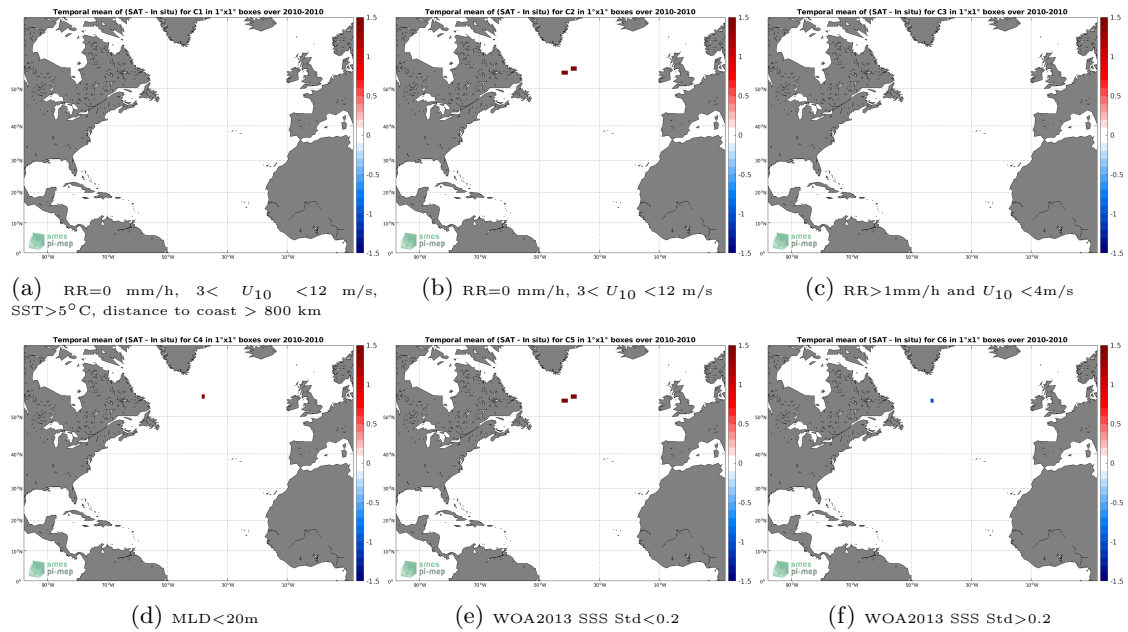
Figure 12: Temporal mean gridded over spatial boxes of size 1^{\circ}\times 1^{\circ} of \Delta\text{SSS} (SMOS L4 v2 Weekly (CATDS-CECOS-IFREMER) - Sea mammals) for 6 different subdatasets corresponding to:RR=0 mm/h, 3 < U_{10} < 12 m/s, SST >5^{\circ}\text{C} , distance to coast > 800 km (a), RR=0 mm/h, 3 < U_{10} < 12 m/s (b), RR >1\text{mm/h} and U_{10} < 4\text{m/s} (c),MLD <20\text{m} (d),WOA2013 SSS Std <0.2 (e),WOA2013 SSS Std >0.2 (f).
