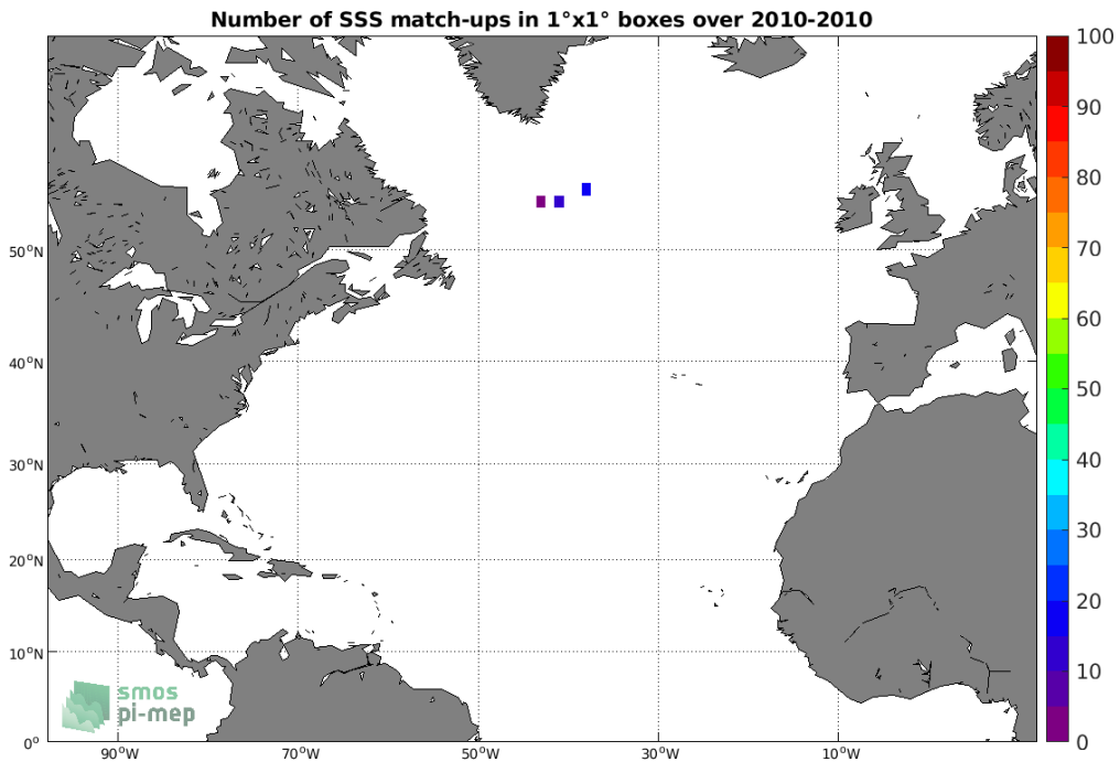
Figure 4: Number of SSS match-ups between Sea mammals SSS and the SMOS L4 v2 Weekly (CATDS-CECOS-IFREMER) SSS product for the North Atlantic Ocean Pi-MEP region over 1^\circ \times 1^\circ boxes and for the full satellite product period.
