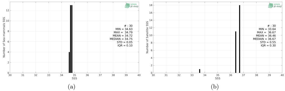
Figure 2: Histograms of SSS from Sea mammals (a) and SMOS L4 v2 Weekly (CATDS-CECOS-IFREMER) (b) considering all match-up pairs per bins of 0.1 over the North Atlantic Ocean Pi-MEP region and for the full satellite product period.
