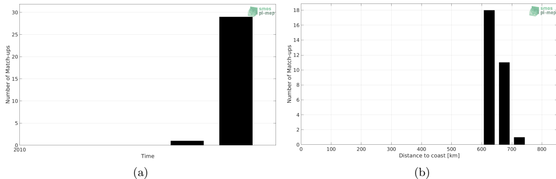
Figure 1: Number of match-ups between Sea mammals and SMOS L4 v2 Weekly (CATDS-CECOS-IFREMER) SSS as a function of time (a) and as function of the distance to coast (b) over the North Atlantic Ocean Pi-MEP region and for the full satellite product period.
