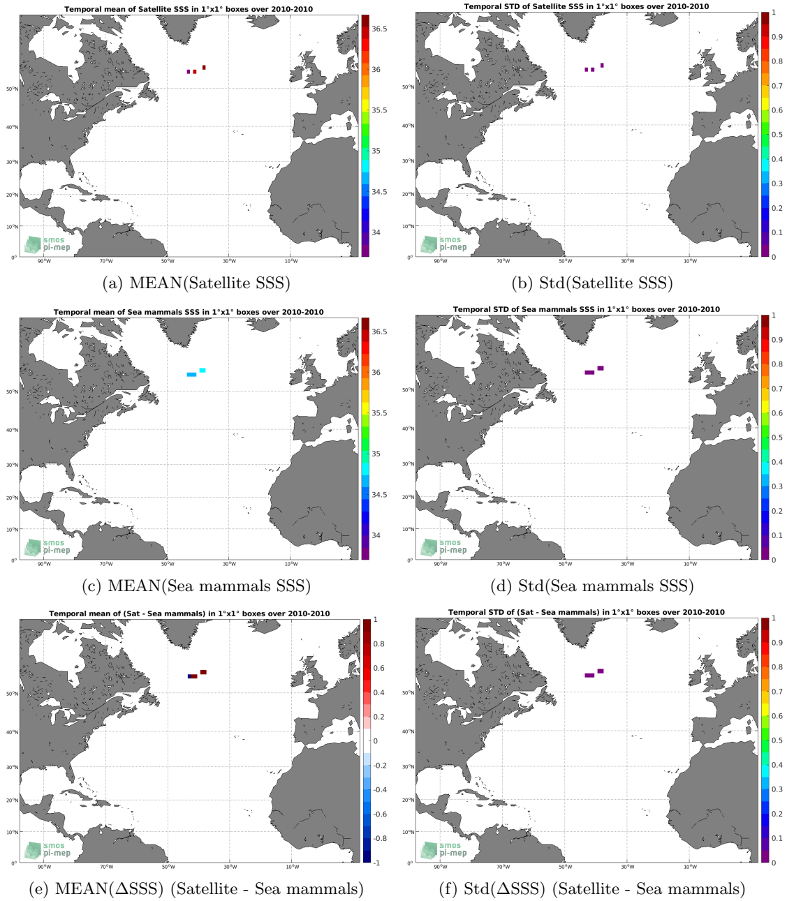
Figure 6: Temporal mean (left) and Std (right) of SSS from SMOS L4 v2 Weekly (CATDS-CECOS-IFREMER) (top), Sea mammals (middle), and of \Delta SSS (Satellite - Sea mammals). Only match-up pairs are used to generate these maps.
