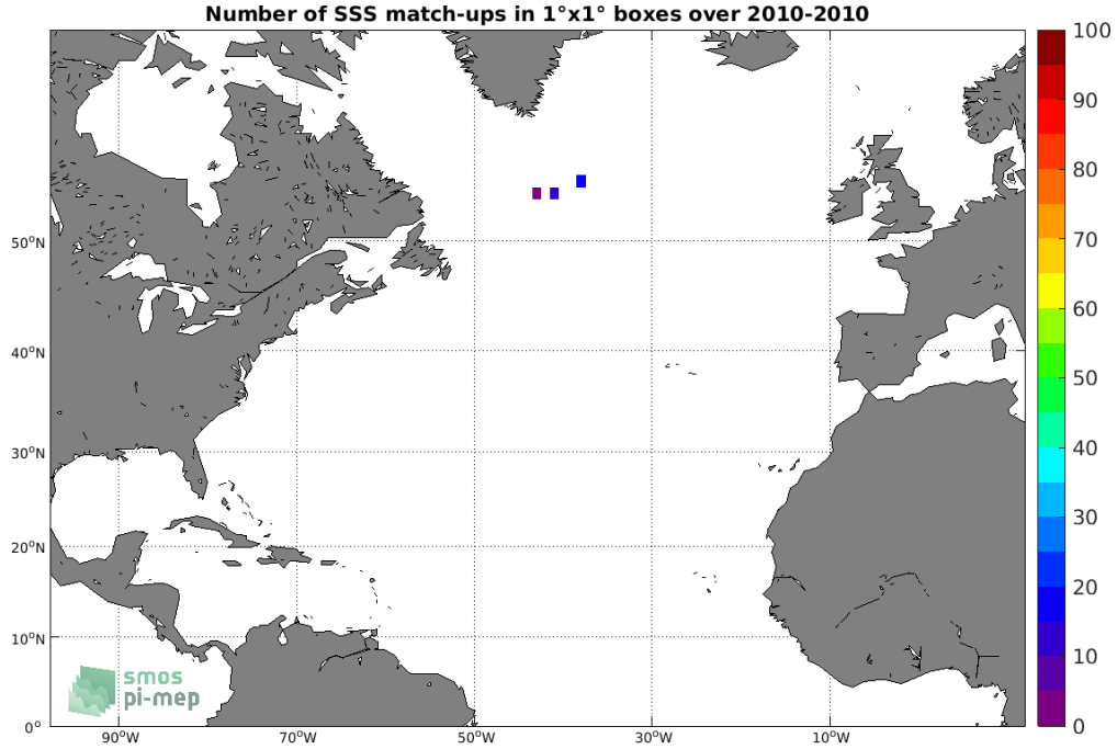
Figure 4: Number of SSS match-ups between Sea mammals SSS and the SMOS L4 v2 Weekly (CATDS-CECOS-IFREMER) SSS product for the North Atlantic Ocean Pi-MEP region over 1°x1° boxes and for the full satellite product period.
