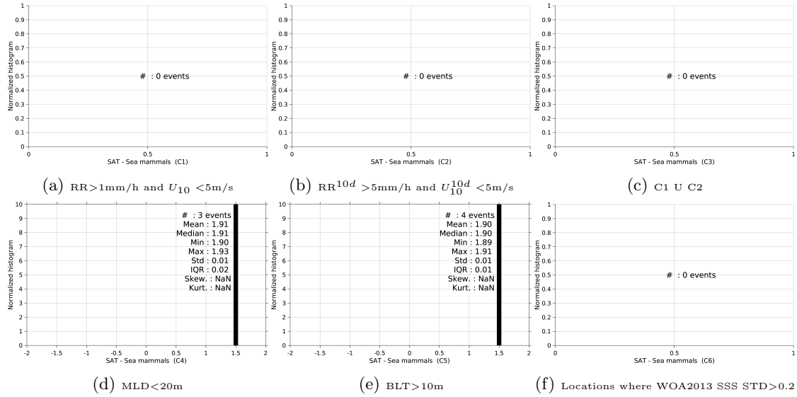
Figure 13: Normalized histogram of \Delta SSS (SMOS-L4-CATDS-CECOS-IFREMER-V2-WEEKLY-0.5DEG - Sea mammals) for 6 different subdatasets corresponding to: RR>1mm/h and U_{10} <5m/s (a), RR^{10d} >5mm/h and U_{10}^{10d} <5m/s (b), C1 U C2 (c),MLD<20m (d),BLT>10m (e),Locations where WOA2013 SSS STD>0.2 (f).
