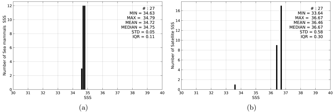
Figure 2: Histograms of SSS from Sea mammals (a) and SMOS-L4-CATDS-CECOS-IFREMER-V2-WEEKLY-0.5DEG (b) considering all match-up pairs per bins of 0.1 over the North Atlantic Ocean Pi-MEP region and for the full satellite product period.
