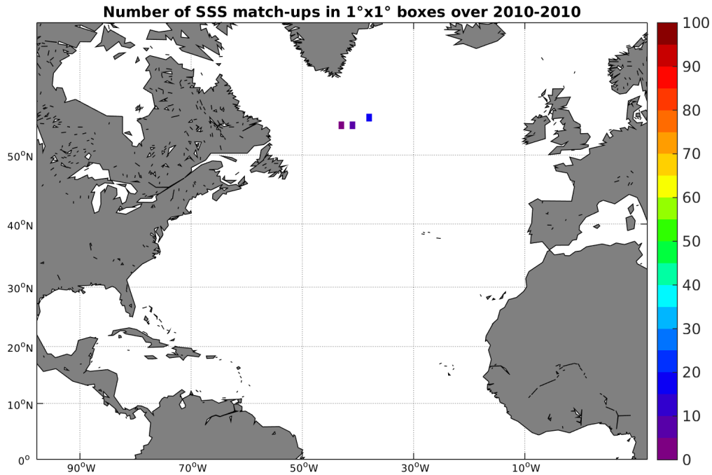
Figure 4: Number of SSS match-ups between Sea mammals SSS and the SMOS-L4-CATDS-CECOS-IFREMER-V2-WEEKLY-0.5DEG SSS product for the North Atlantic Ocean Pi-MEP region over 1^\circ \times 1^\circ boxes and for the full satellite product period.
