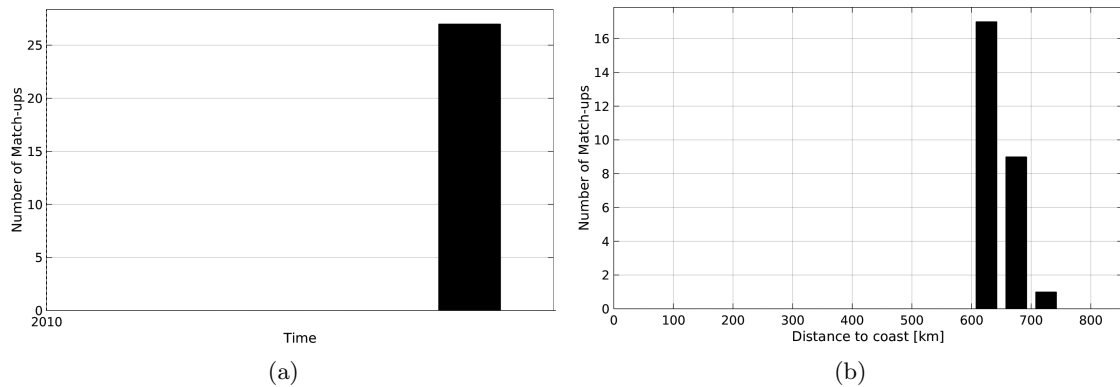
Figure 1: Number of match-ups between Sea mammals and SMOS-L4-CATDS-CECOS-IFREMER-V2-WEEKLY-0.5DEG SSS as a function of time (a) and as function of the distance to coast (b) over the North Atlantic Ocean Pi-MEP region and for the full satellite product period.
