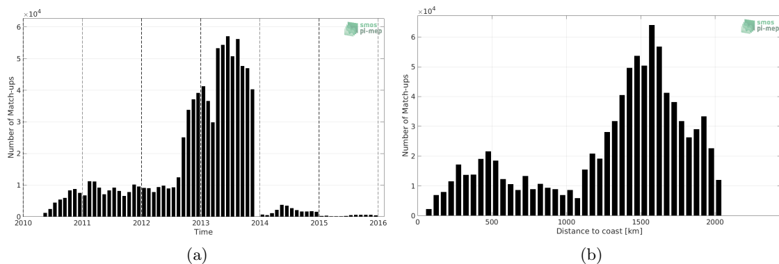
Figure 1: Number of match-ups between Surface drifters and SMOS L4 v2 Weekly (CATDS-CECOS-IFREMER) SSS as a function of time (a) and as function of the distance to coast (b) over the North Atlantic Ocean Pi-MEP region and for the full satellite product period.
