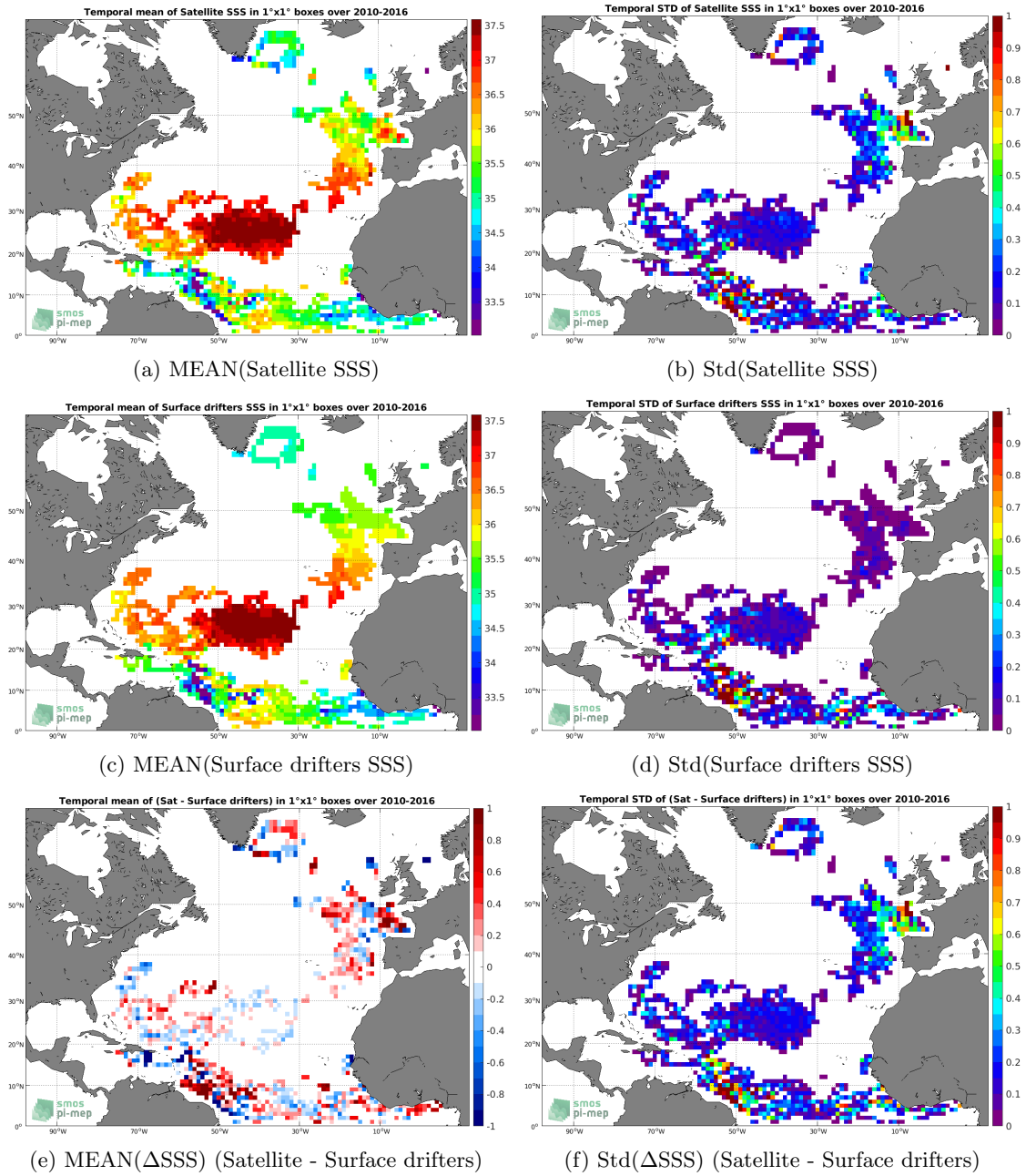
Figure 5: Temporal mean (left) and Std (right) of SSS from SMOS L4 v2 Weekly (CATDS-CECOS-IFREMER) (top), Surface drifters (middle), and of \Delta SSS (Satellite - Surface drifters). Only match-up pairs are used to generate these maps.
