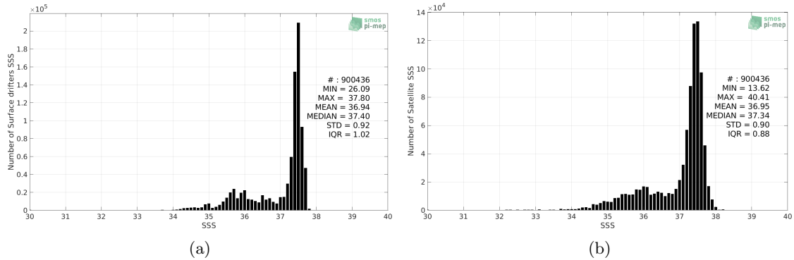
Figure 2: Histograms of SSS from Surface drifters (a) and SMOS L4 v2 Weekly (CATDS-CECOS-IFREMER) (b) considering all match-up pairs per bins of 0.1 over the North Atlantic Ocean Pi-MEP region and for the full satellite product period.
