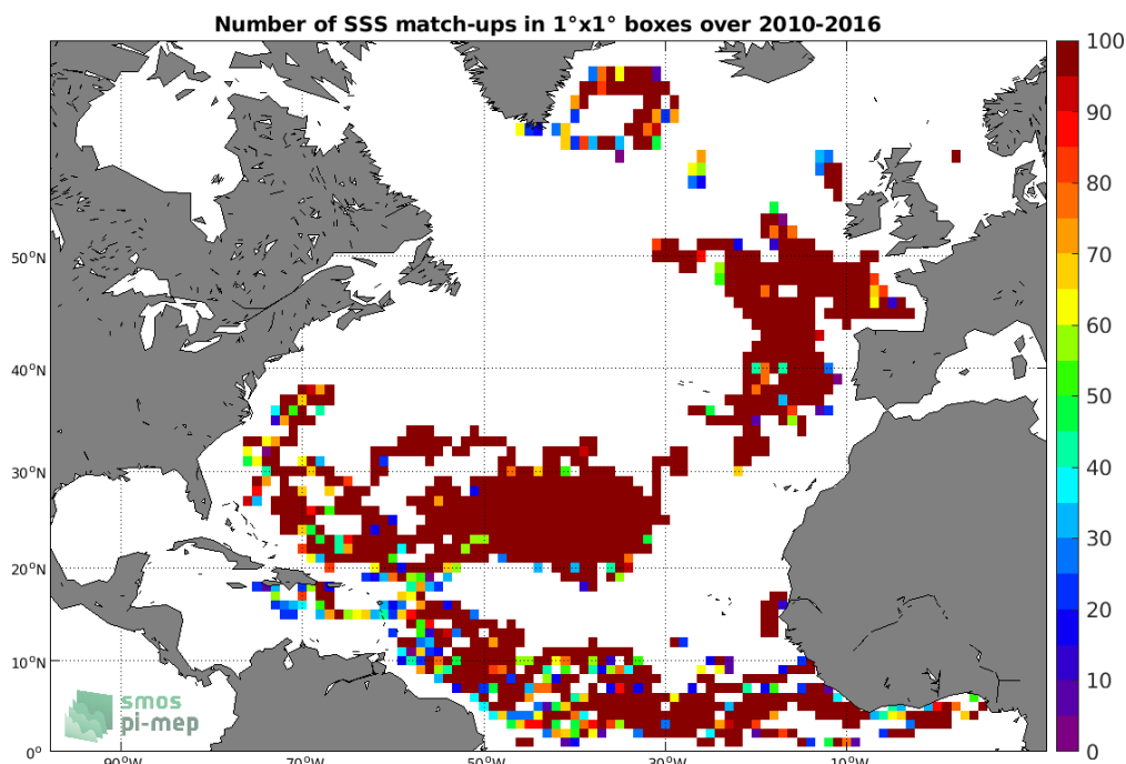
Figure 3: Number of SSS match-ups between Surface drifters SSS and the SMOS L4 v2 Weekly (CATDS-CECOS-IFREMER) SSS product for the North Atlantic Ocean Pi-MEP region over 1^\circ \times 1^\circ boxes and for the full satellite product period.
