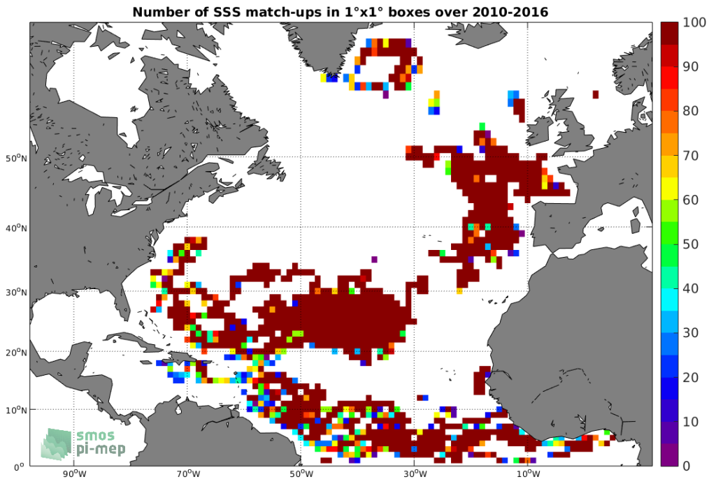
Figure 3: Number of SSS match-ups between Surface drifters SSS and the SMOS-L4-CATDS-CECOS-IFREMER-V2-WEEKLY-0.5DEG SSS product for the North Atlantic Ocean Pi-MEP region over 1^\circ \times 1^\circ boxes and for the full satellite product period.
