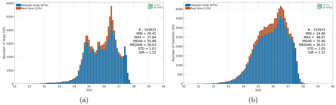
Figure 2: Histograms of SSS from Argo (a) and SMOS L4 v2 Weekly (CATDS-CECOS-IFREMER) (b) considering all match-up pairs per bins of 0.1 over the North Atlantic Ocean Pi-MEP region and for the full satellite product period.
