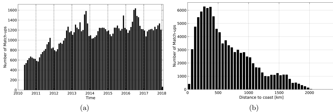
Figure 1: Number of match-ups between Argo and SMOS-L4-CATDS-CECOS-IFREMER-V2-WEEKLY-0.5DEG SSS as a function of time (a) and as function of the distance to coast (b) over the North Atlantic Ocean Pi-MEP region and for the full satellite product period.
