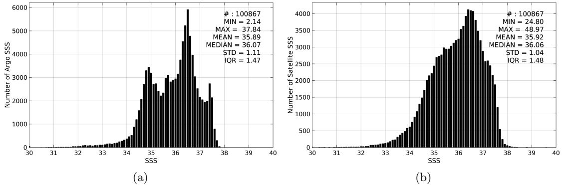
Figure 2: Histograms of SSS from Argo (a) and SMOS-L4-CATDS-CECOS-IFREMER-V2-WEEKLY-0.5DEG (b) considering all match-up pairs per bins of 0.1 over the North Atlantic Ocean Pi-MEP region and for the full satellite product period.
