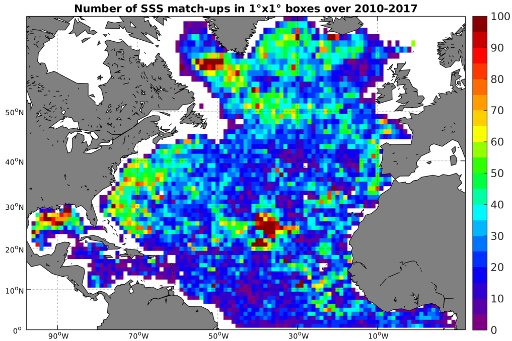
Figure 4: Number of SSS match-ups between Argo SSS and the SMOS-L4-CATDS-CECOS-IFREMER-V2-WEEKLY-0.5DEG SSS product for the North Atlantic Ocean Pi-MEP region over 1^\circ \times 1^\circ boxes and for the full satellite product period.
