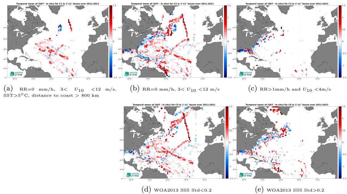
Figure 12: Temporal mean gridded over spatial boxes of size 1^\circ \times 1^\circ of \Delta\text{SSS} (SMOS SSS L4 v2 - Daily (BEC) - TSG (SAMOS)) for 5 different subdatasets corresponding to:RR=0 mm/h, 3 < U_{10} < 12 m/s, SST >5^\circ\text{C} , distance to coast > 800 km (a), RR=0 mm/h, 3 < U_{10} < 12 m/s (b), RR >1 mm/h and U_{10} < 4 m/s (c), WOA2013 SSS Std <0.2 (d), WOA2013 SSS Std >0.2 (e).
