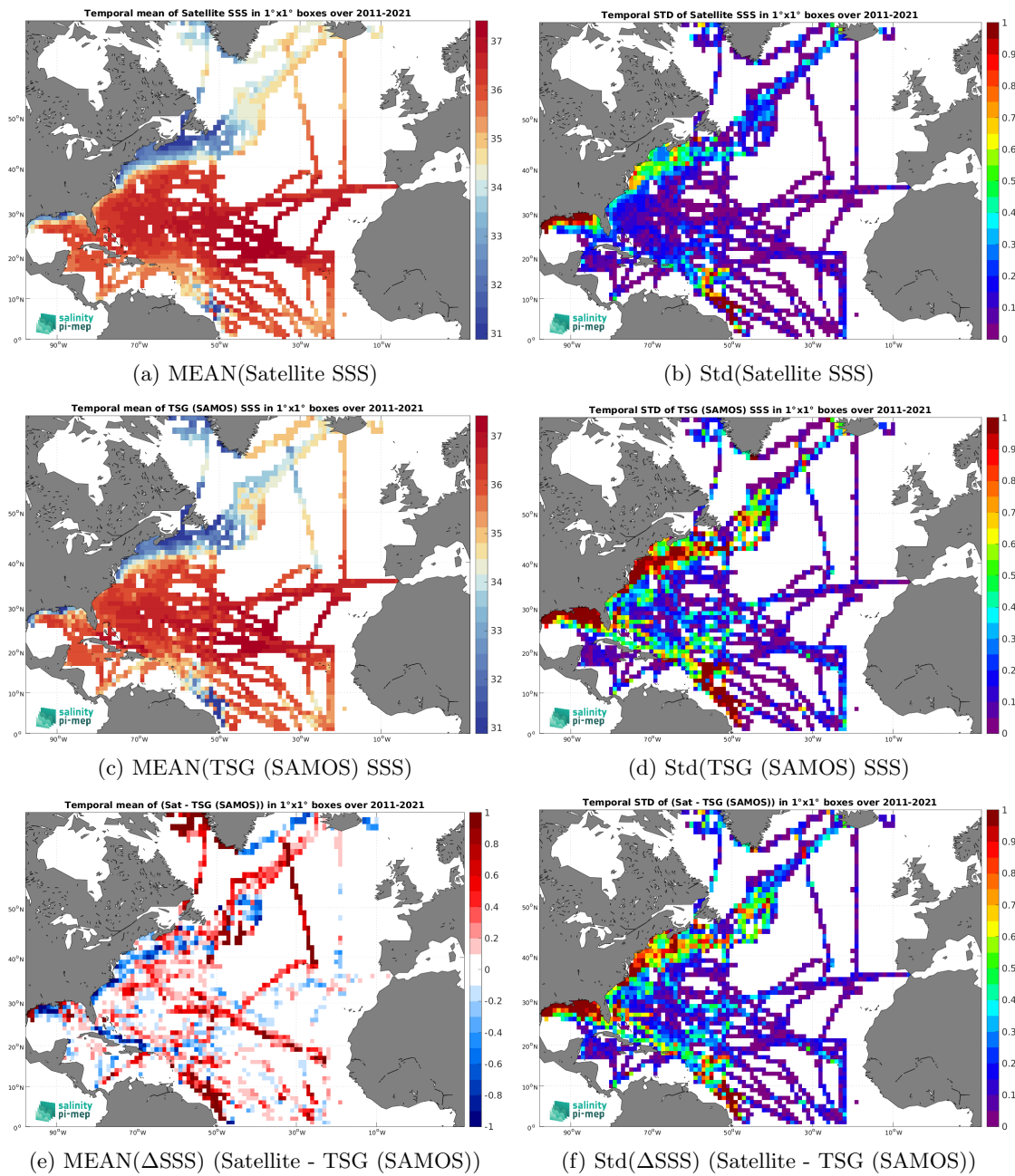
Figure 6: Temporal mean (left) and Std (right) of SSS from SMOS SSS L4 v2 - Daily (BEC) (top), TSG (SAMOS) (middle), and of \Delta SSS (Satellite - TSG (SAMOS)). Only match-up pairs are used to generate these maps.
