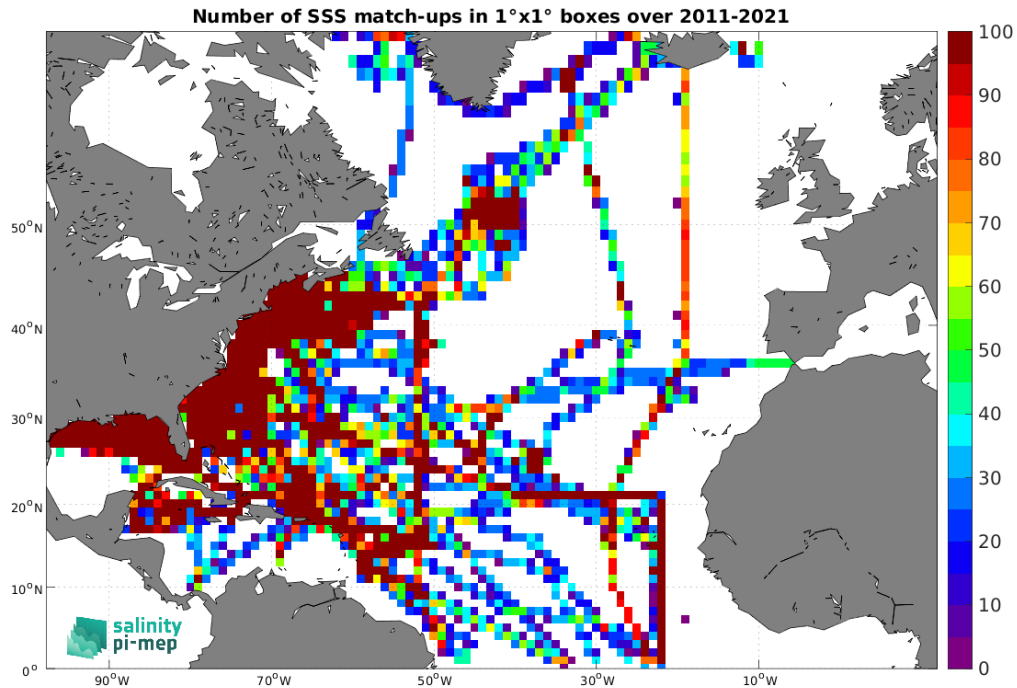
Figure 4: Number of SSS match-ups between TSG (SAMOS) SSS and the SMOS SSS L4 v2 - Daily (BEC) SSS product for the North Atlantic Ocean Pi-MEP region over 1^\circ \times 1^\circ boxes and for the full satellite product period.
