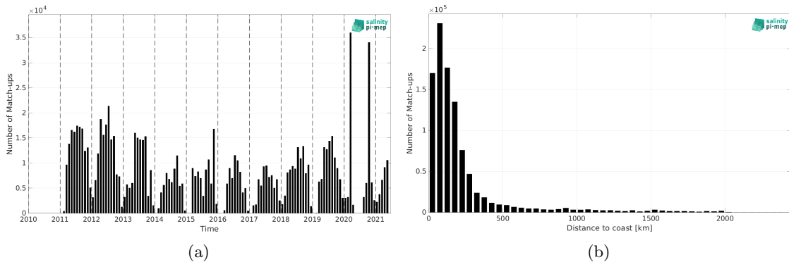
Figure 1: Number of match-ups between TSG (SAMOS) and SMOS SSS L4 v2 - Daily (BEC) SSS as a function of time (a) and as function of the distance to coast (b) over the North Atlantic Ocean Pi-MEP region and for the full satellite product period.
