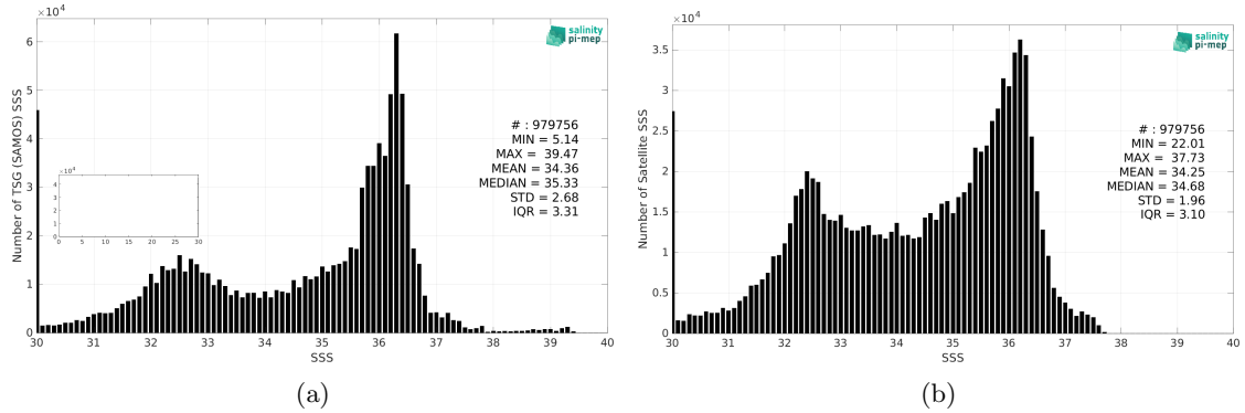
Figure 2: Histograms of SSS from TSG (SAMOS) (a) and SMOS SSS L4 v2 - Daily (BEC) (b) considering all match-up pairs per bins of 0.1 over the North Atlantic Ocean Pi-MEP region and for the full satellite product period.
