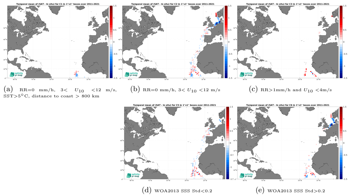
Figure 14: Temporal mean gridded over spatial boxes of size 1^\circ \times 1^\circ of \Delta\text{SSS} (SMOS SSS L4 v2 - Daily (BEC) - TSG (Polarstern)) for 5 different subdatasets corresponding to:RR=0 mm/h, 3 < U_{10} < 12 m/s, SST >5^\circ\text{C} , distance to coast > 800 km (a), RR=0 mm/h, 3 < U_{10} < 12 m/s (b), RR >1 mm/h and U_{10} < 4 m/s (c), WOA2013 SSS Std <0.2 (d), WOA2013 SSS Std >0.2 (e).
