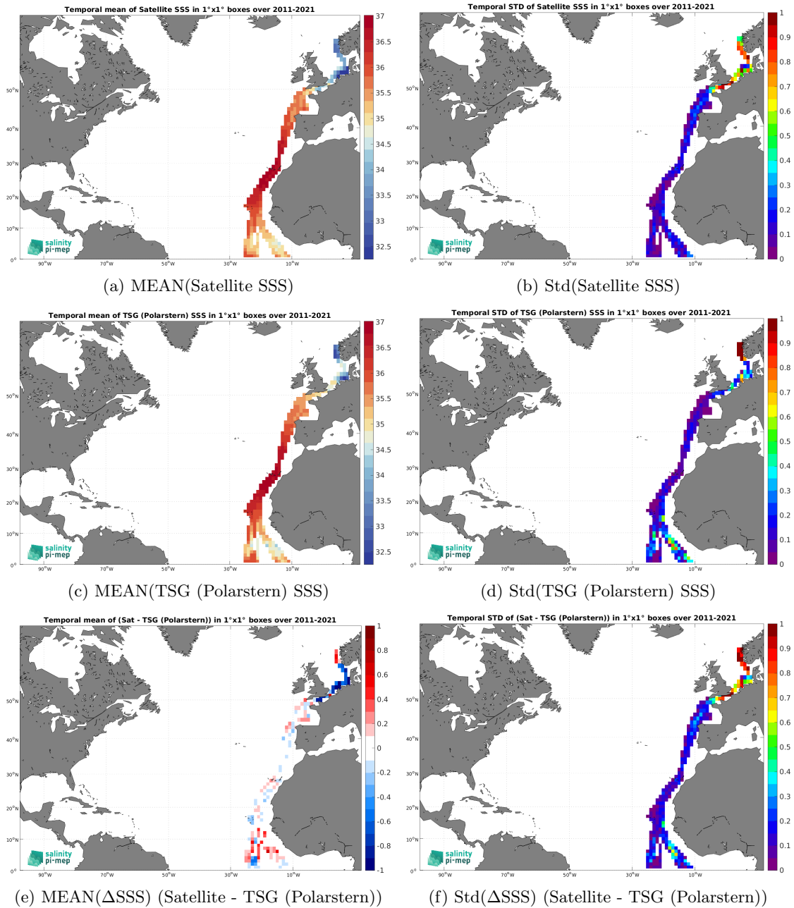
Figure 7: Temporal mean (left) and Std (right) of SSS from SMOS SSS L4 v2 - Daily (BEC) (top), TSG (Polarstern) (middle), and of \Delta SSS (Satellite - TSG (Polarstern)). Only match-up pairs are used to generate these maps.
