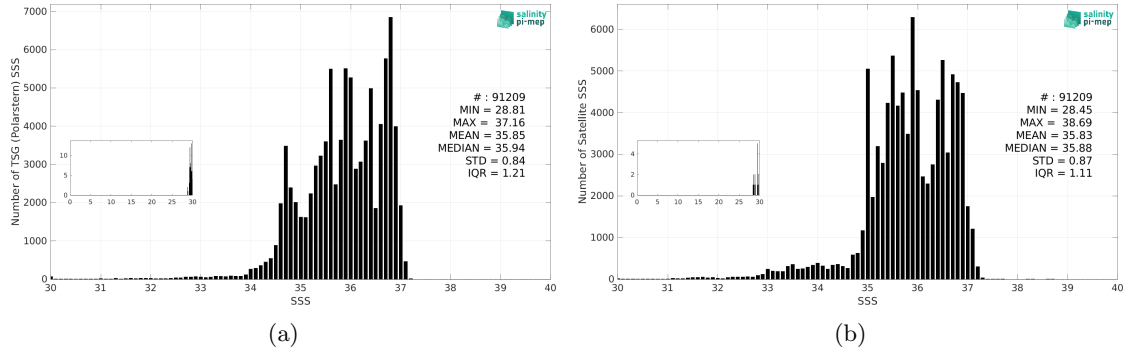
Figure 3: Histograms of SSS from TSG (Polarstern) (a) and SMOS SSS L4 v2 - Daily (BEC) (b) considering all match-up pairs per bins of 0.1 over the North Atlantic Ocean Pi-MEP region and for the full satellite product period.
