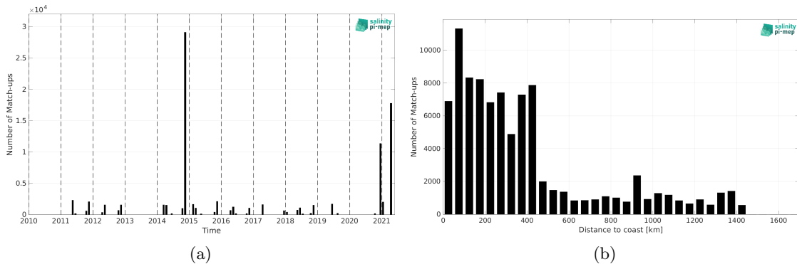
Figure 2: Number of match-ups between TSG (Polarstern) and SMOS SSS L4 v2 - Daily (BEC) SSS as a function of time (a) and as function of the distance to coast (b) over the North Atlantic Ocean Pi-MEP region and for the full satellite product period.
