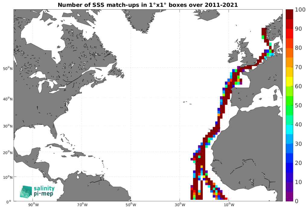
Figure 5: Number of SSS match-ups between TSG (Polarstern) SSS and the SMOS SSS L4 v2 - Daily (BEC) SSS product for the North Atlantic Ocean Pi-MEP region over 1^\circ \times 1^\circ boxes and for the full satellite product period.
