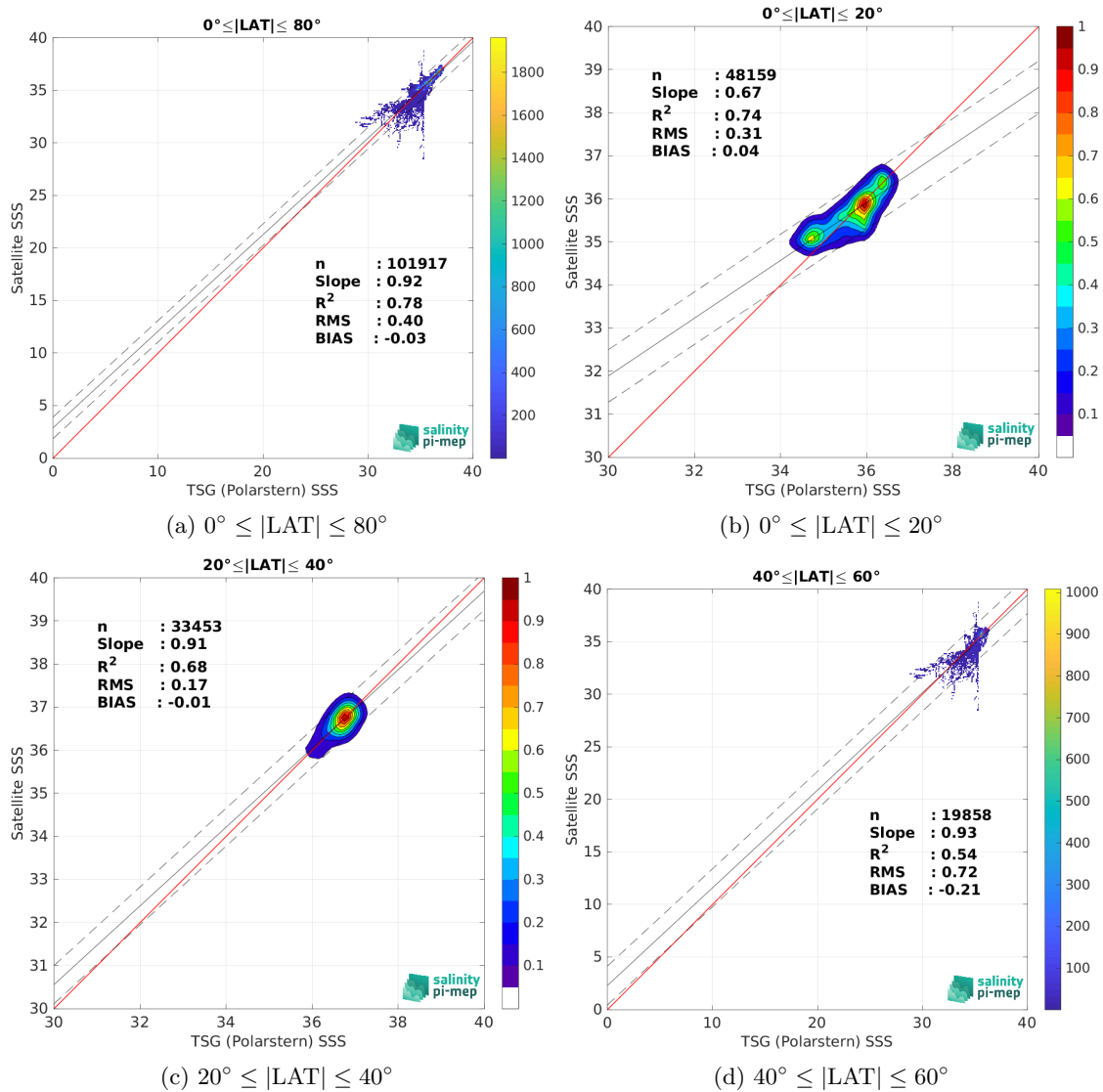
Figure 9: Contour maps of the concentration of SMOS SSS L4 v2 - Daily (BEC) SSS (y-axis) versus TSG (Polarstern) SSS (x-axis) at match-up pairs for different latitude bands. For each plot, the red line shows x=y . The black thin and dashed lines indicate a linear fit through the data cloud and the \pm 95\% confidence levels, respectively. The number match-up pairs n , the slope and R^2 coefficient of the linear fit, the root mean square (RMS) and the mean bias between satellite and in situ data are indicated for each latitude band in each plots.
