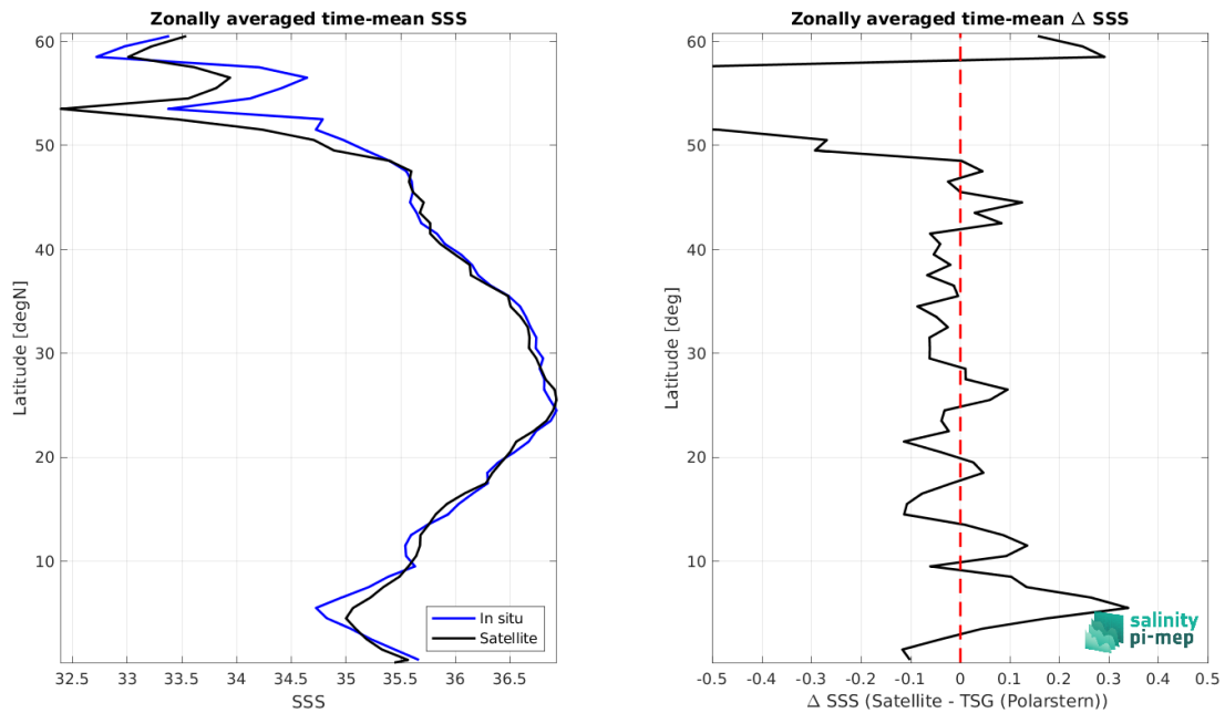
Figure 8: Left panel: Zonal mean SSS from SMOS SSS L4 v2 - Daily (BEC) satellite product (black) and from TSG (Polarstern) (blue). Right panel: Zonal mean of \Delta SSS (Satellite - TSG (Polarstern)) for all the collected Pi-MEP match-up pairs estimated over the full satellite product period.
