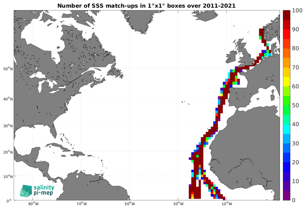
Figure 4: Number of SSS match-ups between TSG (Polarstern) SSS and the SMOS SSS L4 v2 - Daily (BEC) SSS product for the North Atlantic Ocean Pi-MEP region over 1^\circ \times 1^\circ boxes and for the full satellite product period.
