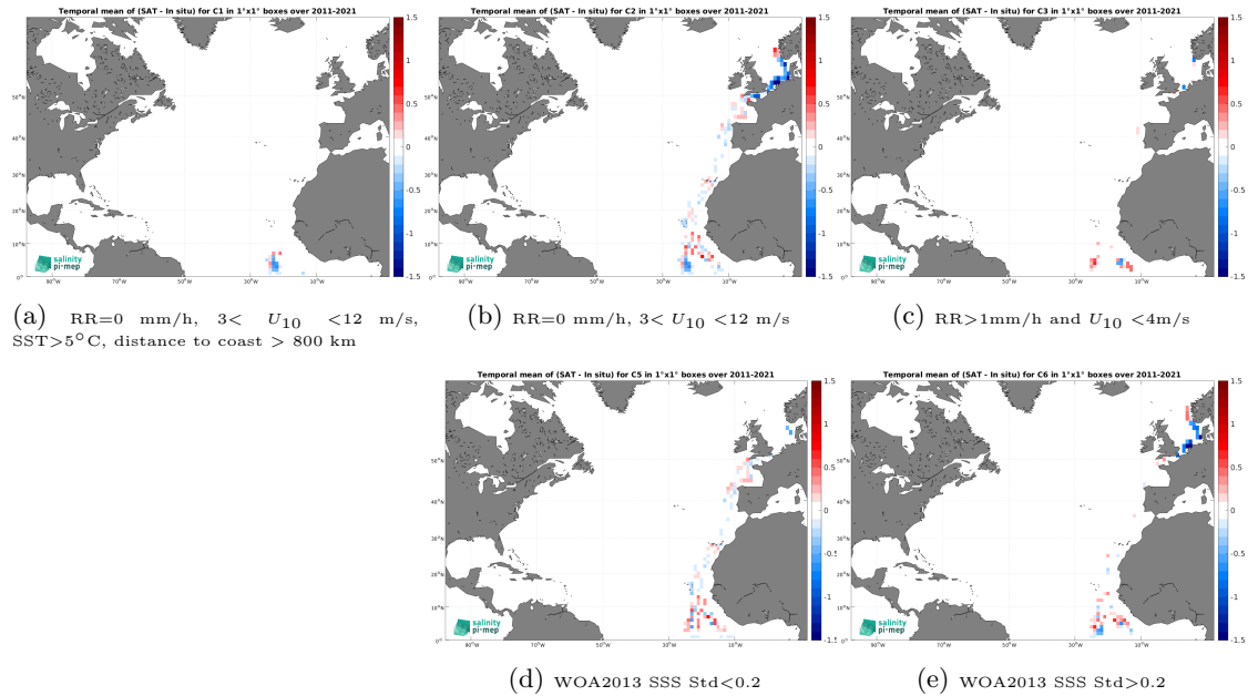
Figure 12: Temporal mean gridded over spatial boxes of size 1^\circ \times 1^\circ of \Delta\text{SSS} (SMOS SSS L4 v2 - Daily (BEC) - TSG (Polarstern)) for 5 different subdatasets corresponding to:RR=0 mm/h, 3 < U_{10} < 12 m/s, SST >5^\circ\text{C} , distance to coast > 800 km (a), RR=0 mm/h, 3 < U_{10} < 12 m/s (b), RR >1 mm/h and U_{10} < 4 m/s (c), WOA2013 SSS Std <0.2 (d), WOA2013 SSS Std >0.2 (e).
