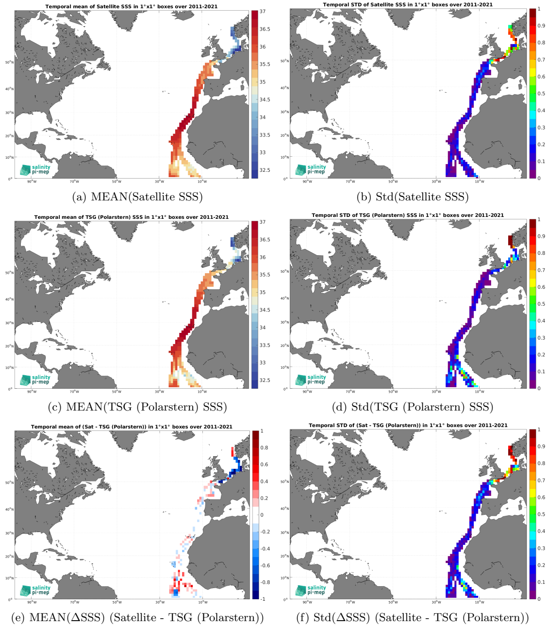
Figure 6: Temporal mean (left) and Std (right) of SSS from SMOS SSS L4 v2 - Daily (BEC) (top), TSG (Polarstern) (middle), and of \Delta SSS (Satellite - TSG (Polarstern)). Only match-up pairs are used to generate these maps.
