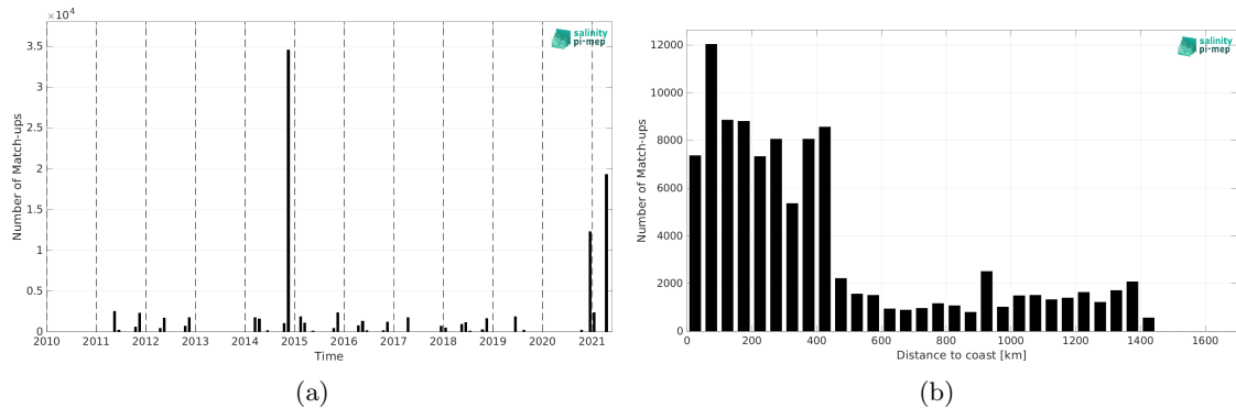
Figure 1: Number of match-ups between TSG (Polarstern) and SMOS SSS L4 v2 - Daily (BEC) SSS as a function of time (a) and as function of the distance to coast (b) over the North Atlantic Ocean Pi-MEP region and for the full satellite product period.
