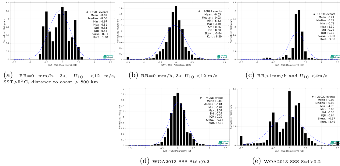
Figure 13: Normalized histogram of \Delta SSS (SMOS SSS L4 v2 - Daily (BEC) - TSG (Polarstern)) for 5 different subdatasets corresponding to: RR=0 mm/h, 3 < U_{10} < 12 m/s, SST > 5°C, distance to coast > 800 km (a), RR=0 mm/h, 3 < U_{10} < 12 m/s (b), RR > 1mm/h and U_{10} < 4 m/s (c), WOA2013 SSS Std < 0.2 (d), WOA2013 SSS Std > 0.2 (e).
