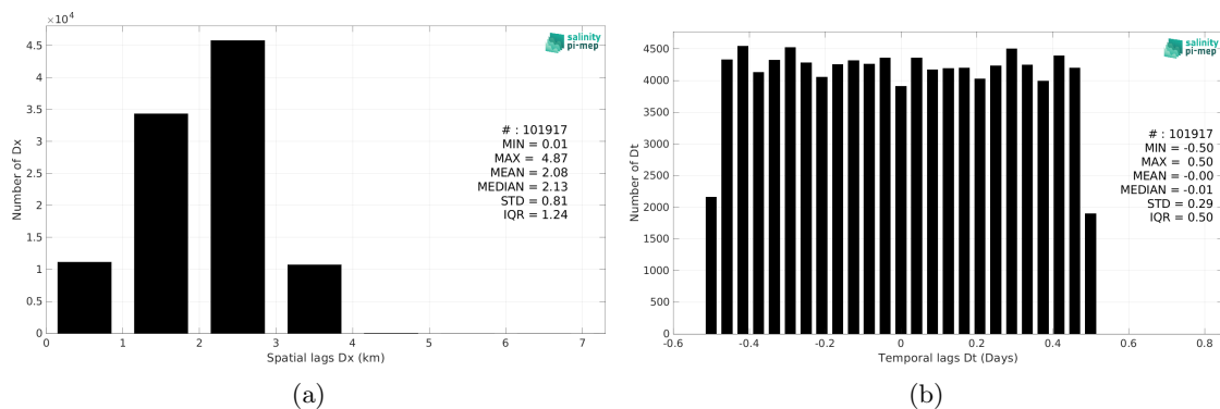
Figure 5: Histograms of the spatial (a) and temporal (b) lags between the location/time of the TSG (Polarstern) measurement and the date of the corresponding SMOS SSS L4 v2 - Daily (BEC) SSS pixel.
