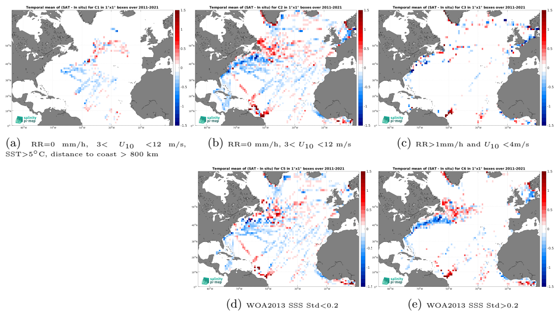
Figure 14: Temporal mean gridded over spatial boxes of size 1^\circ \times 1^\circ of \Delta\text{SSS} (SMOS SSS L4 v2 - Daily (BEC) - TSG (LEGOS-DM)) for 5 different subdatasets corresponding to:RR=0 mm/h, 3 < U_{10} < 12 m/s, SST > 5^\circ\text{C} , distance to coast > 800 km (a), RR=0 mm/h, 3 < U_{10} < 12 m/s (b), RR > 1 mm/h and U_{10} < 4 m/s (c), WOA2013 SSS Std < 0.2 (d), WOA2013 SSS Std > 0.2 (e).
