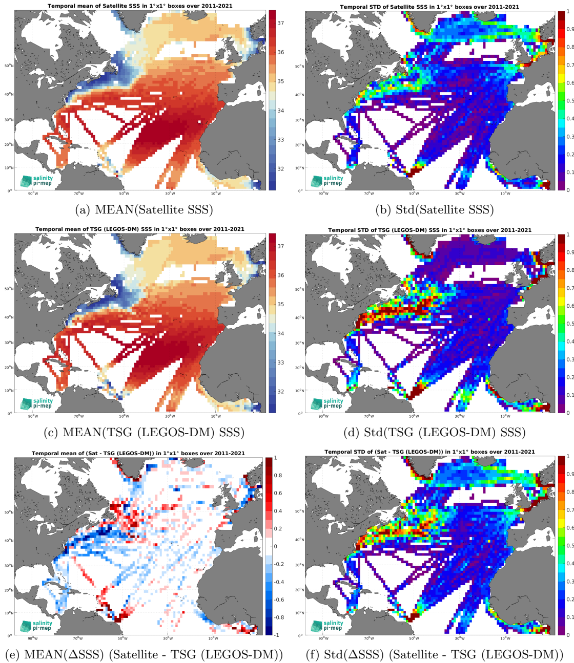
Figure 7: Temporal mean (left) and Std (right) of SSS from SMOS SSS L4 v2 - Daily (BEC) (top), TSG (LEGOS-DM) (middle), and of \Delta SSS (Satellite - TSG (LEGOS-DM)). Only match-up pairs are used to generate these maps.
