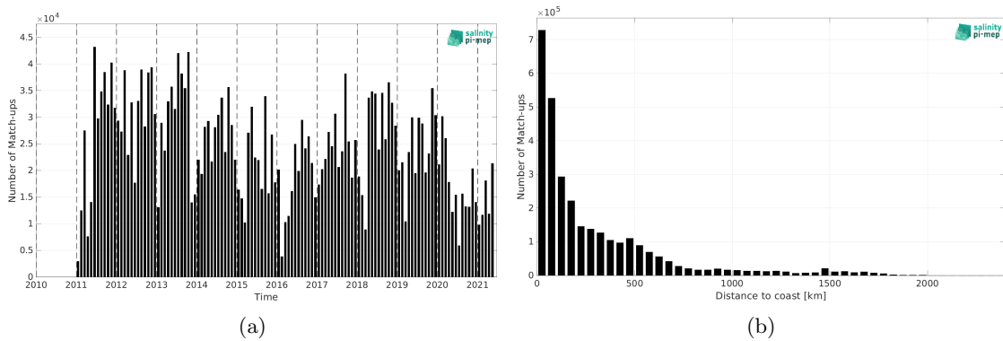
Figure 2: Number of match-ups between TSG (LEGOS-DM) and SMOS SSS L4 v2 - Daily (BEC) SSS as a function of time (a) and as function of the distance to coast (b) over the North Atlantic Ocean Pi-MEP region and for the full satellite product period.
