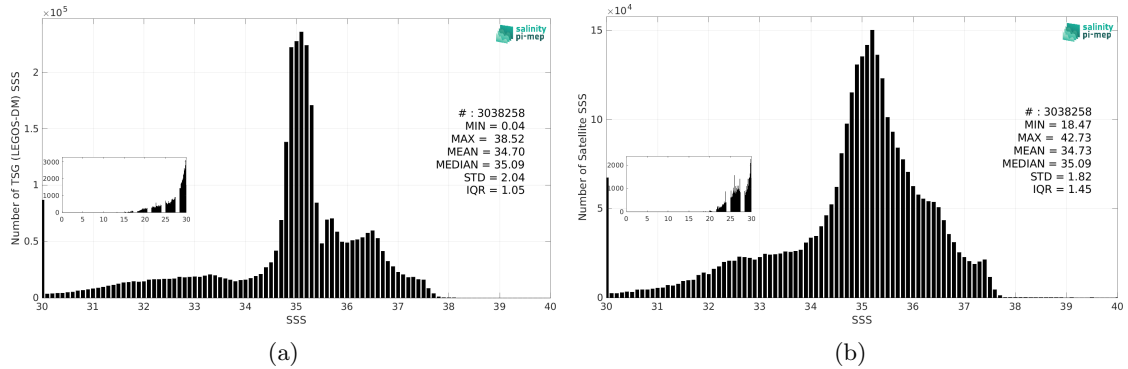
Figure 3: Histograms of SSS from TSG (LEGOS-DM) (a) and SMOS SSS L4 v2 - Daily (BEC) (b) considering all match-up pairs per bins of 0.1 over the North Atlantic Ocean Pi-MEP region and for the full satellite product period.
