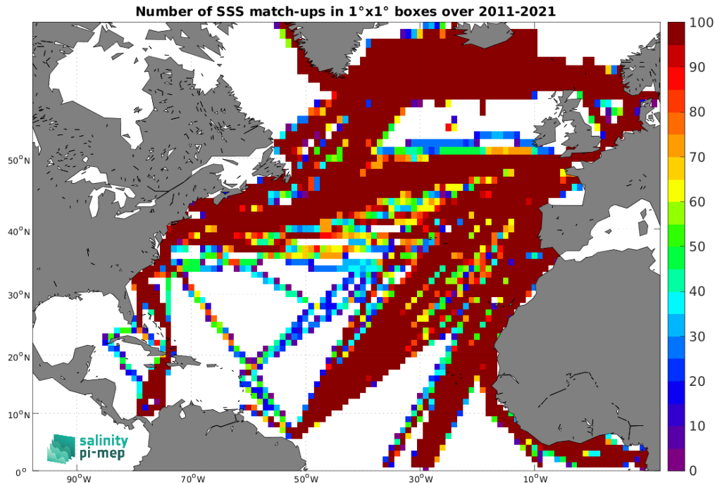
Figure 5: Number of SSS match-ups between TSG (LEGOS-DM) SSS and the SMOS SSS L4 v2 - Daily (BEC) SSS product for the North Atlantic Ocean Pi-MEP region over 1^\circ \times 1^\circ boxes and for the full satellite product period.
