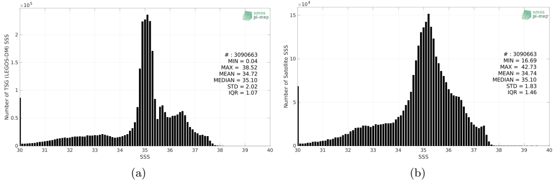
Figure 2: Histograms of SSS from TSG (LEGOS-DM) (a) and SMOS SSS L4 v2 - Daily (BEC) (b) considering all match-up pairs per bins of 0.1 over the North Atlantic Ocean Pi-MEP region and for the full satellite product period.
