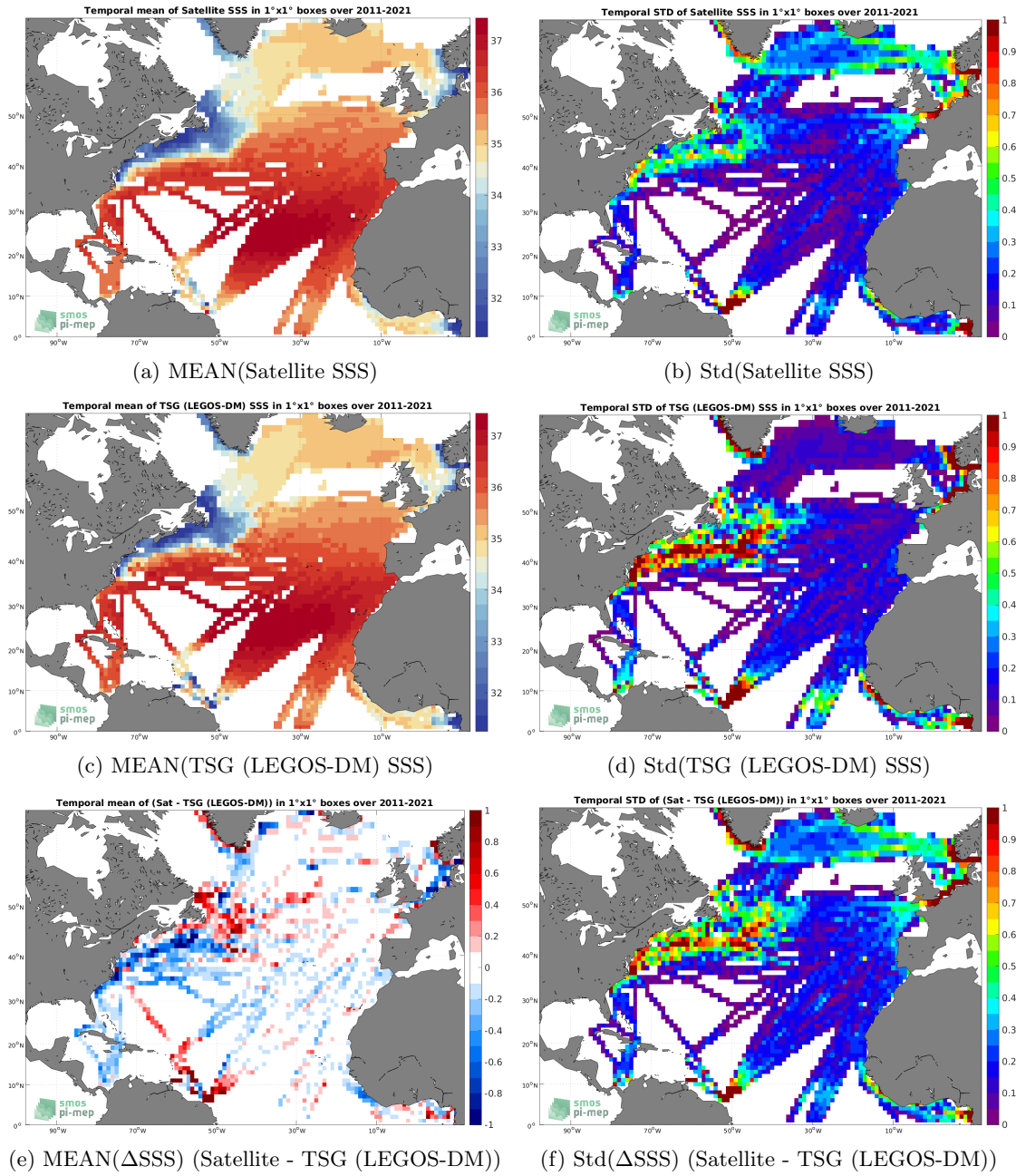
Figure 6: Temporal mean (left) and Std (right) of SSS from SMOS SSS L4 v2 - Daily (BEC) (top), TSG (LEGOS-DM) (middle), and of \Delta SSS (Satellite - TSG (LEGOS-DM)). Only match-up pairs are used to generate these maps.
