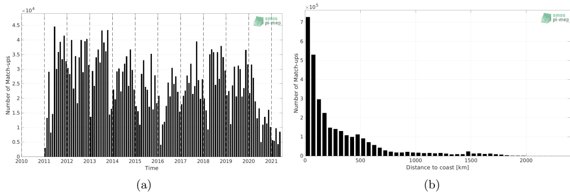
Figure 1: Number of match-ups between TSG (LEGOS-DM) and SMOS SSS L4 v2 - Daily (BEC) SSS as a function of time (a) and as function of the distance to coast (b) over the North Atlantic Ocean Pi-MEP region and for the full satellite product period.
