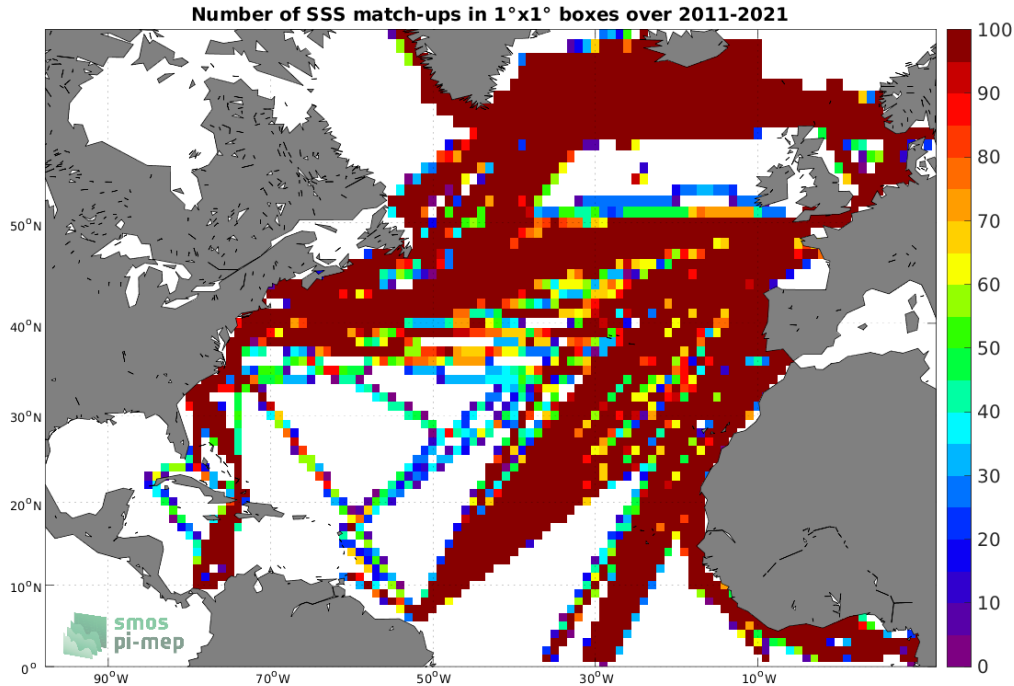
Figure 4: Number of SSS match-ups between TSG (LEGOS-DM) SSS and the SMOS SSS L4 v2 - Daily (BEC) SSS product for the North Atlantic Ocean Pi-MEP region over 1^\circ \times 1^\circ boxes and for the full satellite product period.
