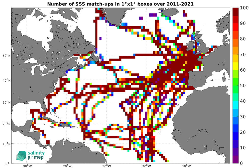
Figure 5: Number of SSS match-ups between TSG (GOSUD-Sailing-ship) SSS and the SMOS SSS L4 v2 - Daily (BEC) SSS product for the North Atlantic Ocean Pi-MEP region over 1^\circ \times 1^\circ boxes and for the full satellite product period.
