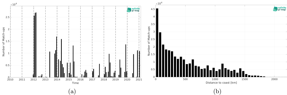
Figure 2: Number of match-ups between TSG (GOSUD-Sailing-ship) and SMOS SSS L4 v2 - Daily (BEC) SSS as a function of time (a) and as function of the distance to coast (b) over the North Atlantic Ocean Pi-MEP region and for the full satellite product period.
