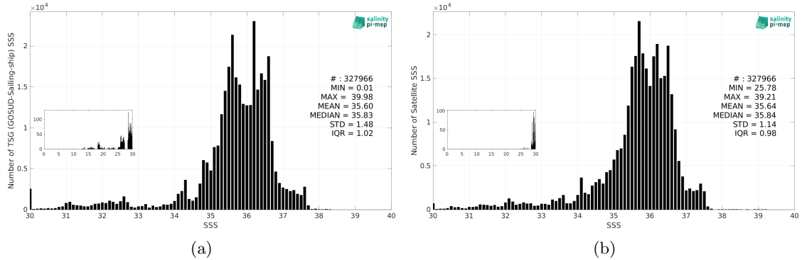
Figure 3: Histograms of SSS from TSG (GOSUD-Sailing-ship) (a) and SMOS SSS L4 v2 - Daily (BEC) (b) considering all match-up pairs per bins of 0.1 over the North Atlantic Ocean Pi-MEP region and for the full satellite product period.
