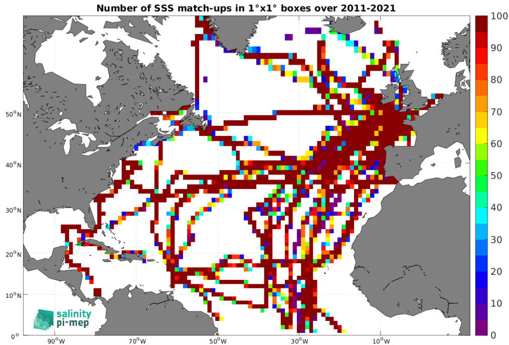
Figure 4: Number of SSS match-ups between TSG (GOSUD-Sailing-ship) SSS and the SMOS SSS L4 v2 - Daily (BEC) SSS product for the North Atlantic Ocean Pi-MEP region over 1^\circ \times 1^\circ boxes and for the full satellite product period.
