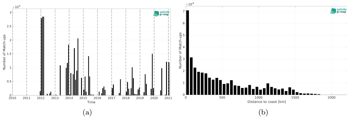
Figure 1: Number of match-ups between TSG (GOSUD-Sailing-ship) and SMOS SSS L4 v2 - Daily (BEC) SSS as a function of time (a) and as function of the distance to coast (b) over the North Atlantic Ocean Pi-MEP region and for the full satellite product period.
