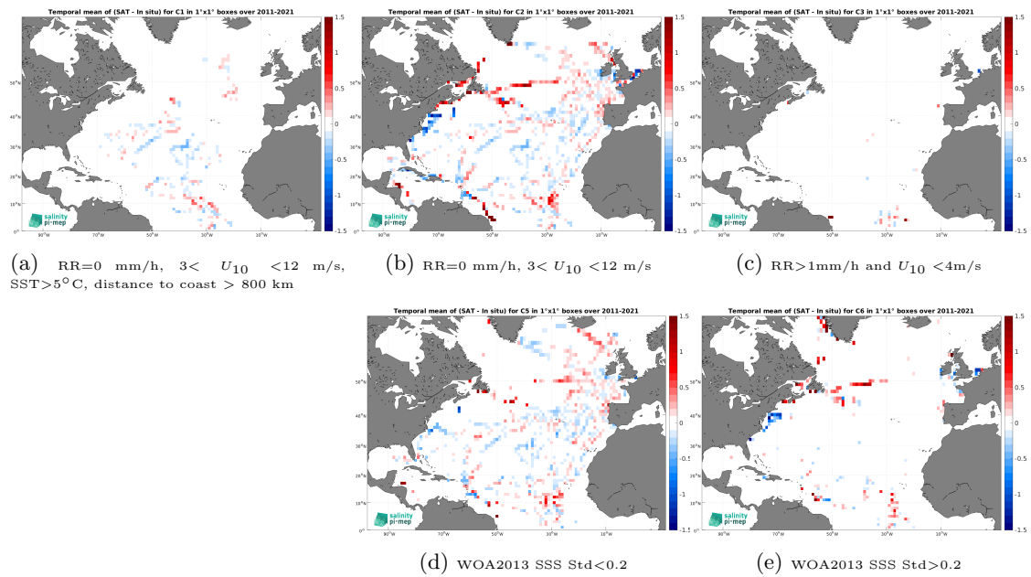
Figure 12: Temporal mean gridded over spatial boxes of size 1^\circ \times 1^\circ of \Delta\text{SSS} (SMOS SSS L4 v2 - Daily (BEC) - TSG (GOSUD-Sailing-ship)) for 5 different subdatasets corresponding to:RR=0 mm/h, 3 < U_{10} < 12 m/s, SST >5^\circ\text{C} , distance to coast > 800 km (a), RR=0 mm/h, 3 < U_{10} < 12 m/s (b), RR >1 mm/h and U_{10} < 4 m/s (c), WOA2013 SSS Std <0.2 (d), WOA2013 SSS Std >0.2 (e).
