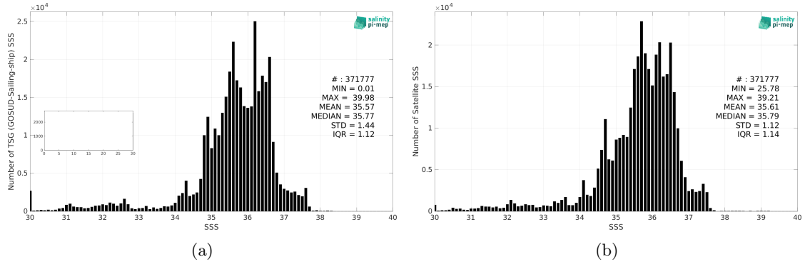
Figure 2: Histograms of SSS from TSG (GOSUD-Sailing-ship) (a) and SMOS SSS L4 v2 - Daily (BEC) (b) considering all match-up pairs per bins of 0.1 over the North Atlantic Ocean Pi-MEP region and for the full satellite product period.
