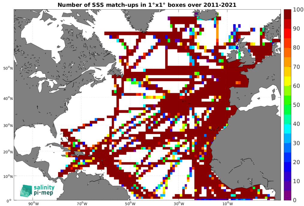
Figure 5: Number of SSS match-ups between TSG (GOSUD-Research-vessel) SSS and the SMOS SSS L4 v2 - Daily (BEC) SSS product for the North Atlantic Ocean Pi-MEP region over 1^\circ \times 1^\circ boxes and for the full satellite product period.
