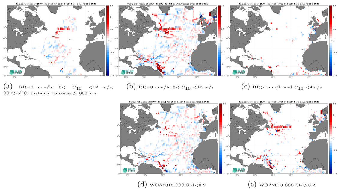
Figure 14: Temporal mean gridded over spatial boxes of size 1^\circ \times 1^\circ of \Delta\text{SSS} (SMOS SSS L4 v2 - Daily (BEC) - TSG (GOSUD-Research-vessel)) for 5 different subdatasets corresponding to:RR=0 mm/h, 3 < U_{10} < 12 m/s, SST>5°C, distance to coast > 800 km (a), RR=0 mm/h, 3 < U_{10} < 12 m/s (b), RR>1mm/h and U_{10} < 4 m/s (c), WOA2013 SSS Std<0.2 (d), WOA2013 SSS Std>0.2 (e).
