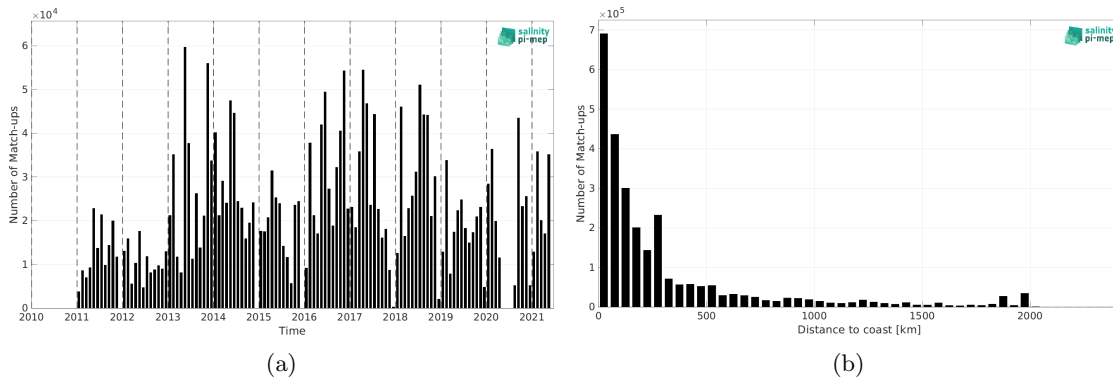
Figure 2: Number of match-ups between TSG (GOSUD-Research-vessel) and SMOS SSS L4 v2 - Daily (BEC) SSS as a function of time (a) and as function of the distance to coast (b) over the North Atlantic Ocean Pi-MEP region and for the full satellite product period.
