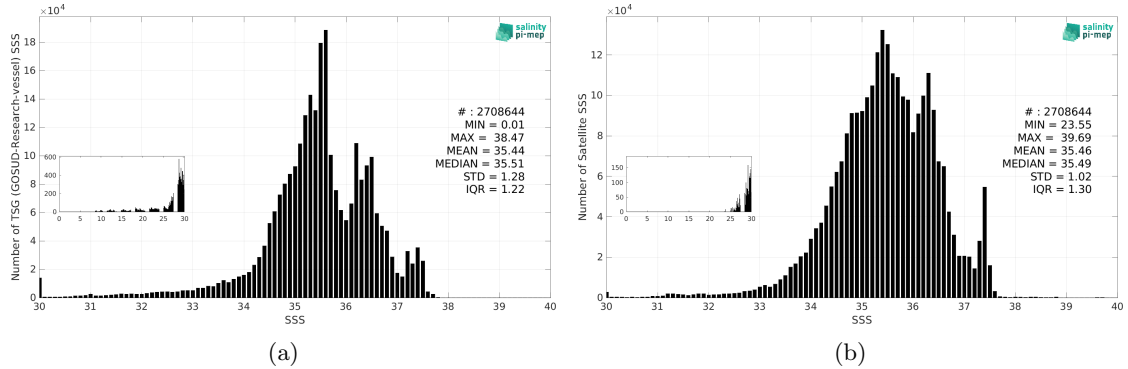
Figure 3: Histograms of SSS from TSG (GOSUD-Research-vessel) (a) and SMOS SSS L4 v2 - Daily (BEC) (b) considering all match-up pairs per bins of 0.1 over the North Atlantic Ocean Pi-MEP region and for the full satellite product period.
