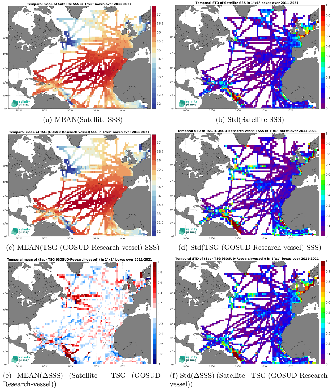
Figure 7: Temporal mean (left) and Std (right) of SSS from SMOS SSS L4 v2 - Daily (BEC) (top), TSG (GOSUD-Research-vessel) (middle), and of \Delta SSS (Satellite - TSG (GOSUD-Research-vessel)). Only match-up pairs are used to generate these maps.
